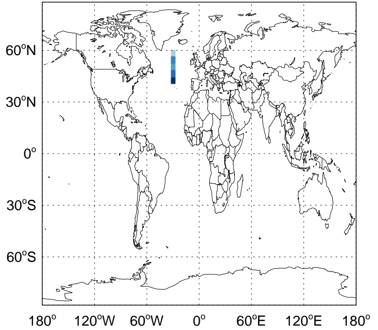
NH3 anthro emissions for Jul
