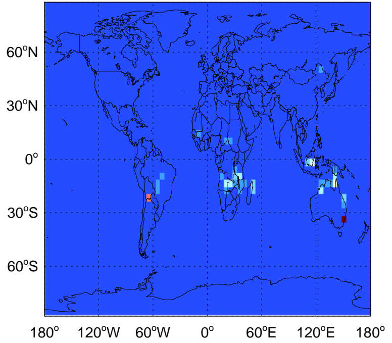
C3H8 biomass emissions for Oct
