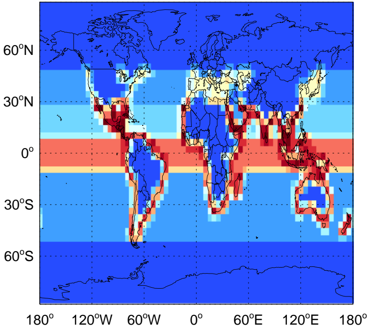
CHBr3 biogenic emissions for Jan
