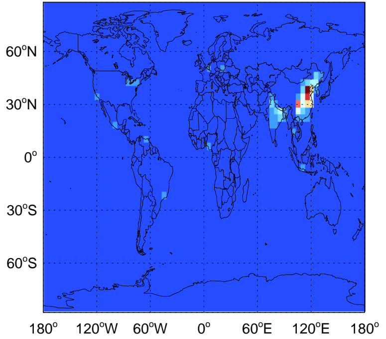
CO anthro+biofuel emissions for Jan
