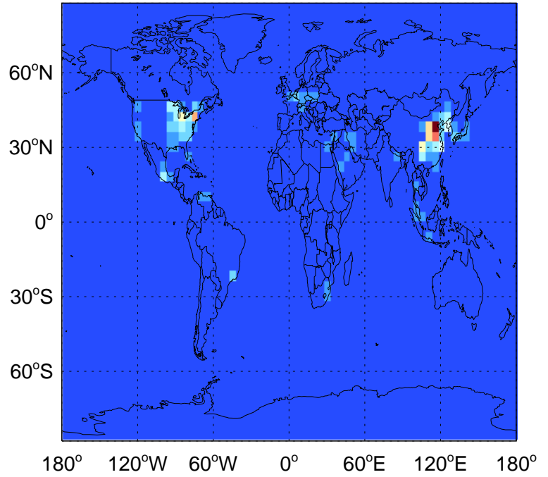
OC anthro emissions for Jan
