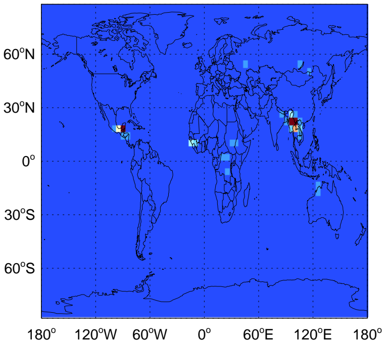
PRPE biomass emissions for Apr
