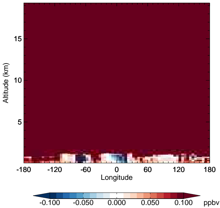
v11-01-public-Run0 - v11-01g-Run0 N2O - Diff along 15S for Jan
