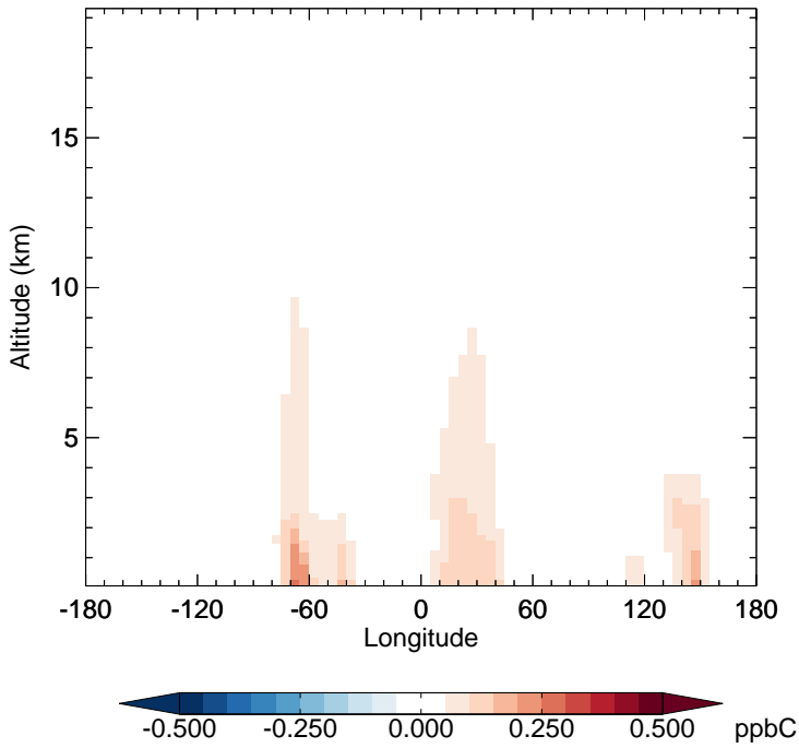
v11-01-public-Run0 - v11-01g-Run0 C3H8 - Diff along 15S for Jan
