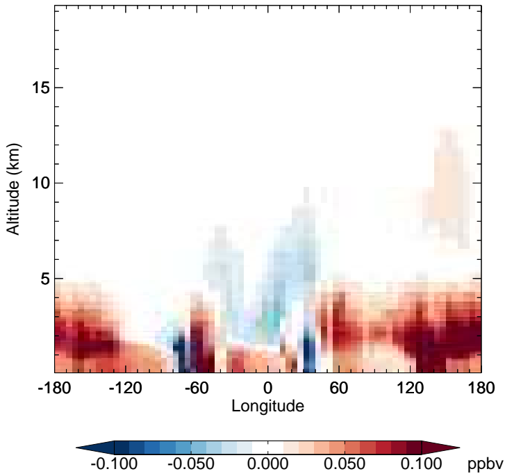
v11-01-public-Run0 - v11-01g-Run0 H2O2 - Diff along 15S for Jan
