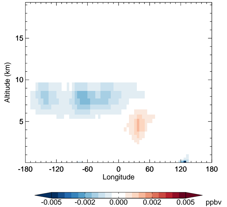
v11-01-public-Run0 - v11-01g-Run0 HNO 4 - Diff along 42N for Jan
