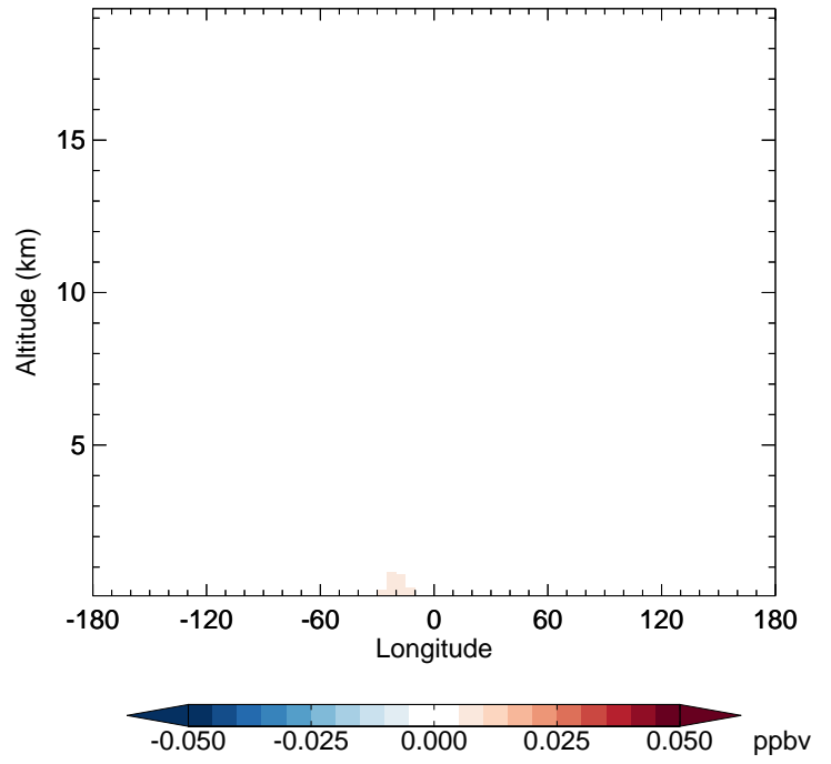
v11-01-public-Run0 - v11-01k-Run0 MP - Diff along 42N for Jan
