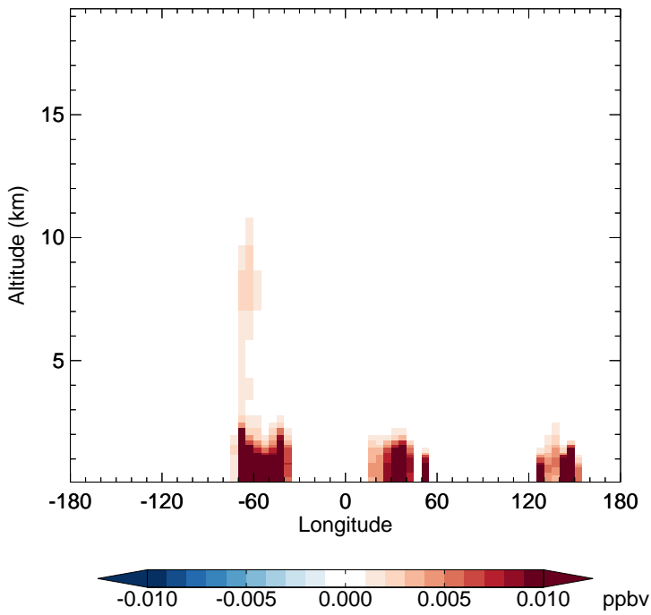
v11-01-public-Run0 - v11-01g-Run0 RIP - Diff along 15S for Jan
