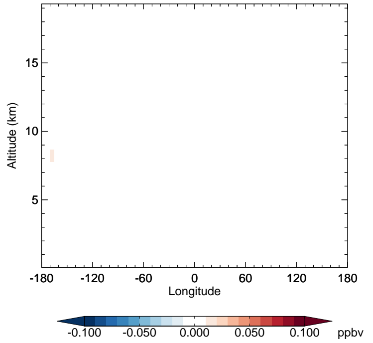
v11-01-public-Run0 - v11-01k-Run0 H2O - Diff along 42N for Jan
