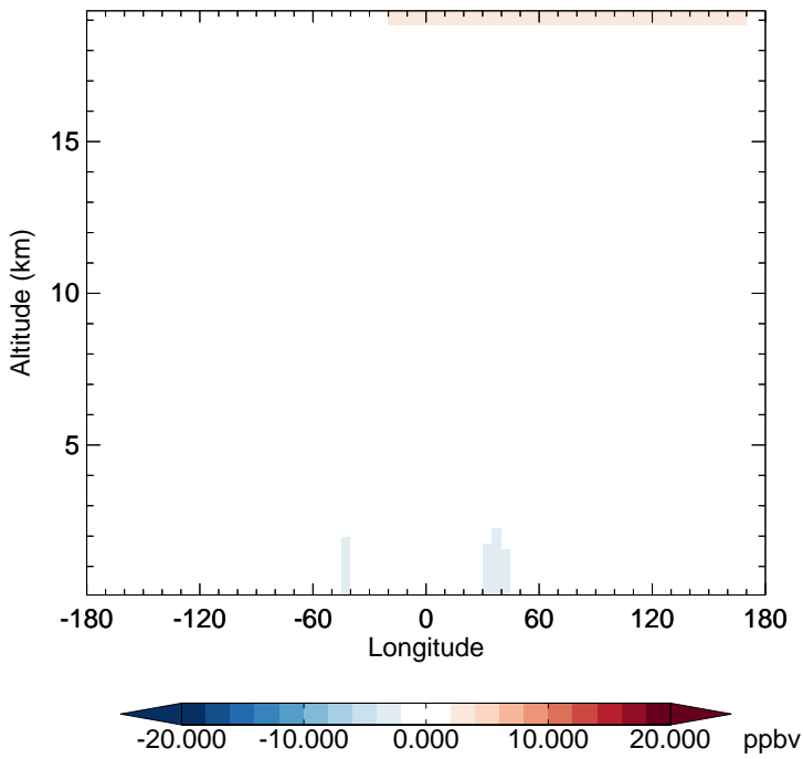
v11-01-public-Run0 - v11-01g-Run0 O3 - Diff along 15S for Jan
