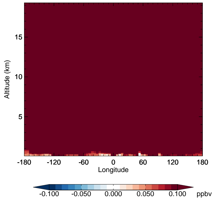
v11-01-public-Run0 - v11-01g-Run0 N2O - Diff along 42N for Jan
