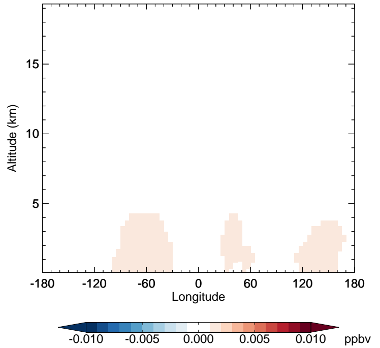
v11-01-public-Run0 - v11-01g-Run0 R4N2 - Diff along 42N for Jan
