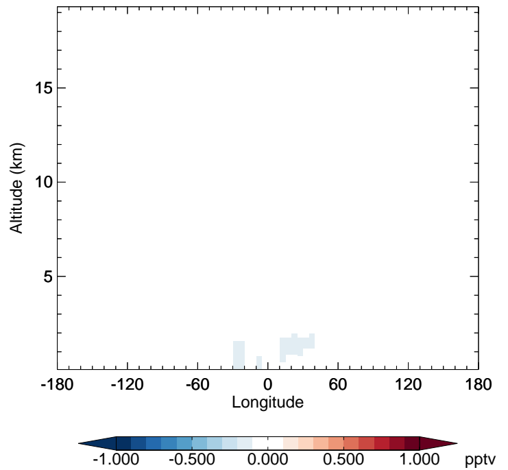
v11-01-public-Run0 - v11-01g-Run0 HO2 - Diff along 42N for Jan
