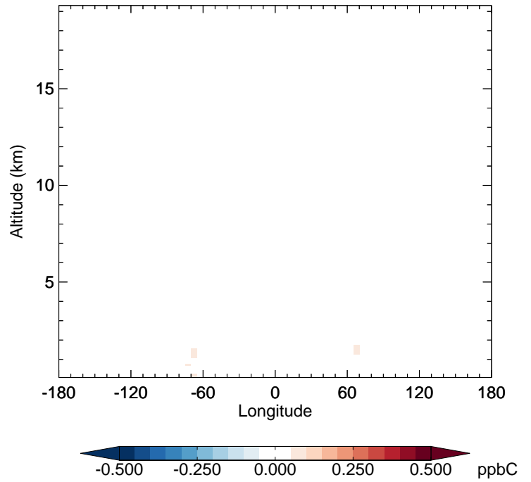
v11-01-public-Run0 - v11-01g-Run0 ALK4 - Diff along 42N for Jan
