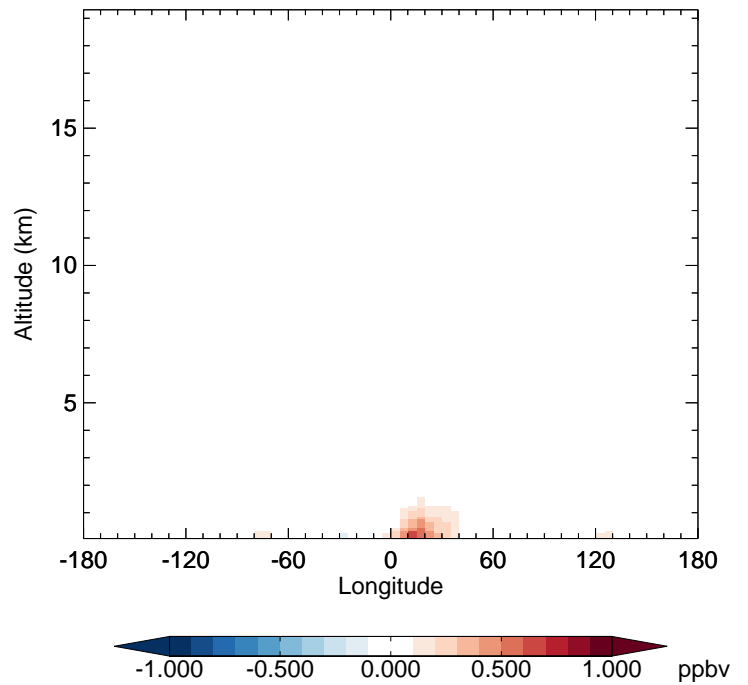
v11-01-public-Run0 - v11-01g-Run0 NO 2 - Diff along 42N for Jan
