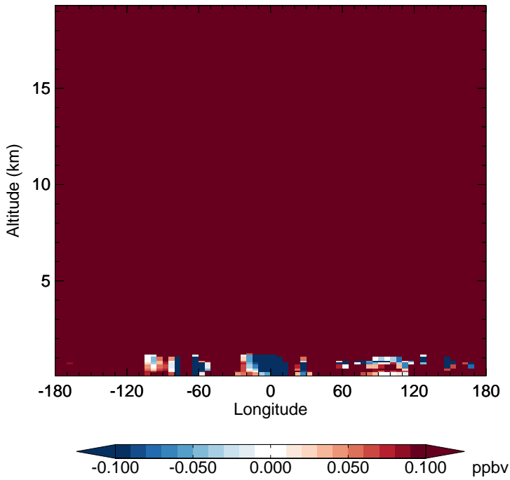
v11-01-public-Run0 - v11-01g-Run0 CH4 - Diff along 15S for Jan
