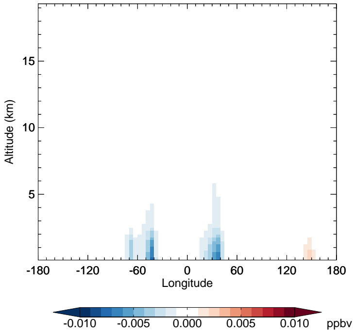
v11-01-public-Run0 - v11-01g-Run0 R4N2 - Diff along 15S for Jan
