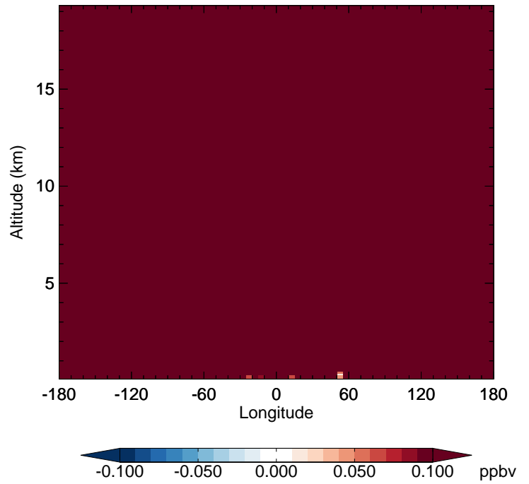
v11-01-public-Run0 - v11-01g-Run0 CH4 - Diff along 42N for Jan
