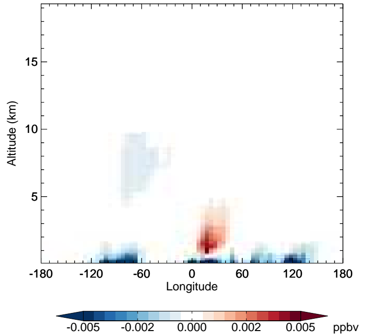
v11-01-public-Run0 - v11-01g-Run0 N2O5 - Diff along 42N for Jan
