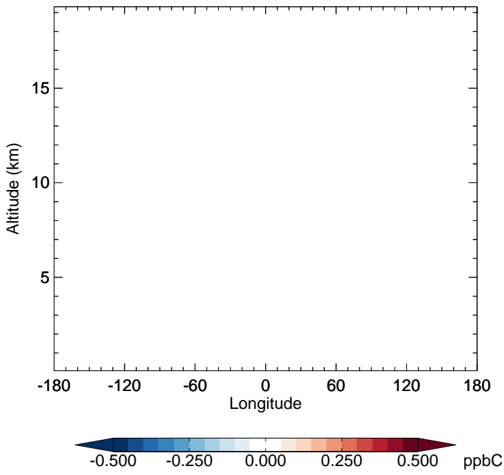
v11-01-public-Run0 - v11-01k-Run0 ISOP - Diff along 15S for Jan
