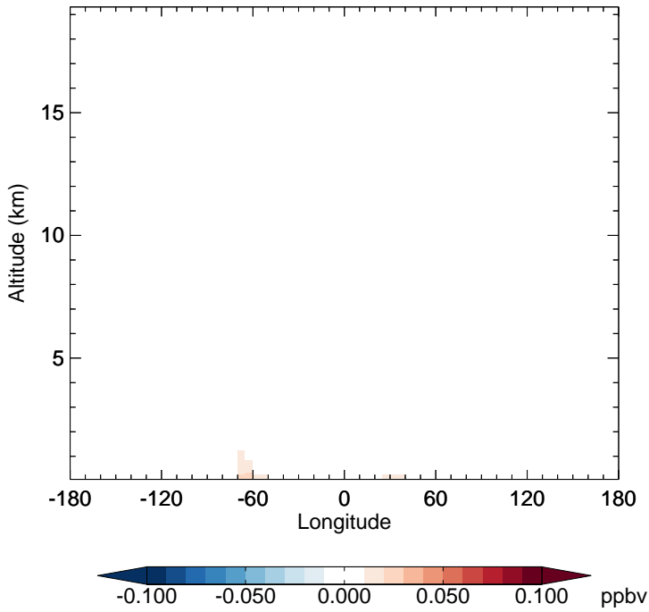
v11-01-public-Run0 - v11-01g-Run0 MTPA - Diff along 15S for Jan
