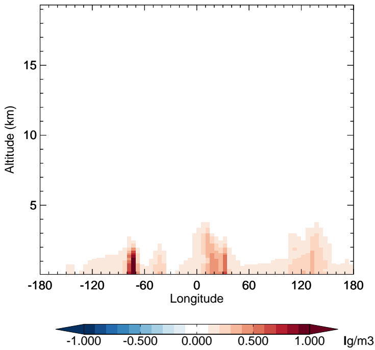
v11-01-public-Run0 - v11-01g-Run0 SO4 - Diff along 15S for Jan
