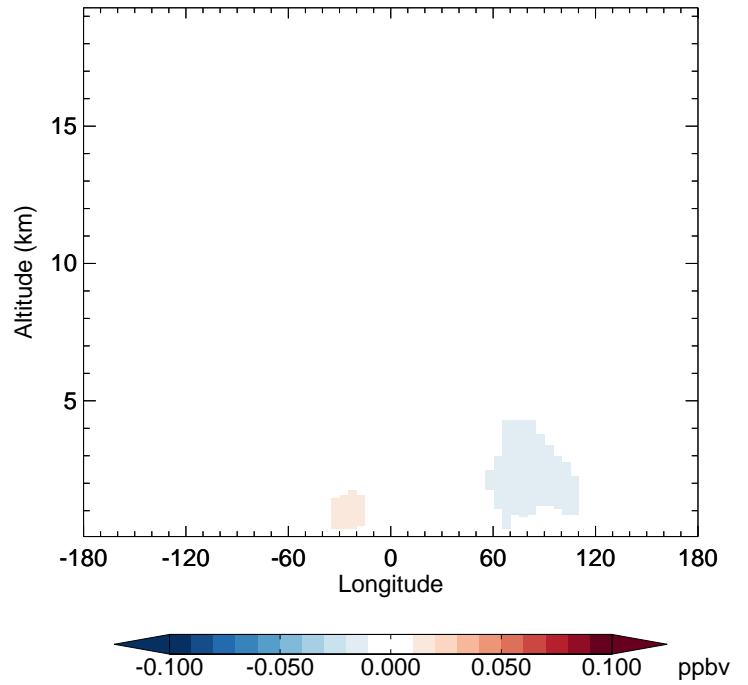
v11-01-public-Run0 - v11-01g-Run0 H2O2 - Diff along 42N for Jan
