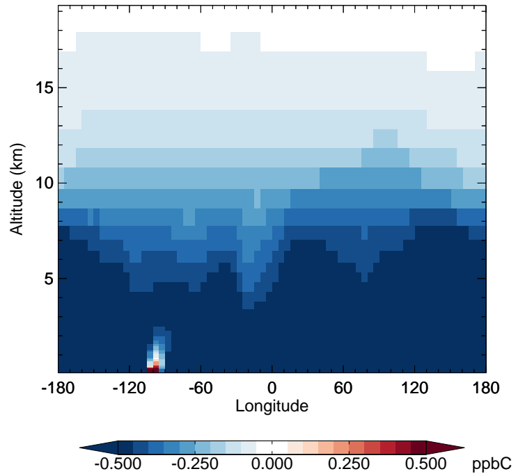
v11-01-public-Run0 - v11-01g-Run0 C2H6 - Diff along 42N for Jan
