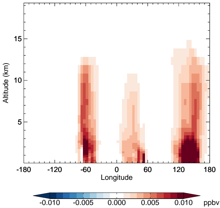
v11-01-public-Run0 - v11-01g-Run0 MAP - Diff along 15S for Jan
