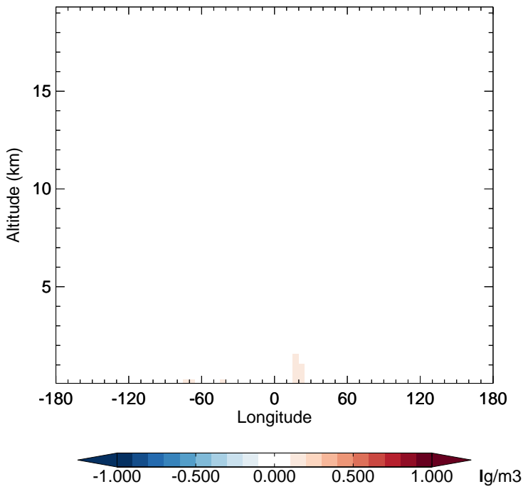
v11-01-public-Run0 - v11-01g-Run0 NH4 - Diff along 15S for Jan
