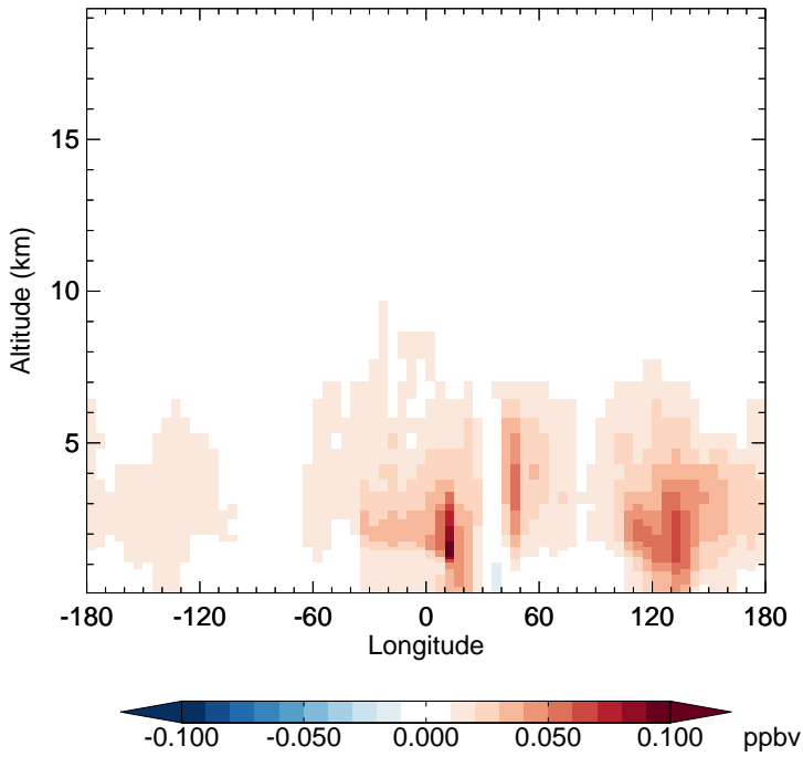
v11-01-public-Run0 - v11-01g-Run0 HNO 3 - Diff along 15S for Jan
