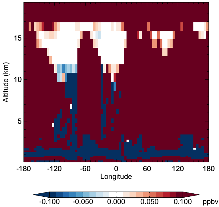
v11-01-public-Run0 - v11-01g-Run0 H2O - Diff along 15S for Jan
