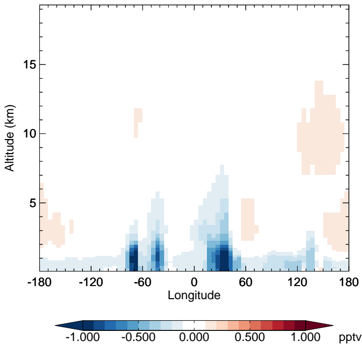
v11-01-public-Run0 - v11-01g-Run0 HO2 - Diff along 15S for Jan
