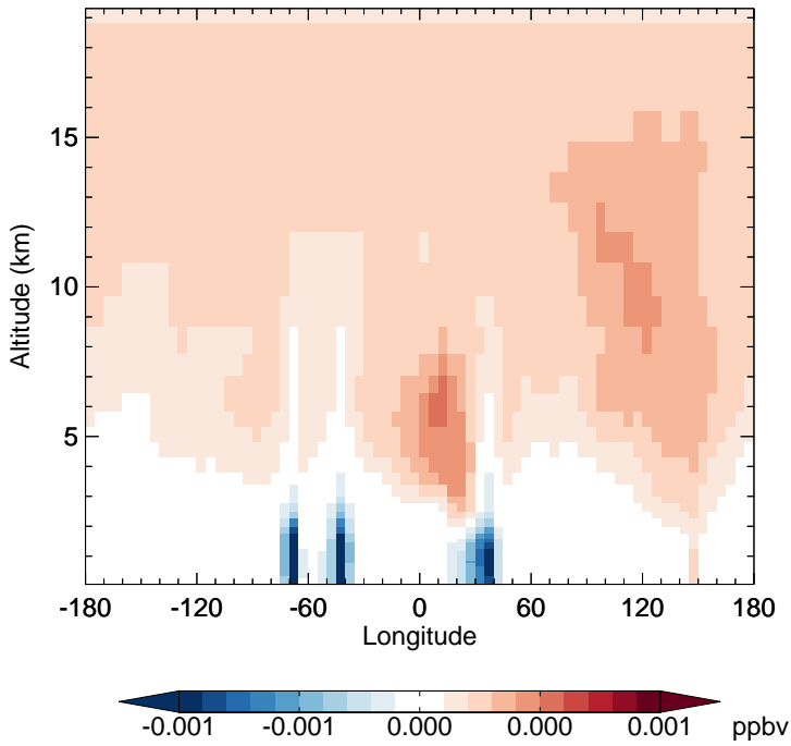
v11-01-public-Run0 - v11-01g-Run0 PPN - Diff along 15S for Jan
