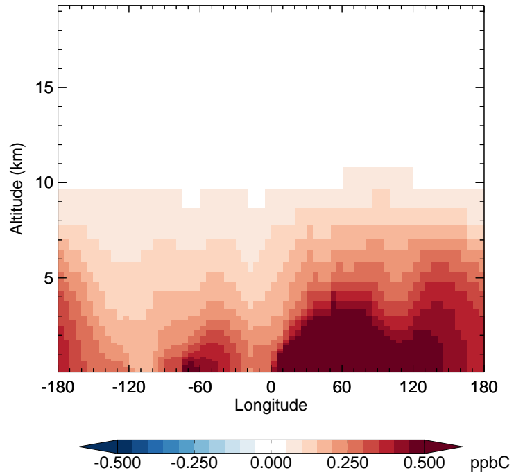
v11-01-public-Run0 - v11-01g-Run0 C3H8 - Diff along 42N for Jan
