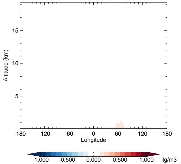
v11-01-public-Run0 - v11-01g-Run0 NH4 - Diff along 42N for Jan
