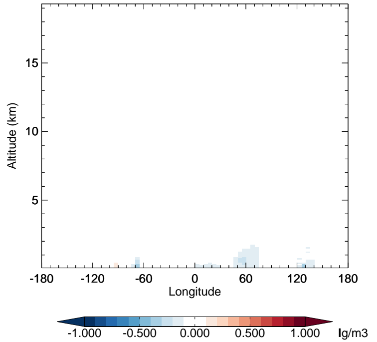
v11-01-public-Run0 - v11-01g-Run0 NIT - Diff along 42N for Jan
