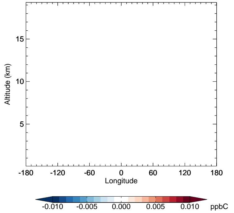
v11-01-public-Run0 - v11-01k-Run0 PRPE - Diff along 42N for Jan
