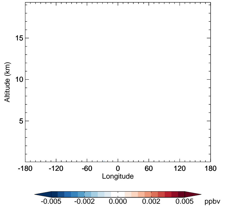
v11-01-public-Run0 - v11-01k-Run0 N2O5 - Diff along 42N for Jan
