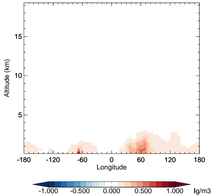
v11-01-public-Run0 - v11-01g-Run0 SO4 - Diff along 42N for Jan
