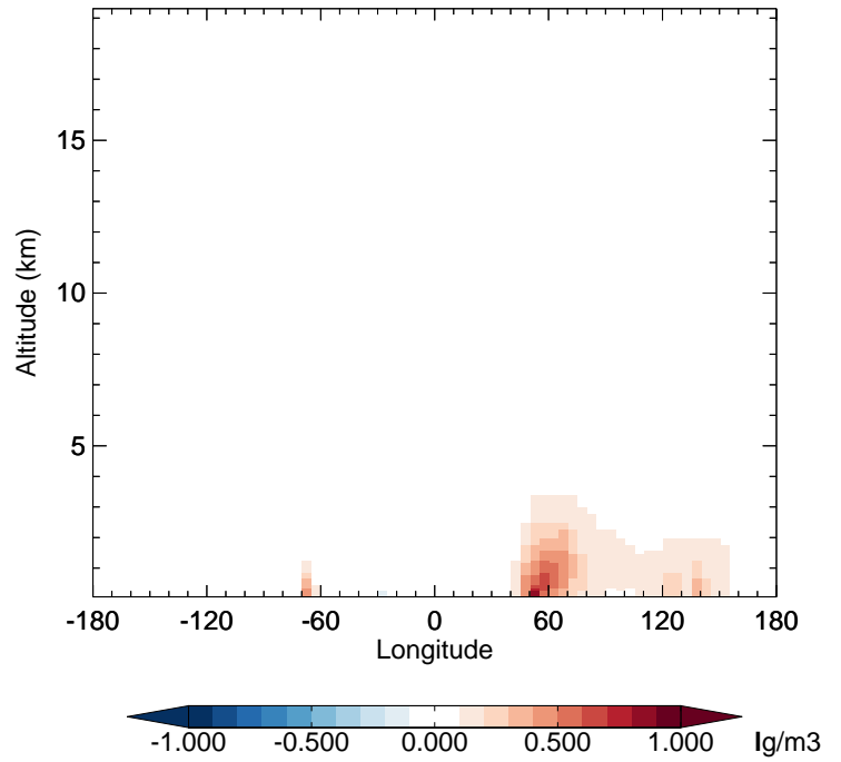
v11-01-public-Run0 - v11-01g-Run0 SO 2 - Diff along 42N for Jan
