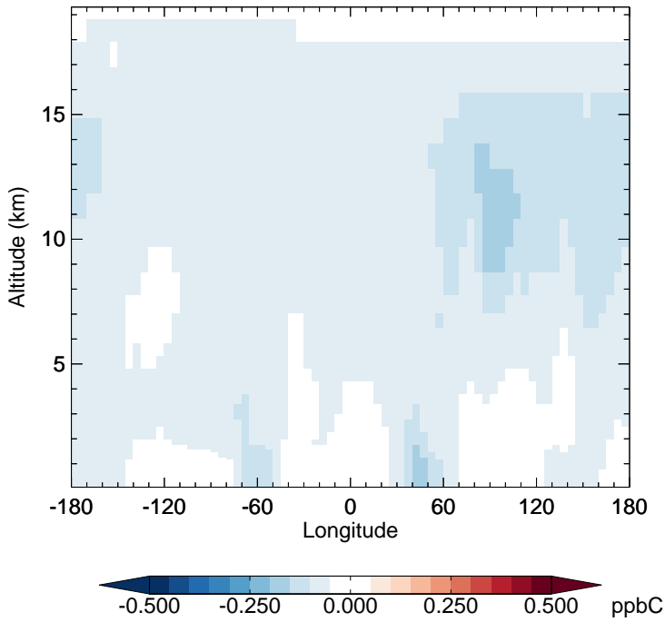
v11-01-public-Run0 - v11-01g-Run0 C2H6 - Diff along 15S for Jan
