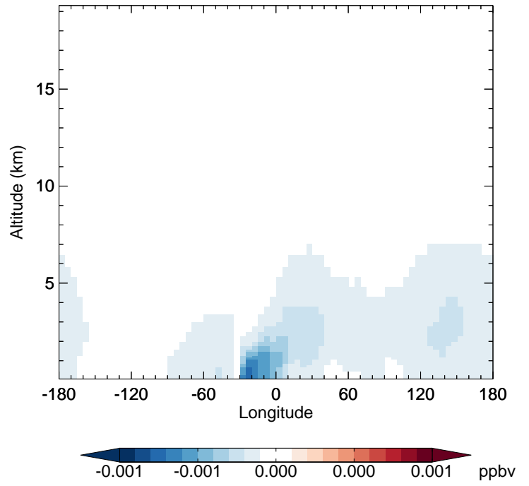
v11-01-public-Run0 - v11-01k-Run0 PPN - Diff along 42N for Jan
