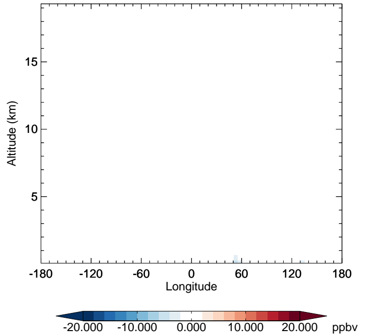
v11-01-public-Run0 - v11-01g-Run0 CO - Diff along 42N for Jan
