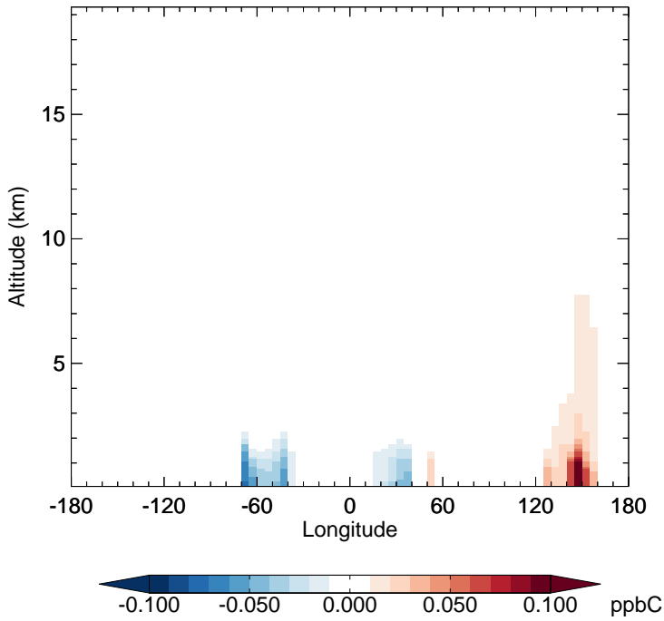
v11-01-public-Run0 - v11-01g-Run0 MEK - Diff along 15S for Jan
