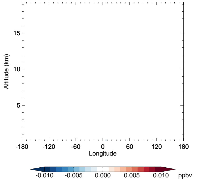
v11-01-public-Run0 - v11-01g-Run0 NO3 - Diff along 42N for Jan
