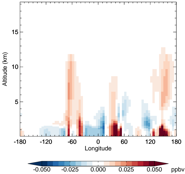
v11-01-public-Run0 - v11-01g-Run0 MP - Diff along 15S for Jan
