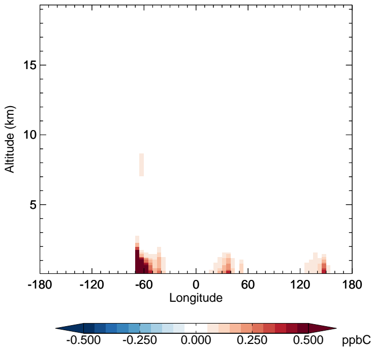
v11-01-public-Run0 - v11-01g-Run0 ISOP - Diff along 15S for Jan
