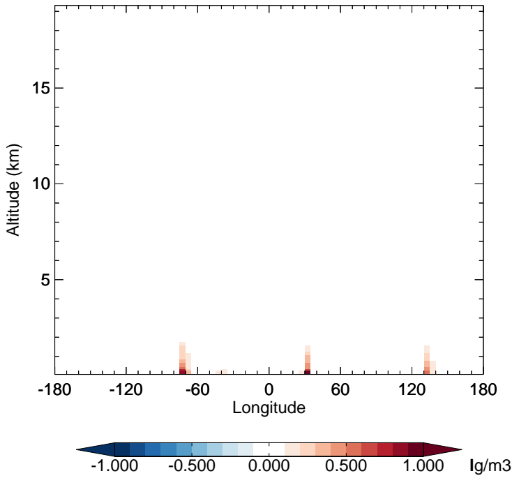
v11-01-public-Run0 - v11-01g-Run0 SO 2 - Diff along 15S for Jan
