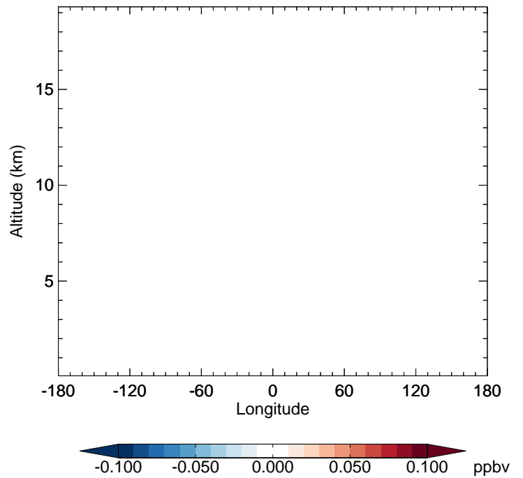
v11-01-public-Run0 - v11-01g-Run0 H1301 - Diff along 42N for Jan
