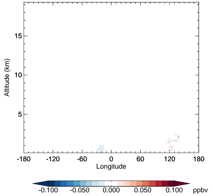
v11-01-public-Run0 - v11-01k-Run0 HNO 3 - Diff along 42N for Jan
