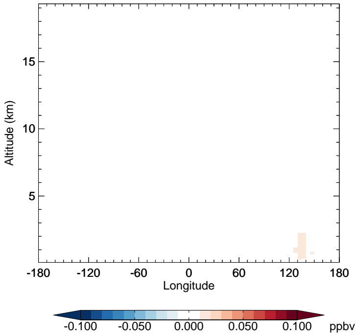
v11-01-public-Run0 - v11-01g-Run0 TSOG2 - Diff along 15S for Jan
