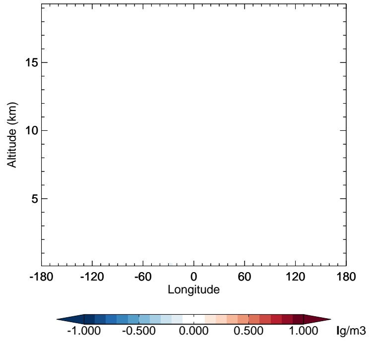
v11-01-public-Run0 - v11-01k-Run0 SO 2 - Diff along 42N for Jan
