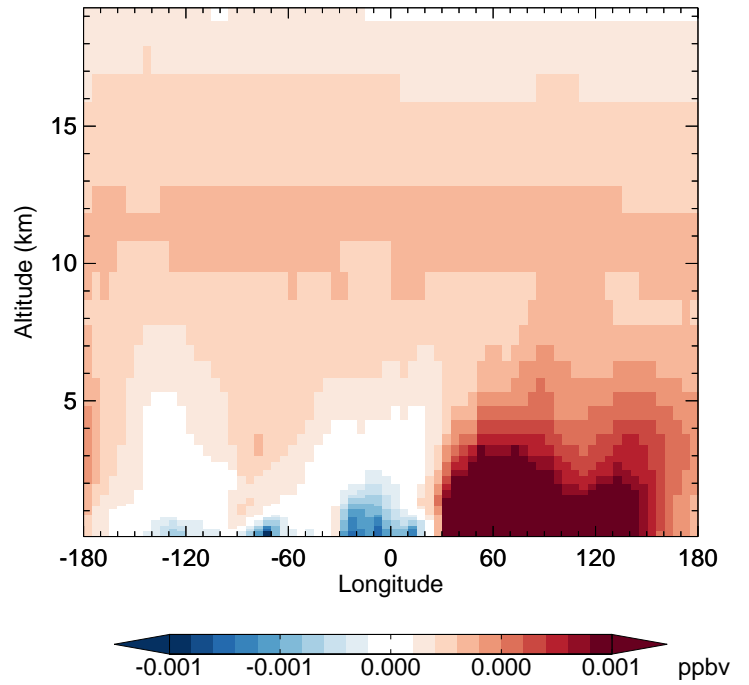
v11-01-public-Run0 - v11-01g-Run0 PPN - Diff along 42N for Jan
