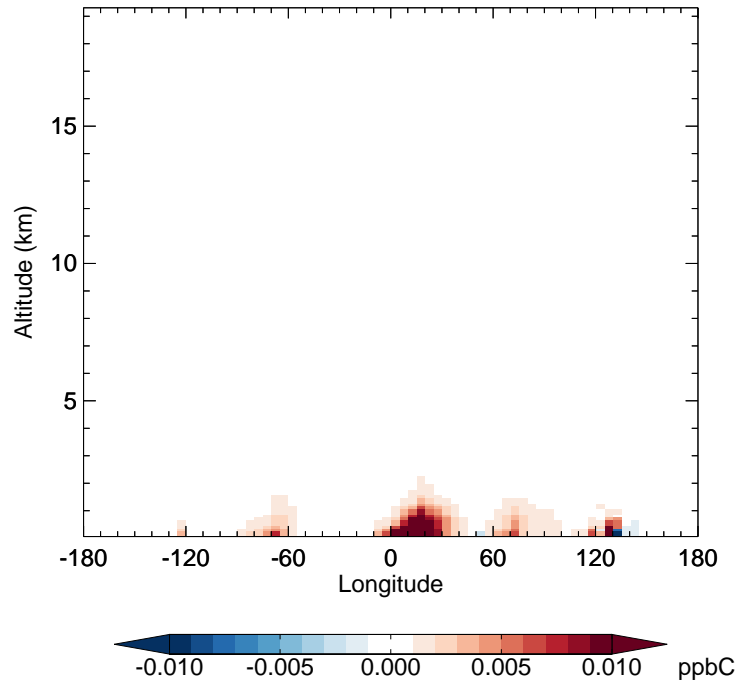
v11-01-public-Run0 - v11-01g-Run0 PRPE - Diff along 42N for Jan
