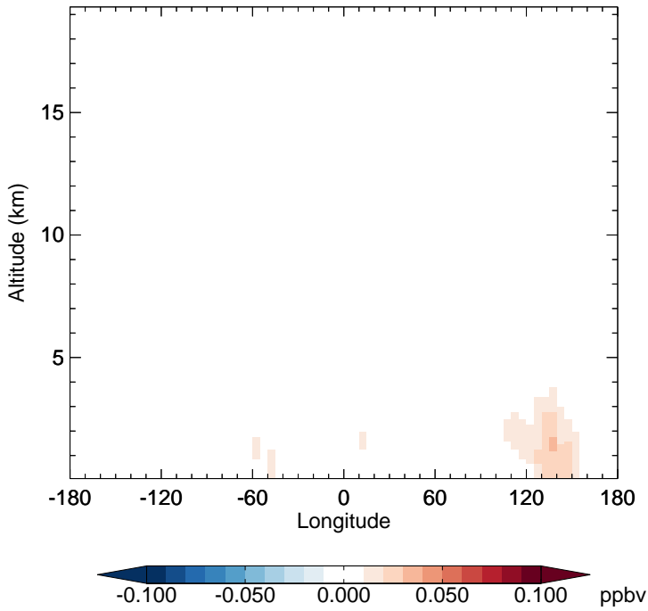
v11-01-public-Run0 - v11-01g-Run0 ISOG3 - Diff along 15S for Jan
