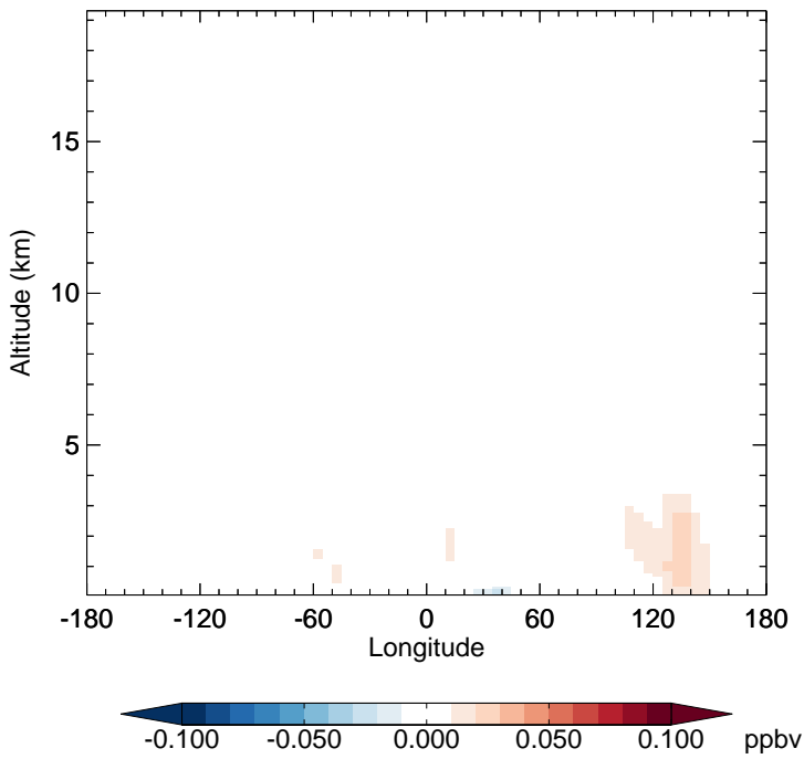
v11-01-public-Run0 - v11-01g-Run0 TSOG3 - Diff along 15S for Jan
