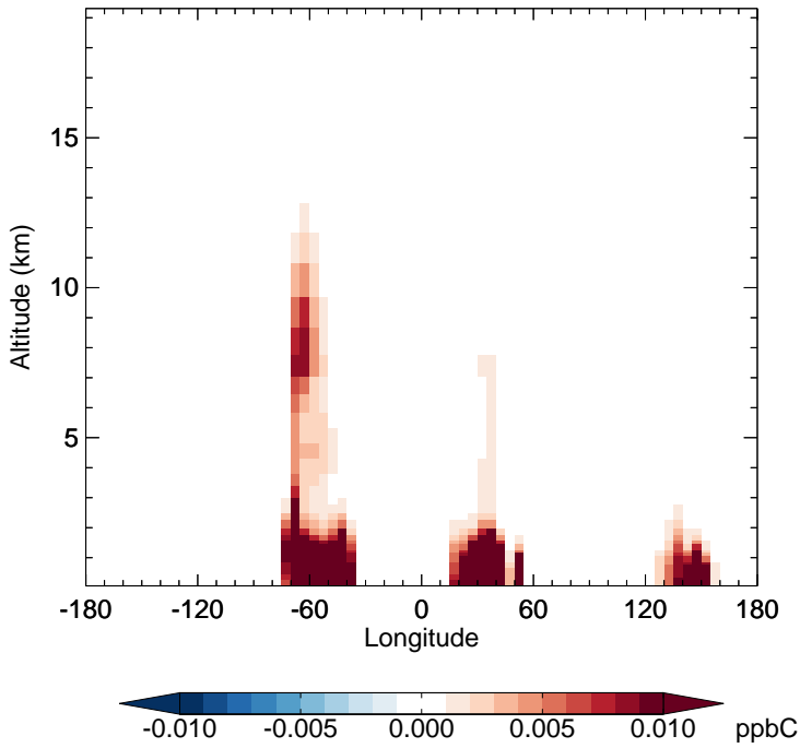
v11-01-public-Run0 - v11-01g-Run0 PRPE - Diff along 15S for Jan
