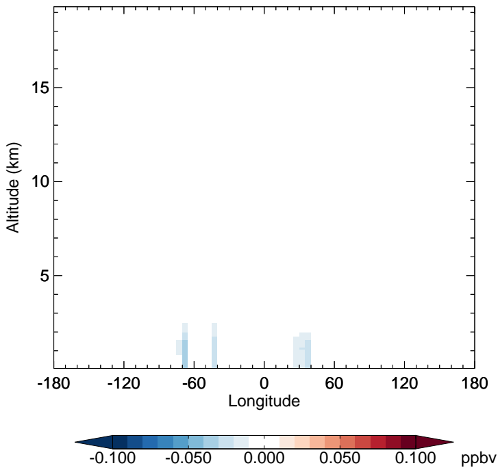
v11-01-public-Run0 - v11-01g-Run0 PAN - Diff along 15S for Jan
