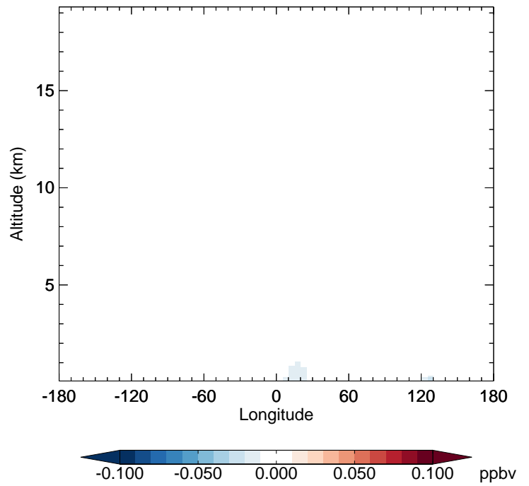
v11-01-public-Run0 - v11-01g-Run0 PAN - Diff along 42N for Jan
