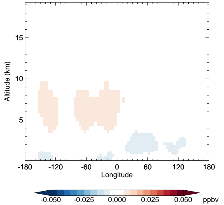
v11-01-public-Run0 - v11-01g-Run0 MP - Diff along 42N for Jan
