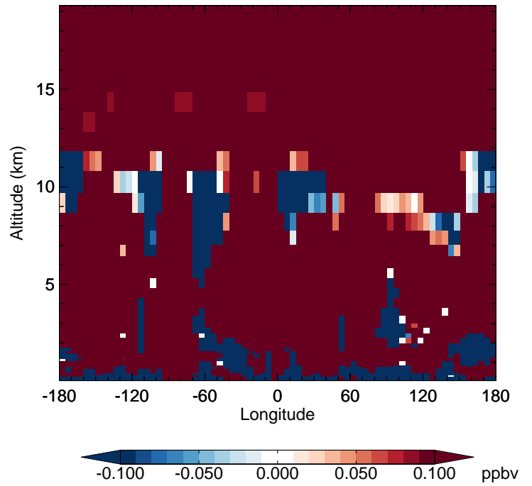
v11-01-public-Run0 - v11-01g-Run0 H2O - Diff along 42N for Jan
