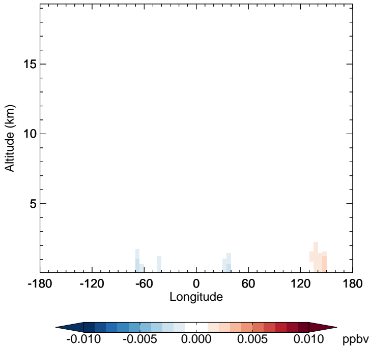
v11-01-public-Run0 - v11-01g-Run0 MVKN - Diff along 15S for Jan
