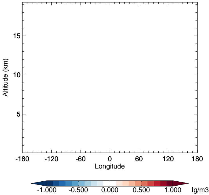
v11-01-public-Run0 - v11-01g-Run0 NIT - Diff along 15S for Jan
