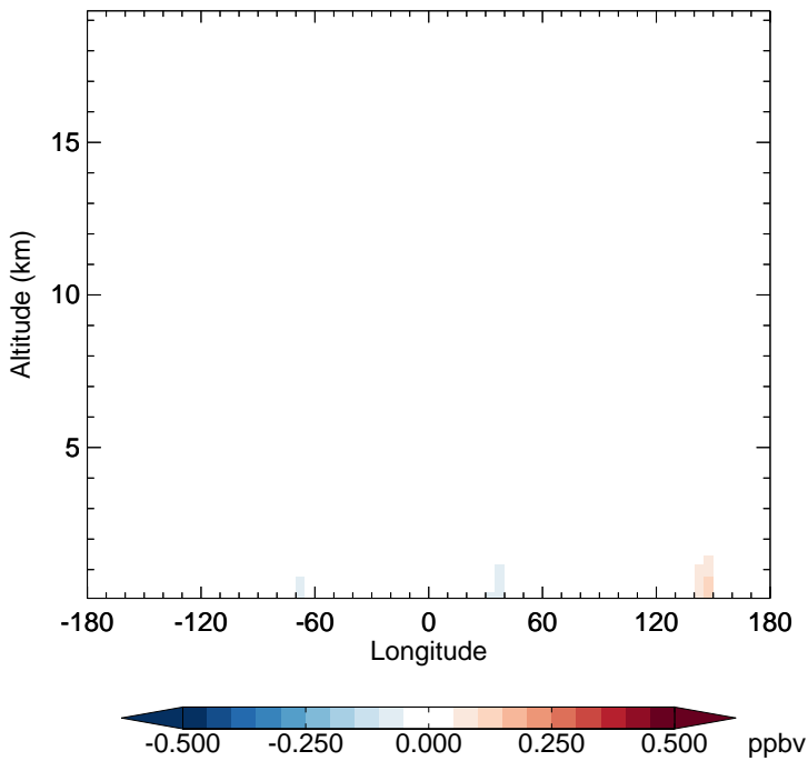
v11-01-public-Run0 - v11-01g-Run0 CH 2 O - Diff along 15S for Jan
