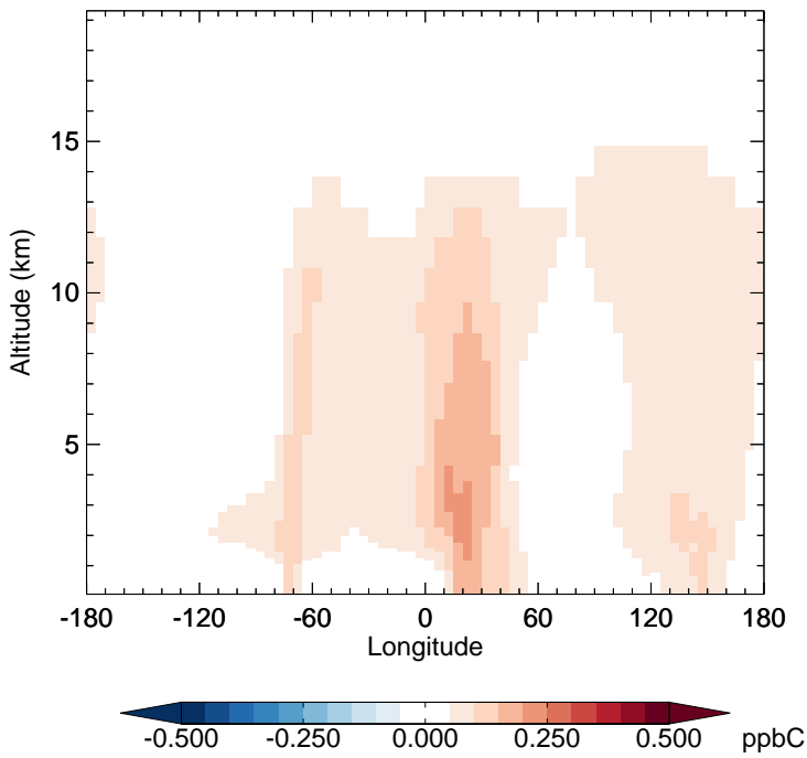
v11-01-public-Run0 - v11-01g-Run0 ACET - Diff along 15S for Jan
