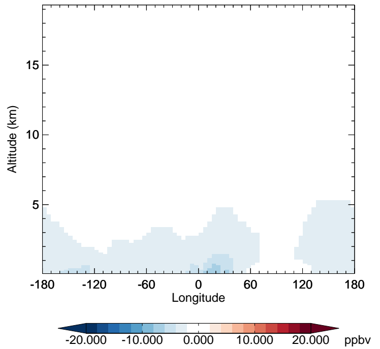
v11-01-public-Run0 - v11-01g-Run0 O3 - Diff along 42N for Jan
