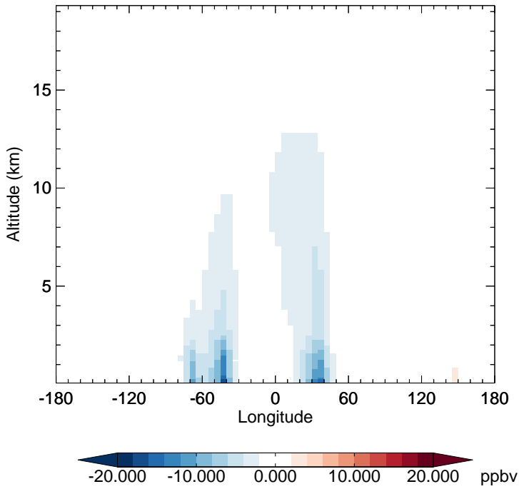
v11-01-public-Run0 - v11-01g-Run0 CO - Diff along 15S for Jan
