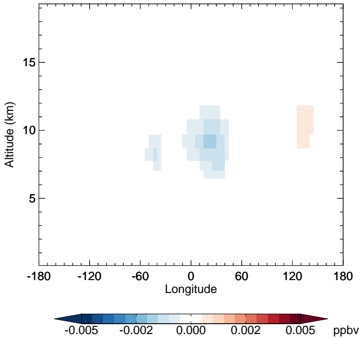
v11-01-public-Run0 - v11-01g-Run0 HNO 4 - Diff along 15S for Jan
