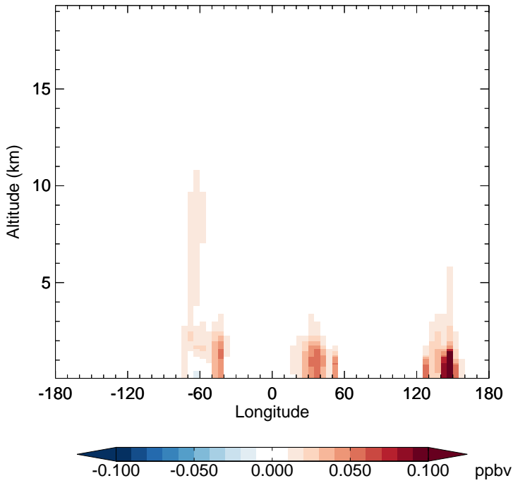
v11-01-public-Run0 - v11-01g-Run0 HAC - Diff along 15S for Jan
