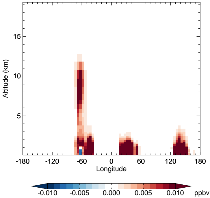
v11-01-public-Run0 - v11-01g-Run0 IEPOX - Diff along 15S for Jan
