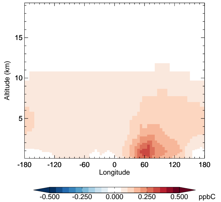
v11-01-public-Run0 - v11-01g-Run0 ACET - Diff along 42N for Jan
