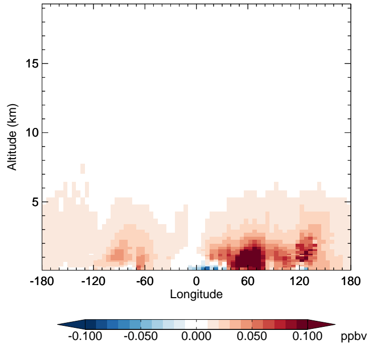
v11-01-public-Run0 - v11-01g-Run0 HNO 3 - Diff along 42N for Jan
