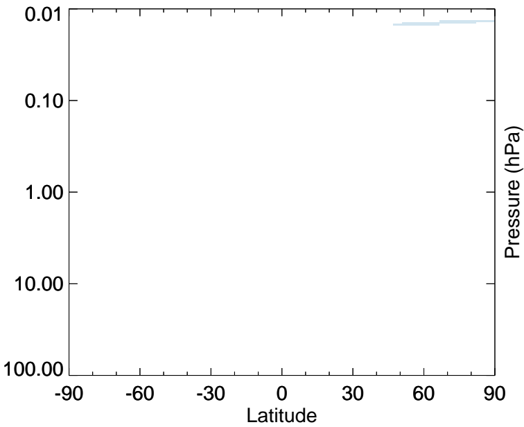
v11-01-public-Run0 - v11-01g-Run0 ClO - Strat zonal mean abs diff for Jan
