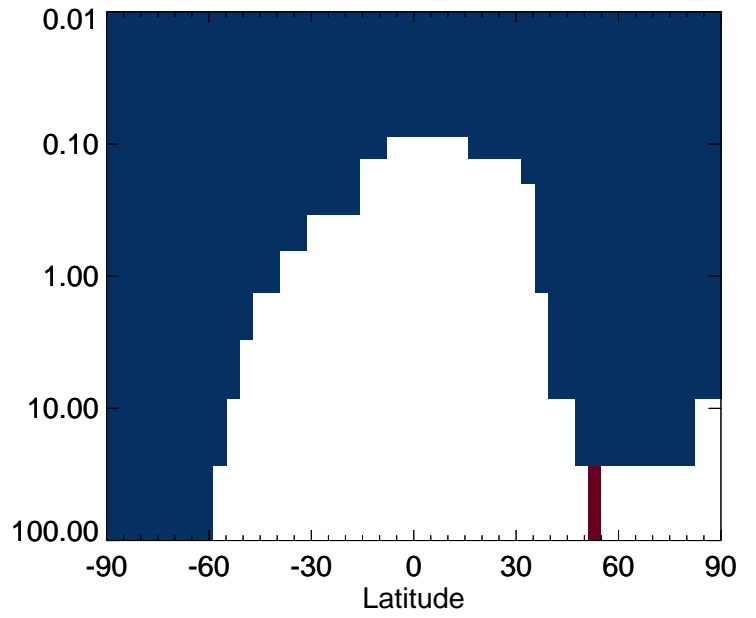
v11-01-public-Run0 / v11-01k-Run0 NIT - Strat zonal mean % diff for Jan
