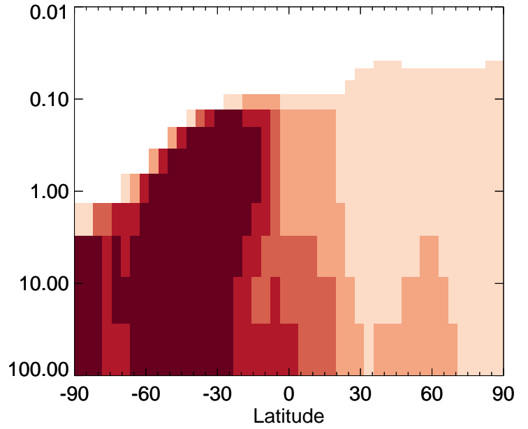
v11-01-public-Run0 / v11-01g-Run0 NITs - Strat zonal mean % diff for Jan
