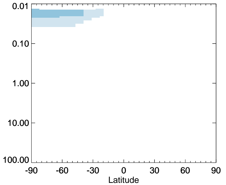
v11-01-public-Run0 / v11-01g-Run0 OCS - Strat zonal mean % diff for Jan
