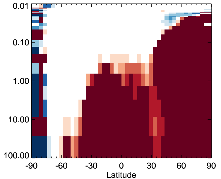
v11-01-public-Run0 / v11-01g-Run0 RIP - Strat zonal mean % diff for Jan
