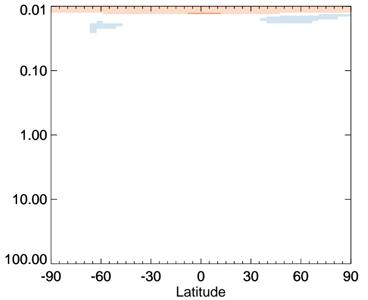
v11-01-public-Run0 / v11-01g-Run0 BrCl - Strat zonal mean % diff for Jan
