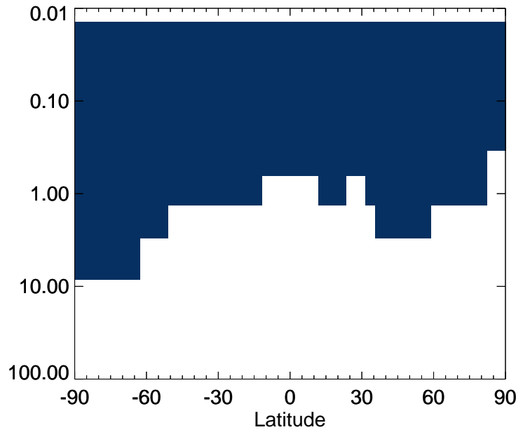
v11-01-public-Run0 / v11-01k-Run0 SO4s - Strat zonal mean % diff for Jan
