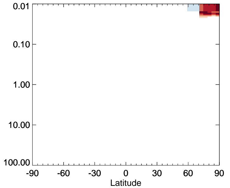
v11-01-public-Run0 / v11-01g-Run0 HO2 - Strat zonal mean % diff for Jan
