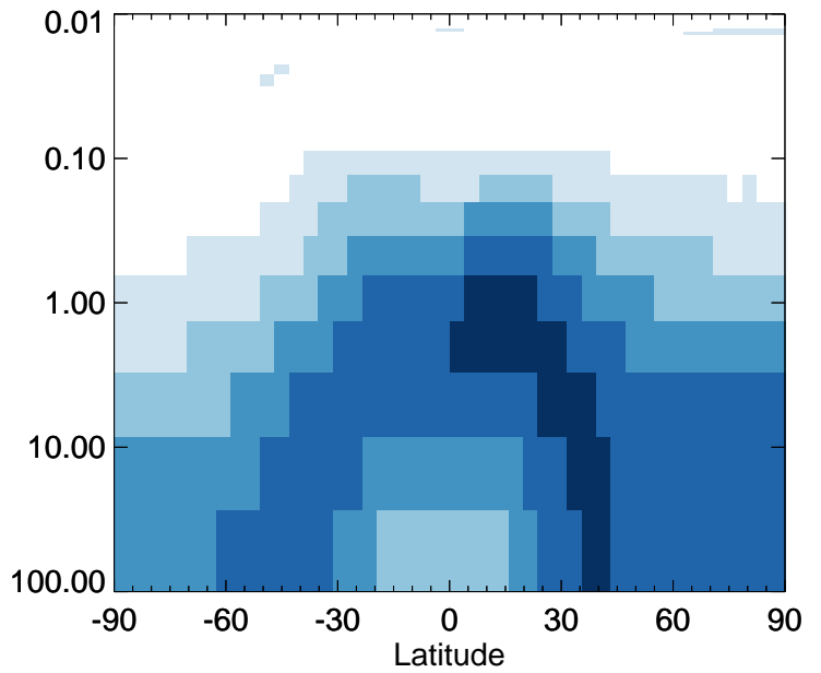
v11-01-public-Run0 / v11-01g-Run0 ALD2 - Strat zonal mean % diff for Jan
