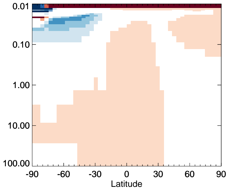
v11-01-public-Run0 / v11-01g-Run0 ALK4 - Strat zonal mean % diff for Jan
