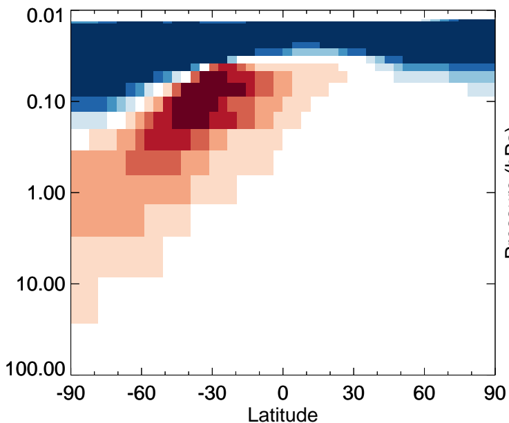
v11-01-public-Run0 - v11-01g-Run0 O3 - Strat zonal mean abs diff for Jan
