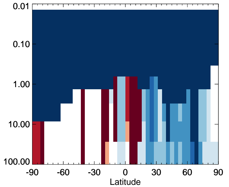
v11-01-public-Run0 / v11-01g-Run0 SO4s - Strat zonal mean % diff for Jan
