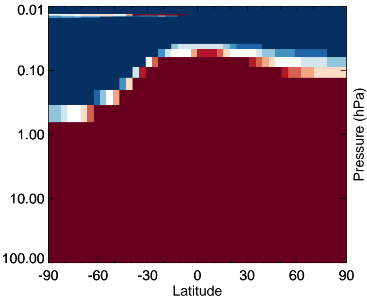
v11-01-public-Run0 - v11-01g-Run0 N2O - Strat zonal mean abs diff for Jan
