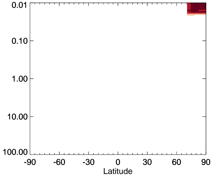
v11-01-public-Run0 / v11-01g-Run0 OH - Strat zonal mean % diff for Jan
