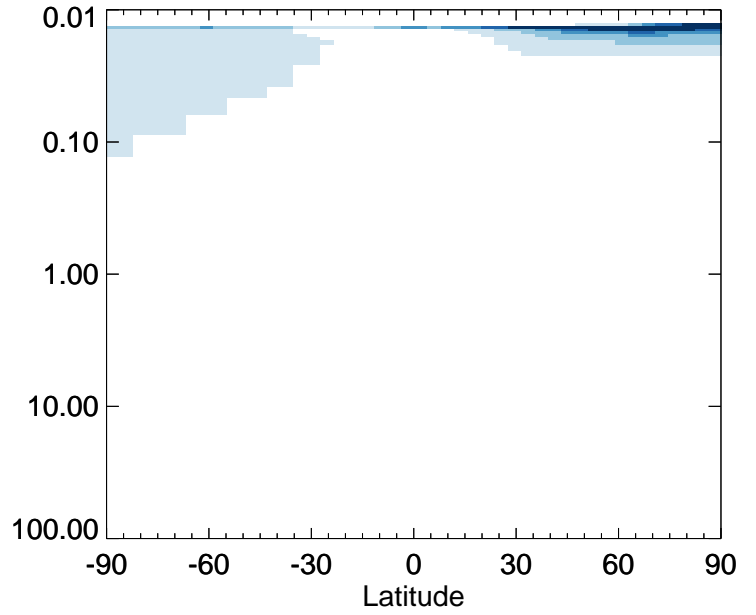
v11-01-public-Run0 / v11-01g-Run0 MP - Strat zonal mean % diff for Jan
