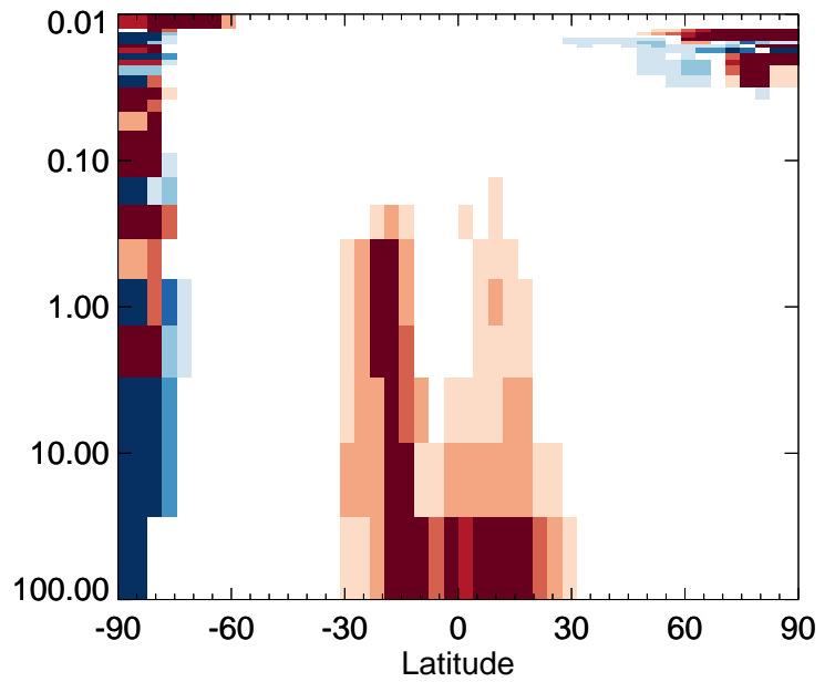
v11-01-public-Run0 / v11-01g-Run0 PMN - Strat zonal mean % diff for Jan
