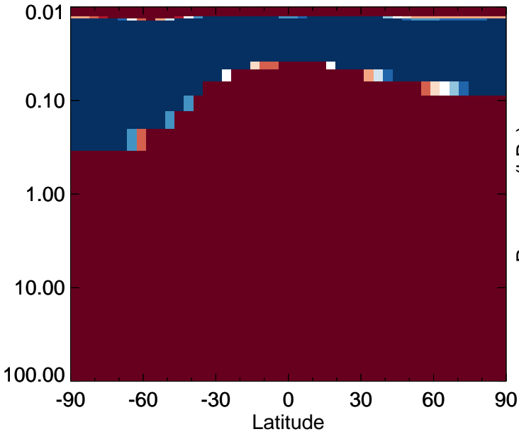
v11-01-public-Run0 - v11-01g-Run0 CH4 - Strat zonal mean abs diff for Jan
