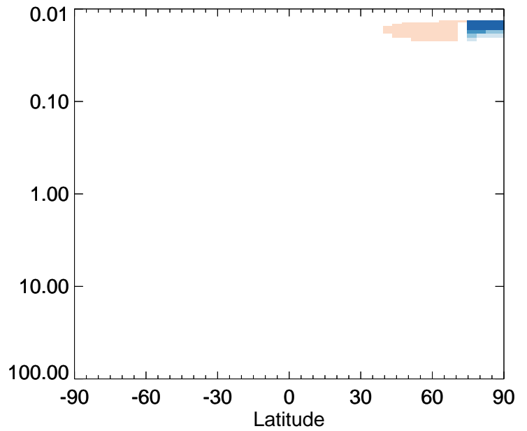
v11-01-public-Run0 / v11-01g-Run0 CIOO - Strat zonal mean % diff for Jan
