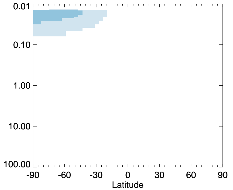
v11-01-public-Run0 / v11-01g-Run0 CCI4 - Strat zonal mean % diff for Jan
