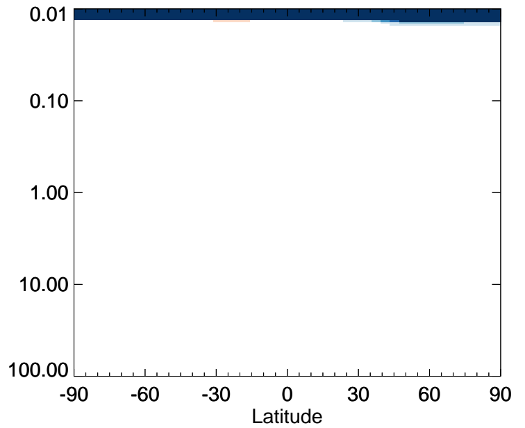
v11-01-public-Run0 / v11-01g-Run0 N2O - Strat zonal mean % diff for Jan
