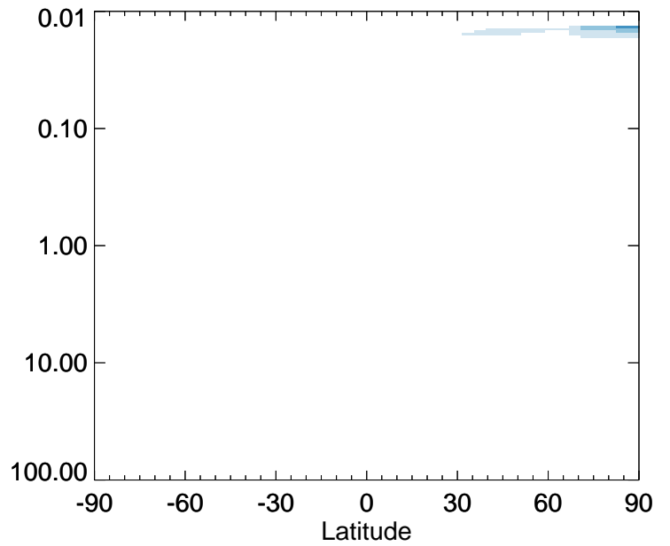
v11-01-public-Run0 / v11-01g-Run0 Cl2 - Strat zonal mean % diff for Jan
