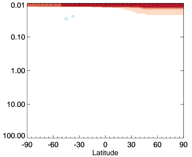
v11-01-public-Run0 / v11-01g-Run0 SO 2 - Strat zonal mean % diff for Jan
