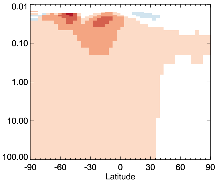
v11-01-public-Run0 / v11-01g-Run0 MEK - Strat zonal mean % diff for Jan
