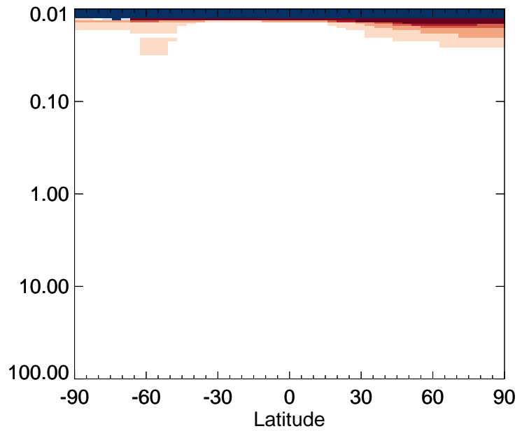
v11-01-public-Run0 / v11-01g-Run0 NO2 - Strat zonal mean % diff for Jan
