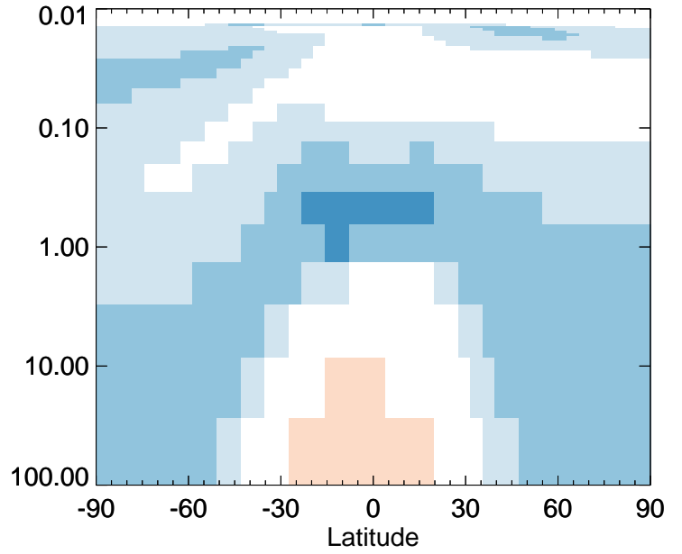
v11-01-public-Run0 / v11-01g-Run0 MAP - Strat zonal mean % diff for Jan
