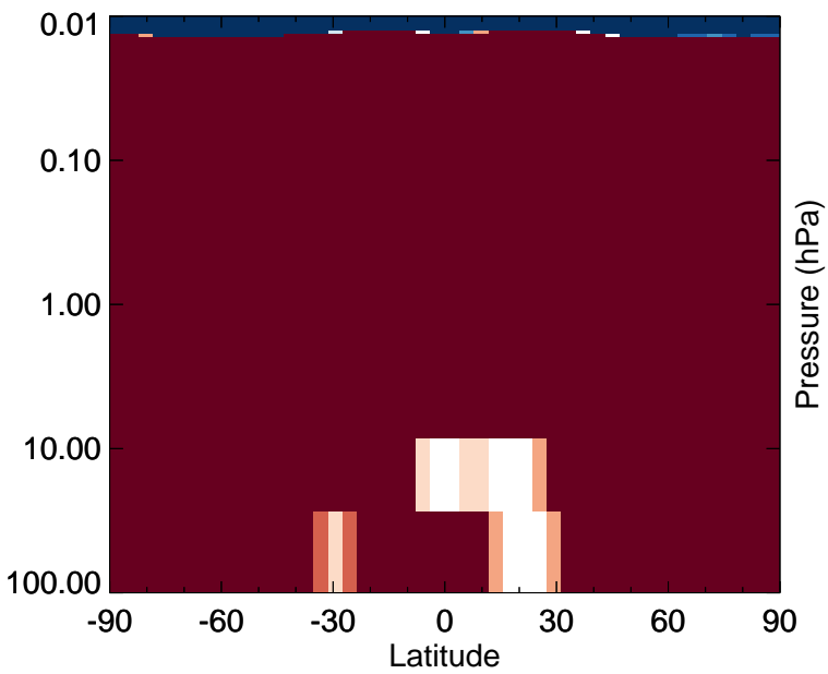
v11-01-public-Run0 - v11-01g-Run0 H2O - Strat zonal mean abs diff for Jan
