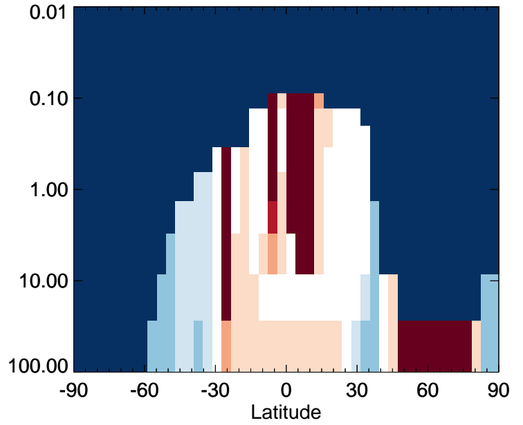
v11-01-public-Run0 / v11-01g-Run0 NIT - Strat zonal mean % diff for Jan
