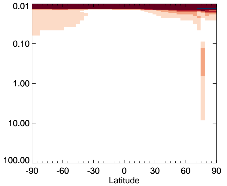
v11-01-public-Run0 / v11-01g-Run0 NO - Strat zonal mean % diff for Jan
