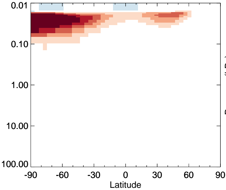
v11-01-public-Run0 - v11-01g-Run0 OH - Strat zonal mean abs diff for Jan
