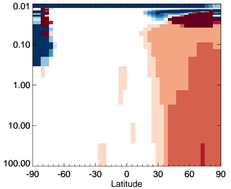
v11-01-public-Run0 / v11-01g-Run0 DMS - Strat zonal mean % diff for Jan
