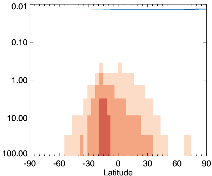
v11-01-public-Run0 / v11-01g-Run0 LIMO - Strat zonal mean % diff for Jan
