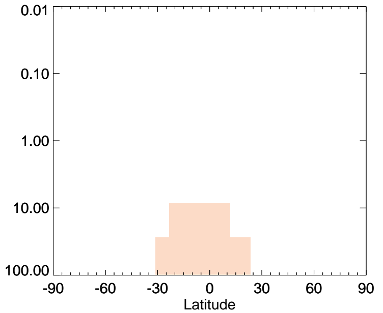
v11-01-public-Run0 / v11-01g-Run0 BCPI - Strat zonal mean % diff for Jan
