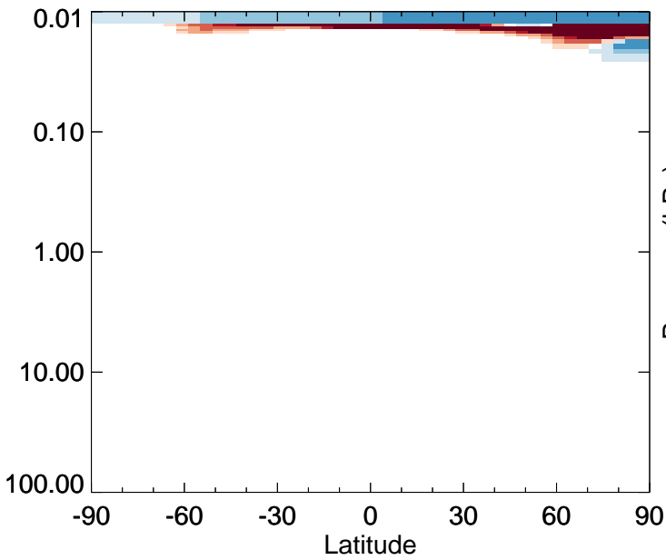
v11-01-public-Run0 - v11-01g-Run0 NO3 - Strat zonal mean abs diff for Jan
