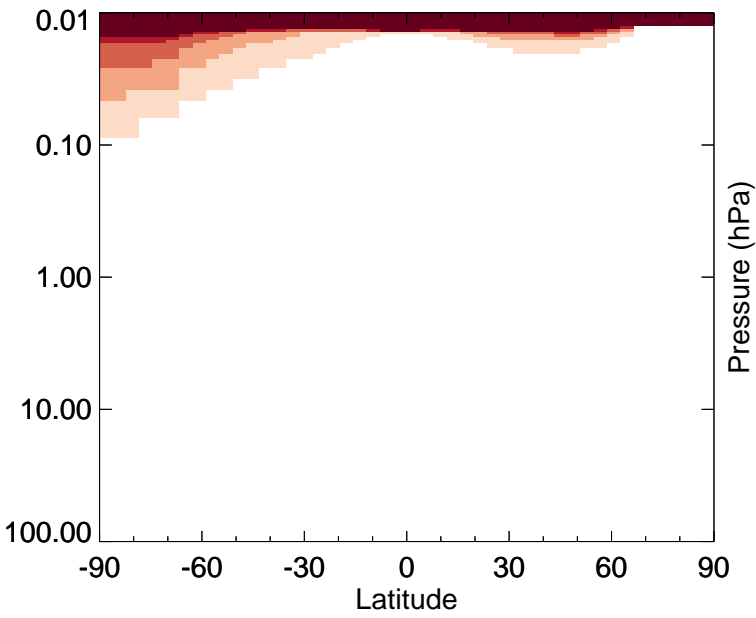
v11-01-public-Run0 - v11-01g-Run0 NO - Strat zonal mean abs diff for Jan
