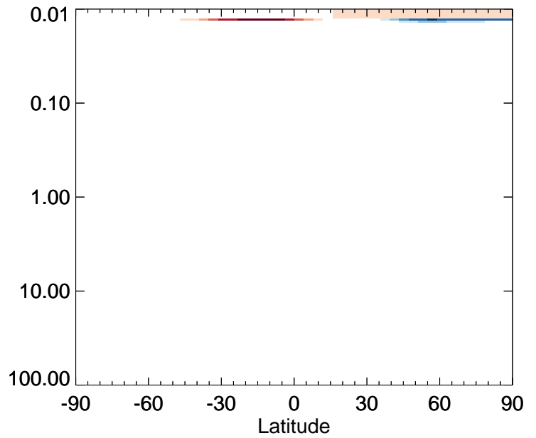
v11-01-public-Run0 / v11-01g-Run0 MPN - Strat zonal mean % diff for Jan
