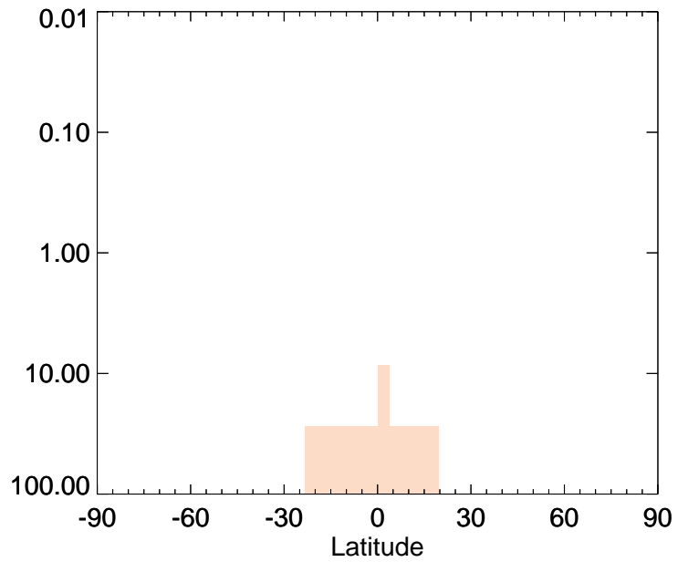
v11-01-public-Run0 / v11-01g-Run0 MSA - Strat zonal mean % diff for Jan
