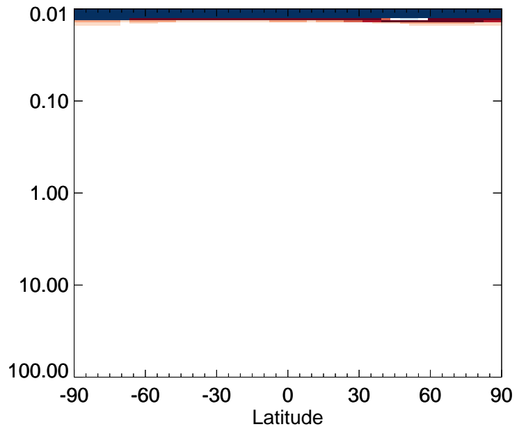
v11-01-public-Run0 / v11-01g-Run0 NO3 - Strat zonal mean % diff for Jan
