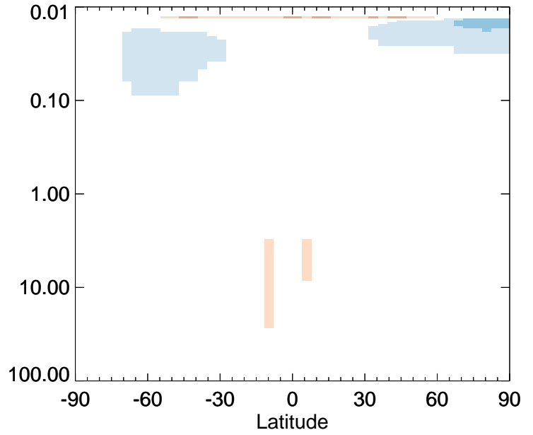
v11-01-public-Run0 / v11-01g-Run0 OCIO - Strat zonal mean % diff for Jan
