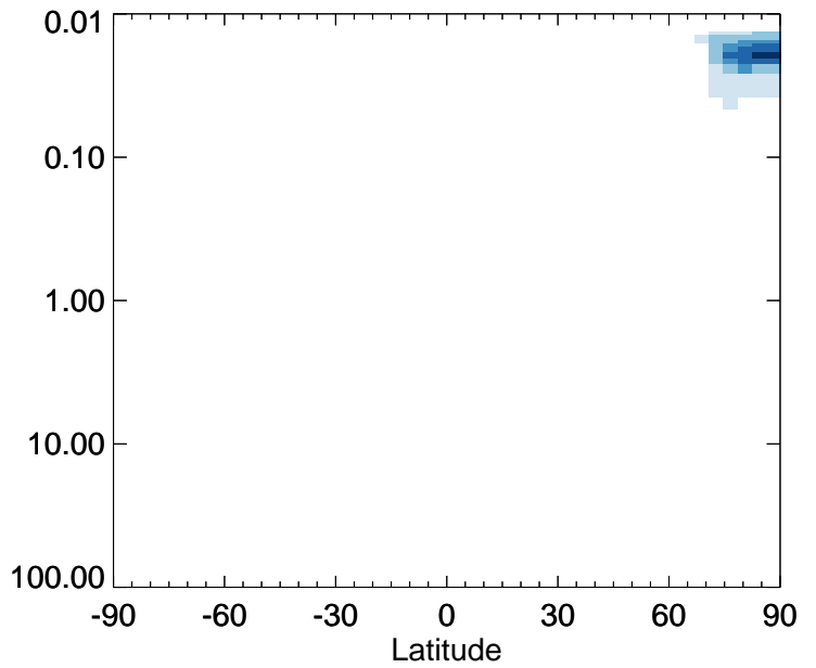
v11-01-public-Run0 / v11-01g-Run0 BrO - Strat zonal mean % diff for Jan
