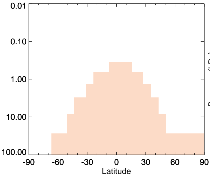
v11-01-public-Run0 - v11-01g-Run0 PPN - Strat zonal mean abs diff for Jan
