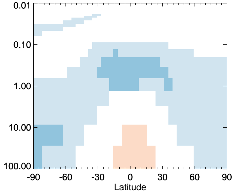
v11-01-public-Run0 / v11-01g-Run0 PAN - Strat zonal mean % diff for Jan
