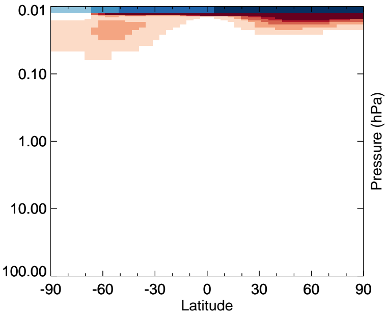
v11-01-public-Run0 - v11-01g-Run0 NO2 - Strat zonal mean abs diff for Jan
