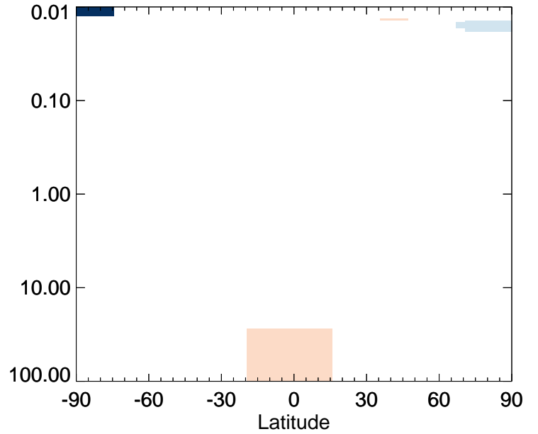
v11-01-public-Run0 / v11-01g-Run0 Br2 - Strat zonal mean % diff for Jan
