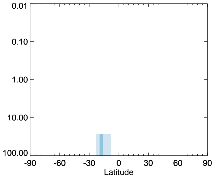
v11-01-public-Run0 / v11-01g-Run0 NH3 - Strat zonal mean % diff for Jan
