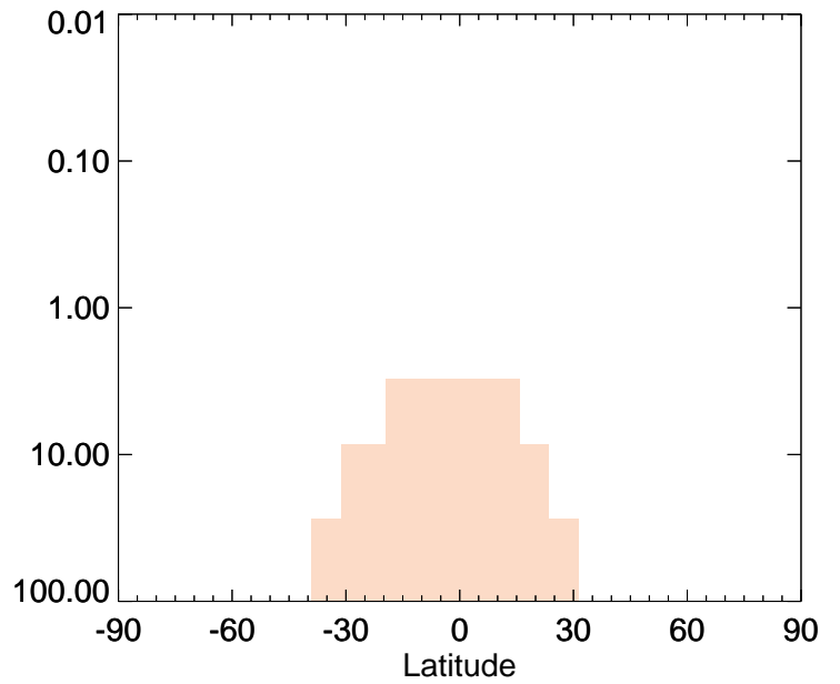
v11-01-public-Run0 / v11-01g-Run0 PPN - Strat zonal mean % diff for Jan
