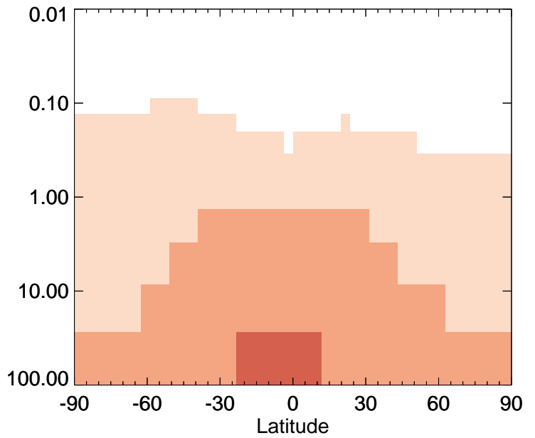
v11-01-public-Run0 / v11-01g-Run0 SALA - Strat zonal mean % diff for Jan
