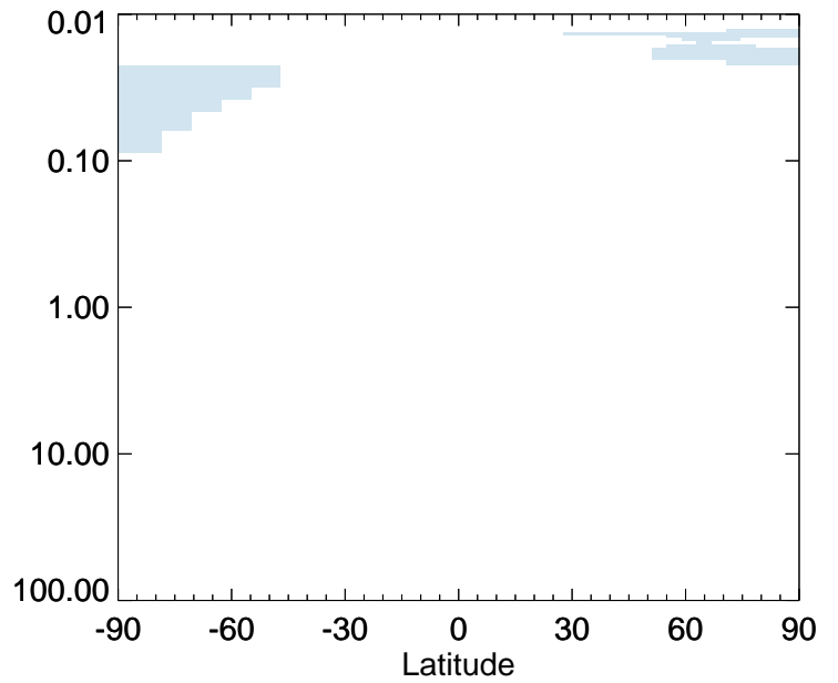
v11-01-public-Run0 / v11-01g-Run0 HOCl - Strat zonal mean % diff for Jan
