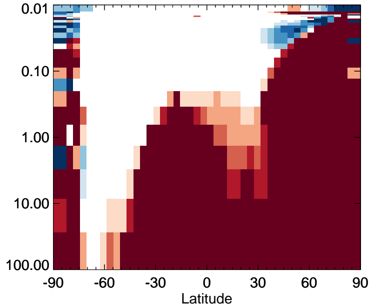
v11-01-public-Run0 / v11-01g-Run0 ISOP - Strat zonal mean % diff for Jan
