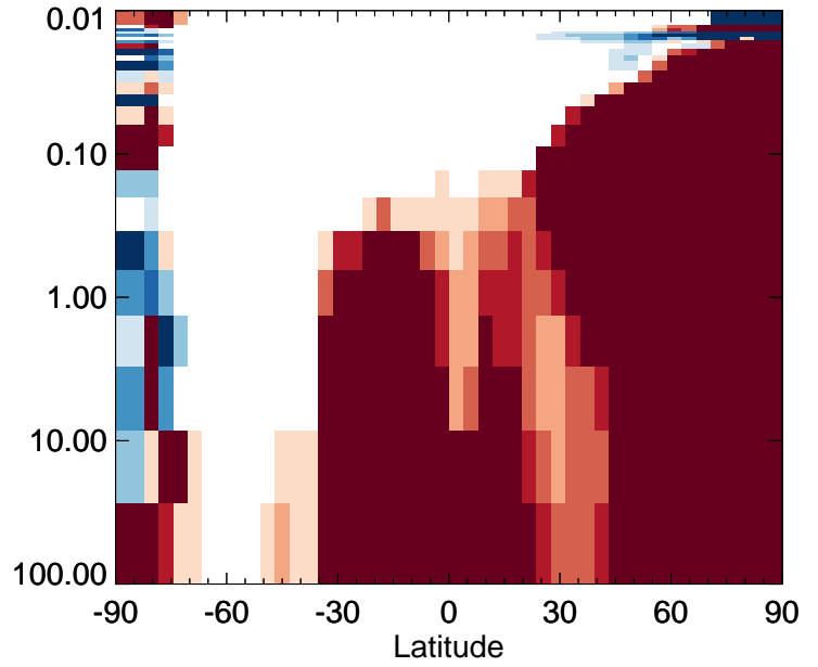
v11-01-public-Run0 / v11-01g-Run0 MVK - Strat zonal mean % diff for Jan
