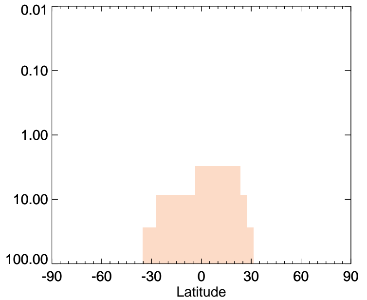
v11-01-public-Run0 / v11-01g-Run0 NH4 - Strat zonal mean % diff for Jan
