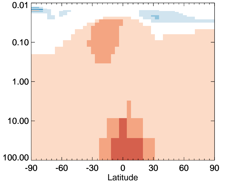
v11-01-public-Run0 / v11-01g-Run0 HAC - Strat zonal mean % diff for Jan
