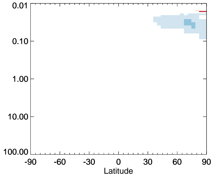
v11-01-public-Run0 / v11-01k-Run0 DMS - Strat zonal mean % diff for Jan
