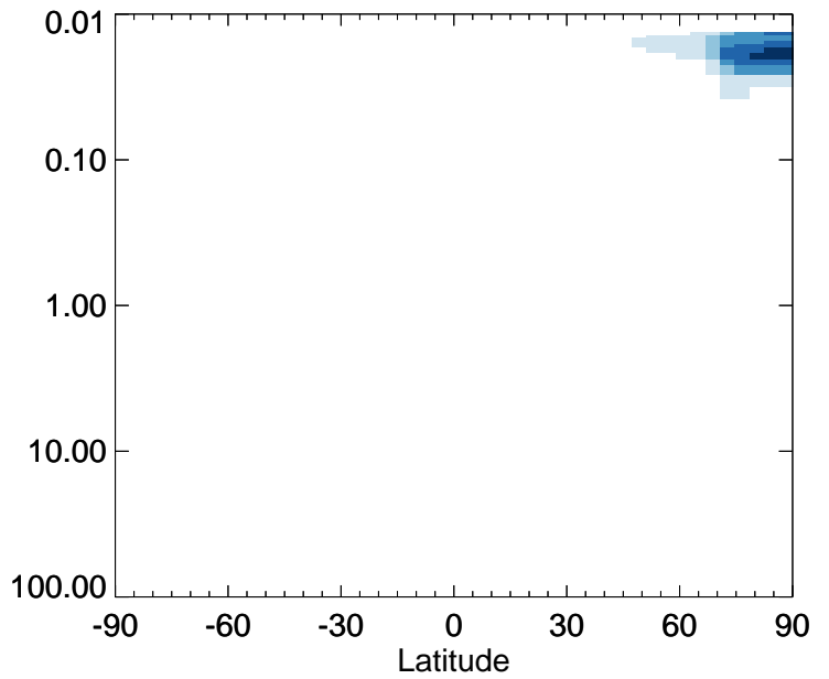
v11-01-public-Run0 / v11-01g-Run0 ClO - Strat zonal mean % diff for Jan
