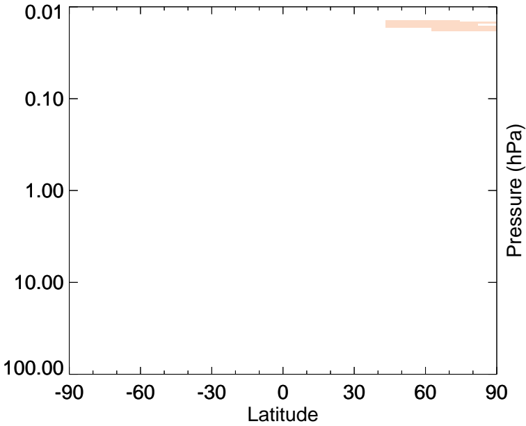
v11-01-public-Run0 - v11-01g-Run0 HCl - Strat zonal mean abs diff for Jan
