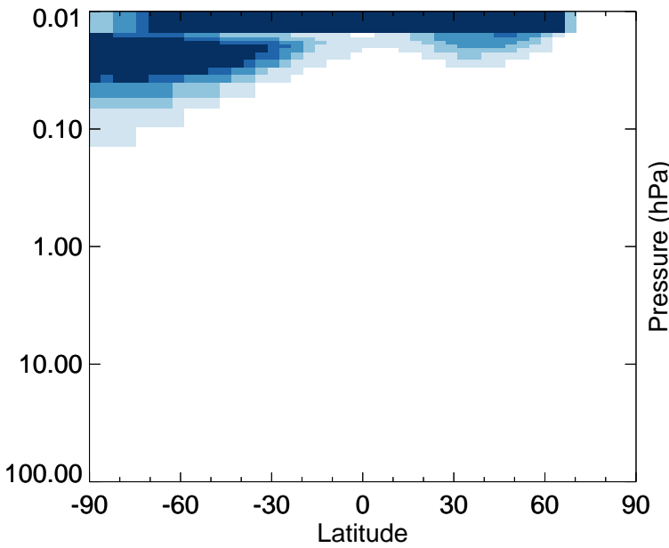
v11-01-public-Run0 - v11-01g-Run0 HO2 - Strat zonal mean abs diff for Jan
