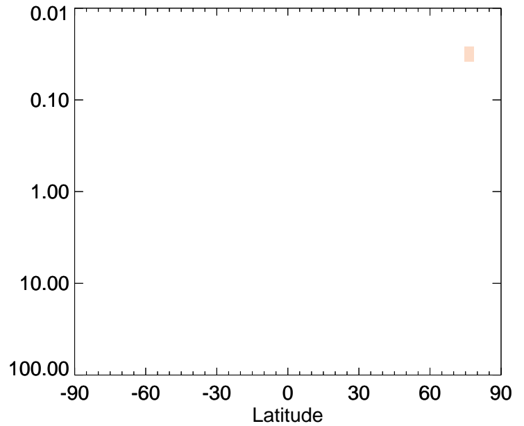
v11-01-public-Run0 / v11-01k-Run0 RIP - Strat zonal mean % diff for Jan
