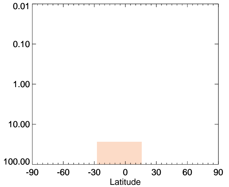
v11-01-public-Run0 / v11-01g-Run0 OCPI - Strat zonal mean % diff for Jan
