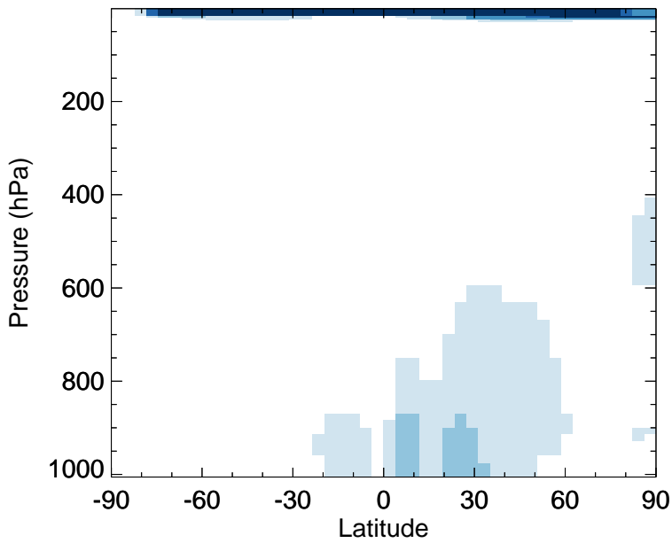
v11-01-public-Run0 - v11-01g-Run0 HO2 - Zonal mean abs diff for Apr
