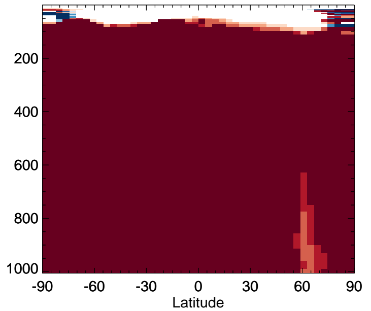
v11-01-public-Run0 / v11-01g-Run0 MOBA - Zonal mean % diff for Apr
