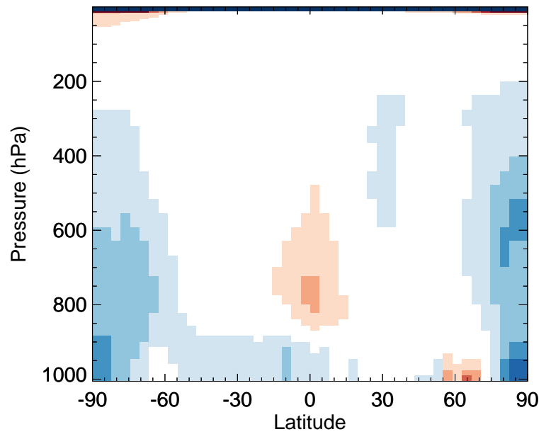
v11-01-public-Run0 / v11-01g-Run0 NO2 - Zonal mean % diff for Apr
