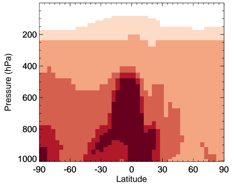
v11-01-public-Run0 / v11-01g-Run0 BCPI - Zonal mean % diff for Apr
