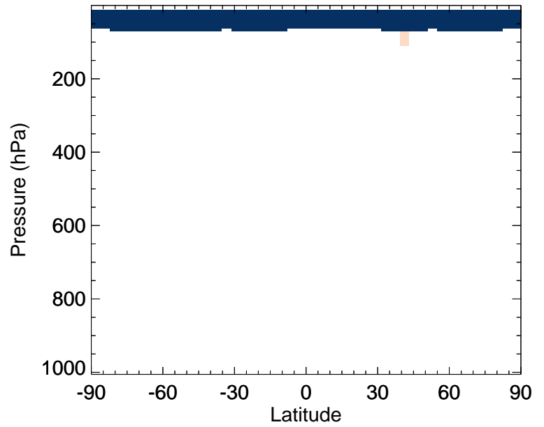
v11-01-public-Run0 / v11-01k-Run0 SO4s - Zonal mean % diff for Apr
