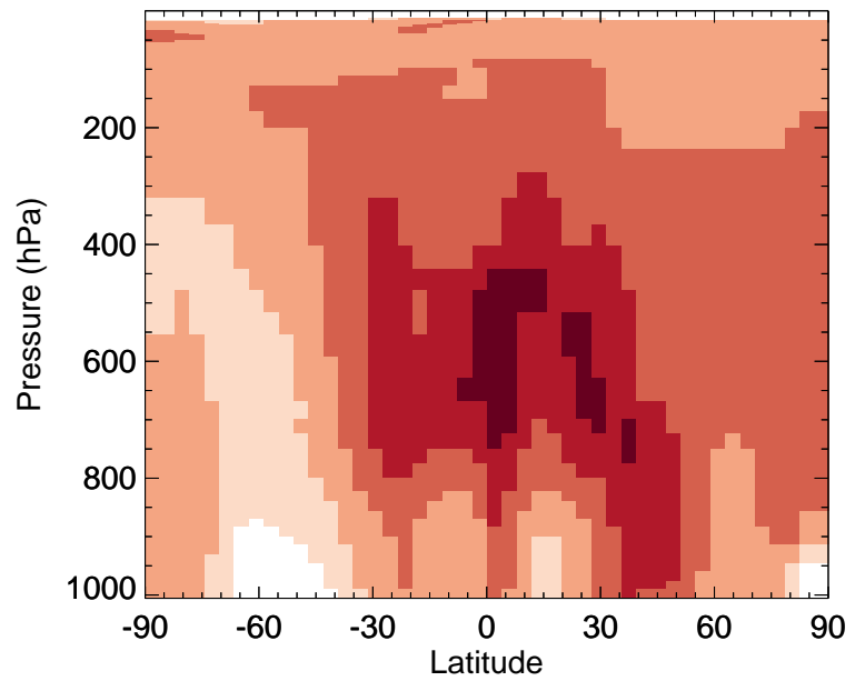
v11-01-public-Run0 / v11-01g-Run0 SALC - Zonal mean % diff for Apr
