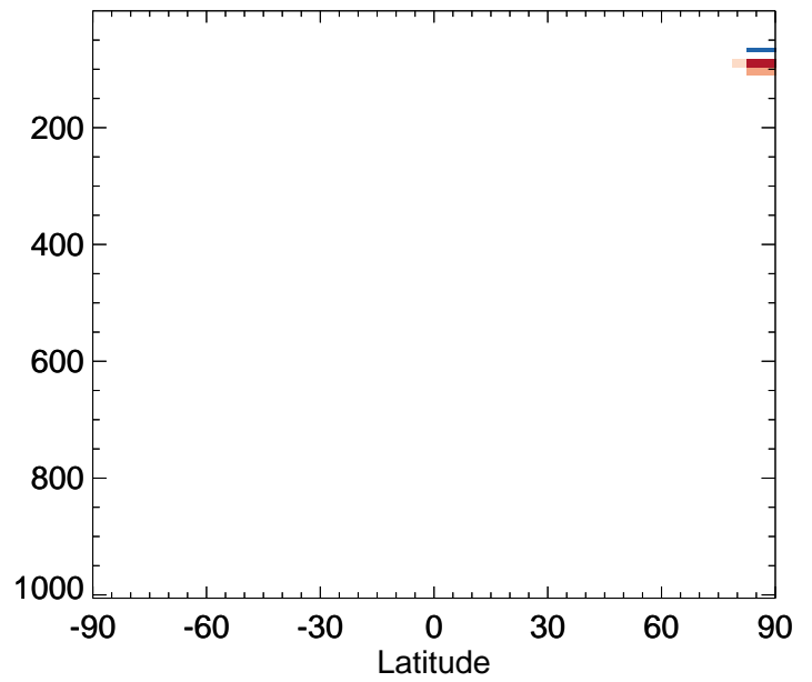
v11-01-public-Run0 / v11-01k-Run0 MOBA - Zonal mean % diff for Apr
