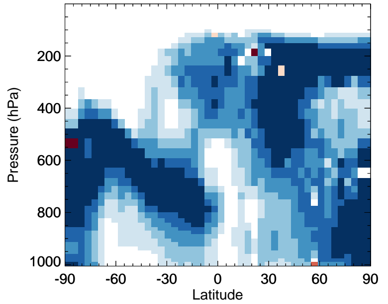
v11-01-public-Run0 / v11-01g-Run0 NH3 - Zonal mean % diff for Apr
