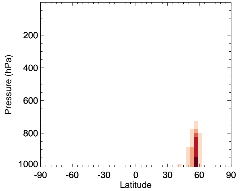
v11-01-public-Run0 / v11-01k-Run0 OCIO - Zonal mean % diff for Apr
