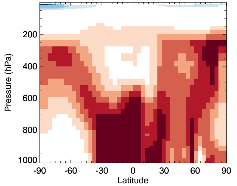
v11-01-public-Run0 / v11-01g-Run0 OCIO - Zonal mean % diff for Apr
