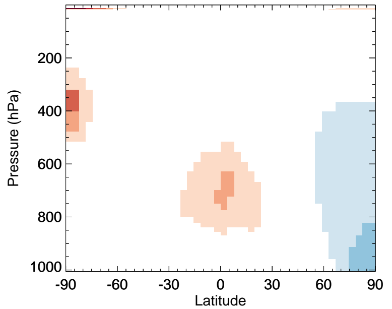
v11-01-public-Run0 / v11-01g-Run0 ClOO - Zonal mean % diff for Apr
