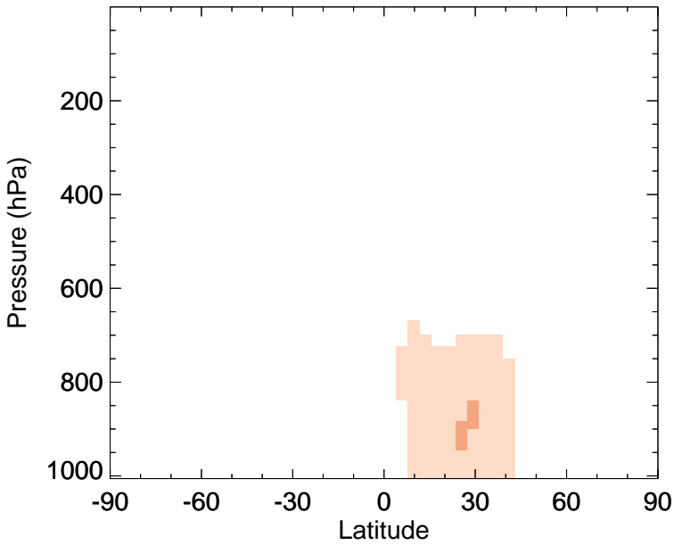
v11-01-public-Run0 - v11-01g-Run0 DST2 - Zonal mean abs diff for Apr
