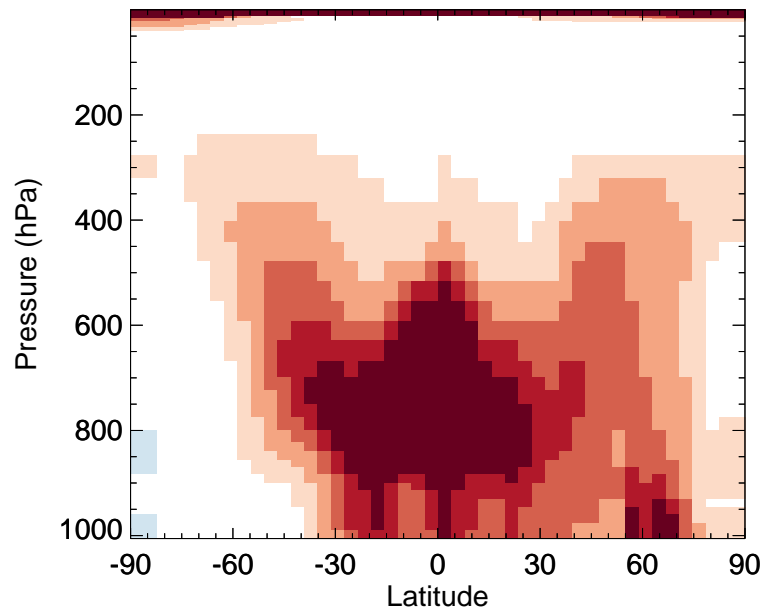
v11-01-public-Run0 / v11-01g-Run0 BrNO2 - Zonal mean % diff for Apr
