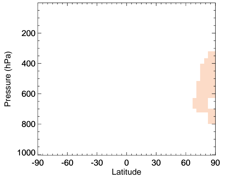
v11-01-public-Run0 / v11-01k-Run0 MTPA - Zonal mean % diff for Apr
