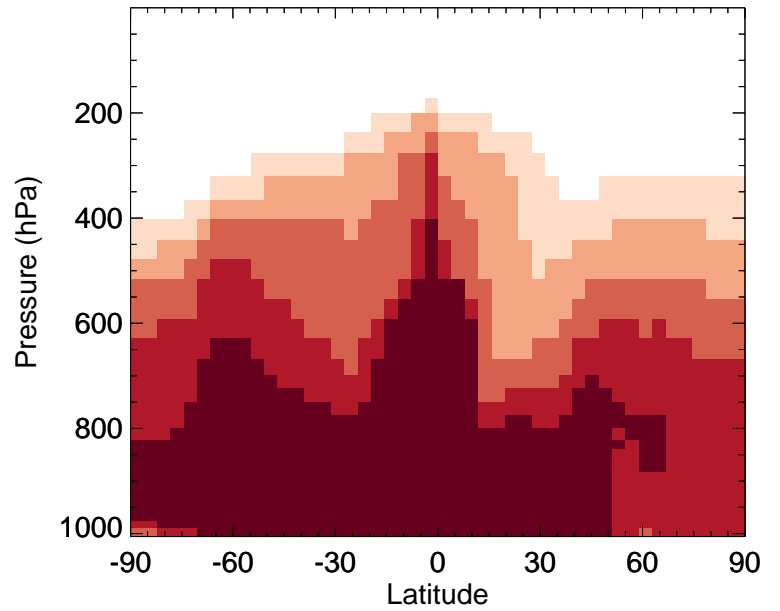
v11-01-public-Run0 / v11-01g-Run0 ISO G 1 - Zonal mean % diff for Apr
