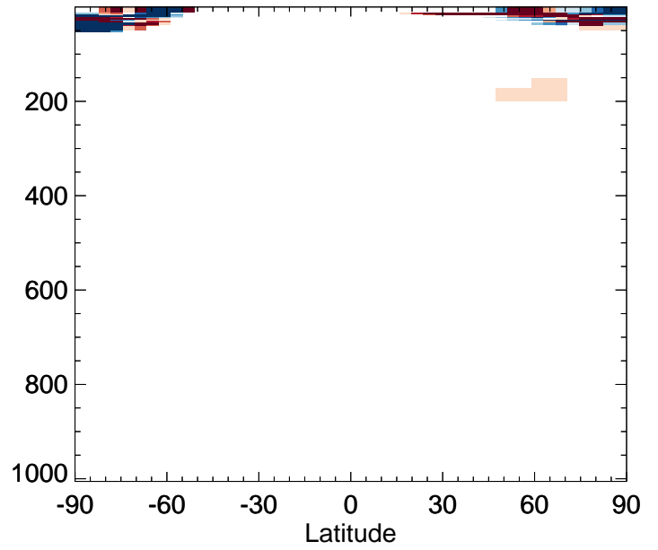
v11-01-public-Run0 / v11-01g-Run0 OCPO - Zonal mean % diff for Apr
