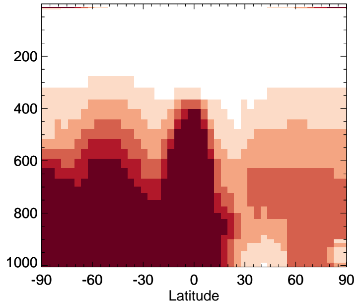
v11-01-public-Run0 / v11-01g-Run0 HNO 3 - Zonal mean % diff for Apr
