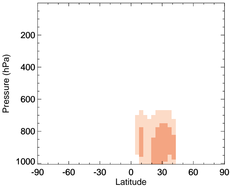
v11-01-public-Run0 - v11-01g-Run0 DST3 - Zonal mean abs diff for Apr
