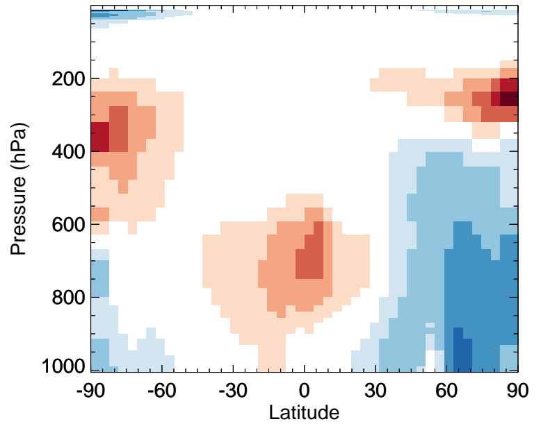
v11-01-public-Run0 / v11-01g-Run0 Cl2O2 - Zonal mean % diff for Apr
