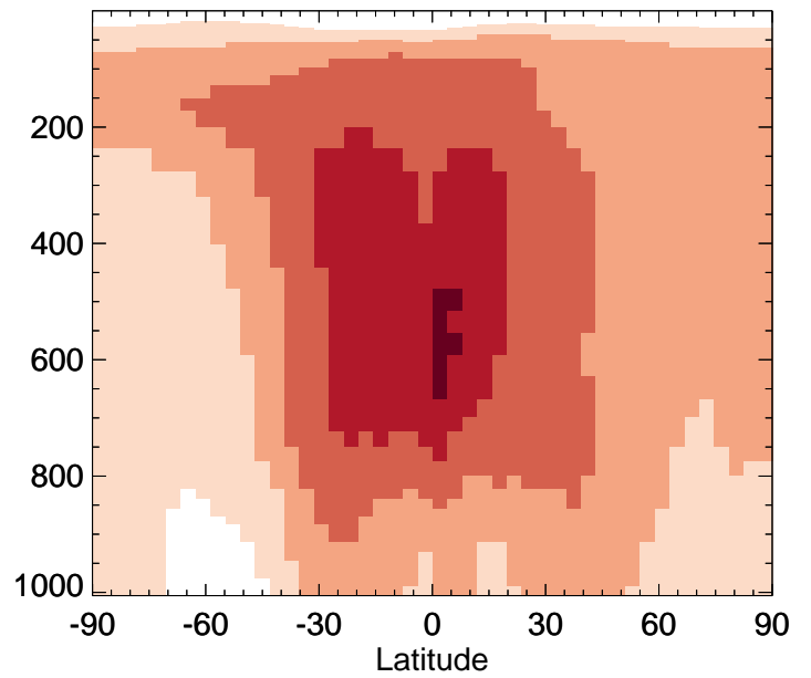
v11-01-public-Run0 / v11-01g-Run0 SALA - Zonal mean % diff for Apr
