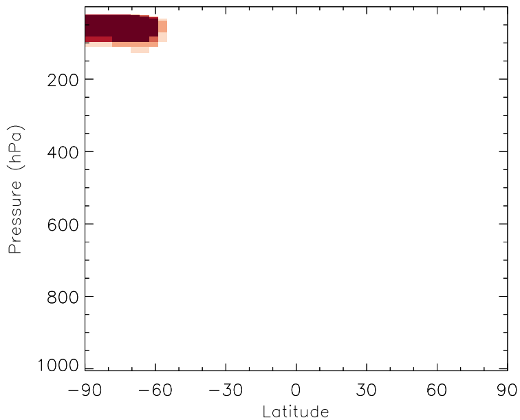
v11-01b-Run0 - v10-01i-geosfp-Run0 Cl2O2 - Zonal mean abs diff for Jul
