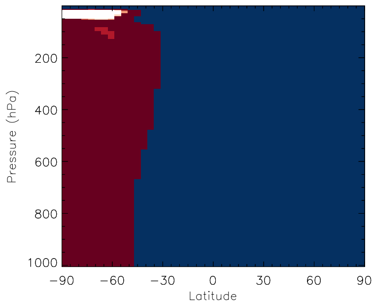
v11-01b-Run0 / v10-01-public-Run0 CIN02 - Zonal mean % diff for Jul
