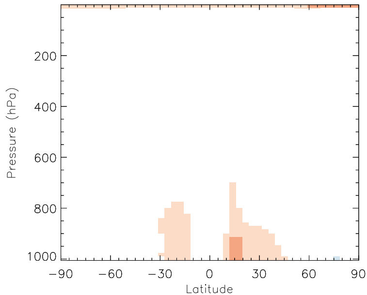
v11-01b-Run0 / v10-01i-geosfp-Run0 PPN - Zonal mean % diff for Jul
