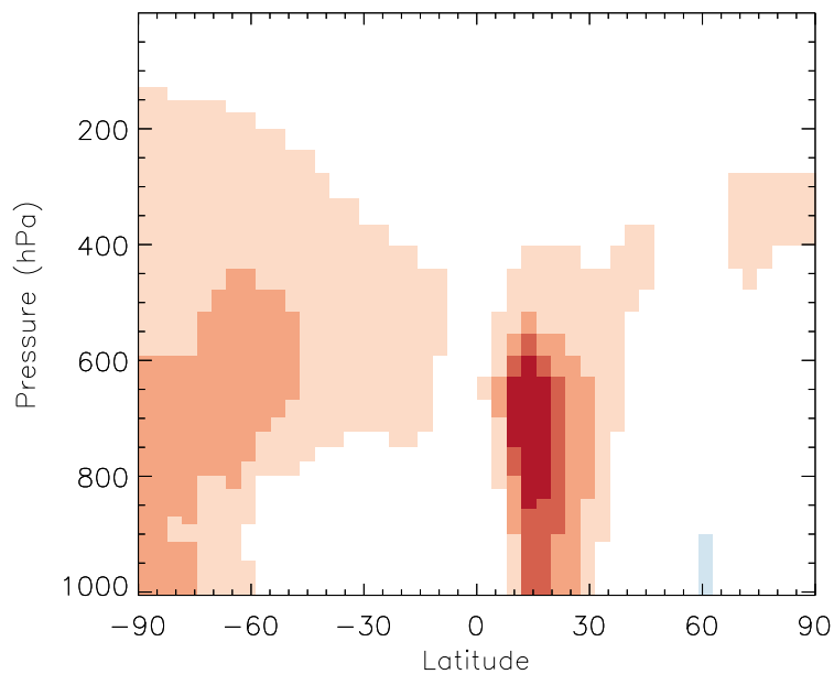
v11-01b-Run0 / v10-01-public-Run0 HN04 - Zonal mean % diff for Jul
