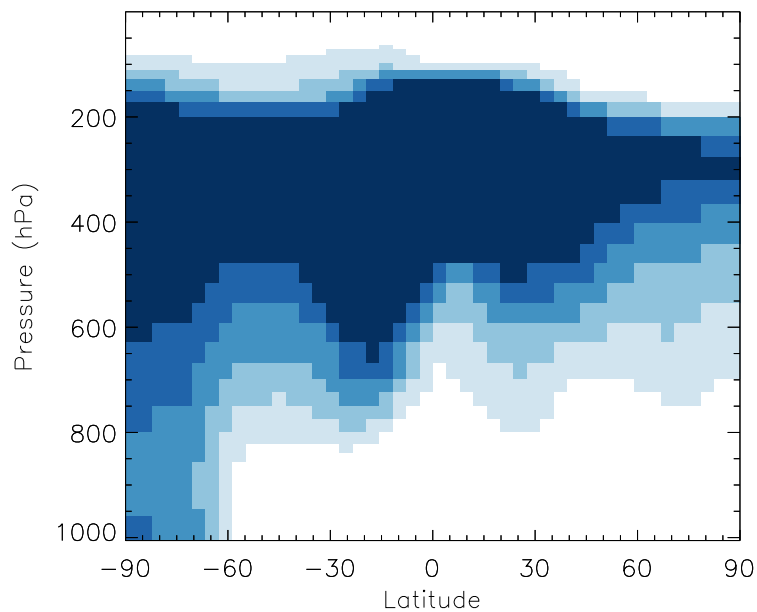
v11-01b-Run0 / v10-01-public-Run0 SO4 - Zonal mean % diff for Jul
