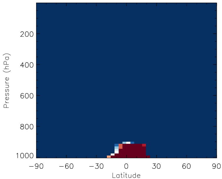
v11-01b-Run0 - v10-01i-geosfp-Run0 CH4 - Zonal mean abs diff for Jul
