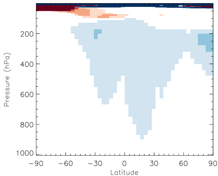
v11-01b-Run0 / v10-01-public-Run0 HAC - Zonal mean % diff for Jul
