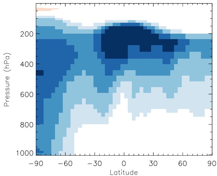
v11-01b-Run0 / v10-01-public-Run0 SO2 - Zonal mean % diff for Jul
