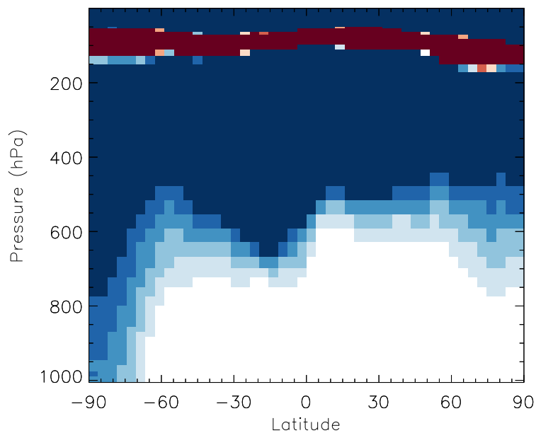
v11-01b-Run0 / v10-01-public-Run0 NITs - Zonal mean % diff for Jul
