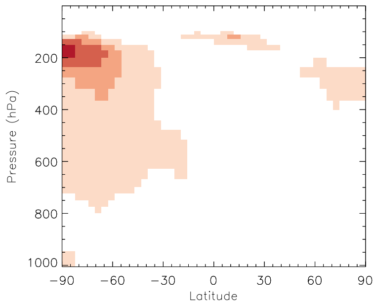
v11-01b-Run0 / v10-01-public-Run0 NO2 - Zonal mean % diff for Jul
