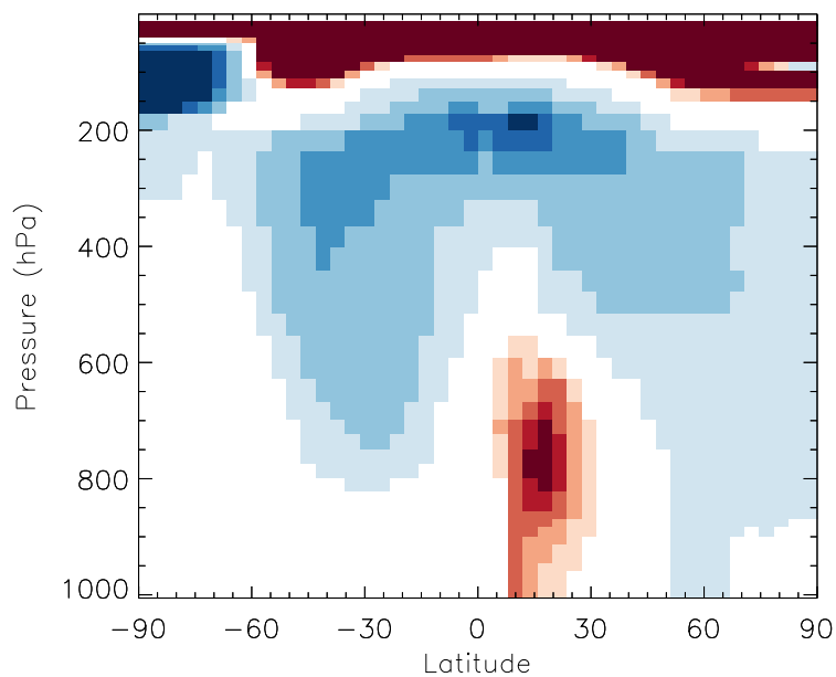
v11-01b-Run0 / v10-01i-geosp-Run0 HOBr - Zonal mean % diff for Jul
