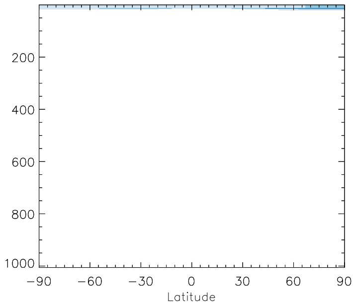
v11-01b-Run0 / v10-01i-geosfp-Run0 CFC12 - Zonal mean % diff for Jul
