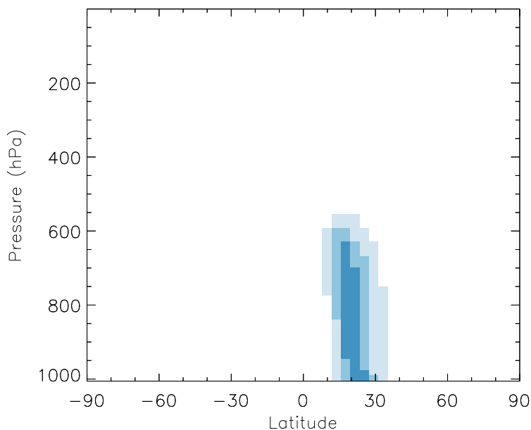
v11-01b-Run0 - v10-01i-geosfp-Run0 DST1 - Zonal mean abs diff for Jul
