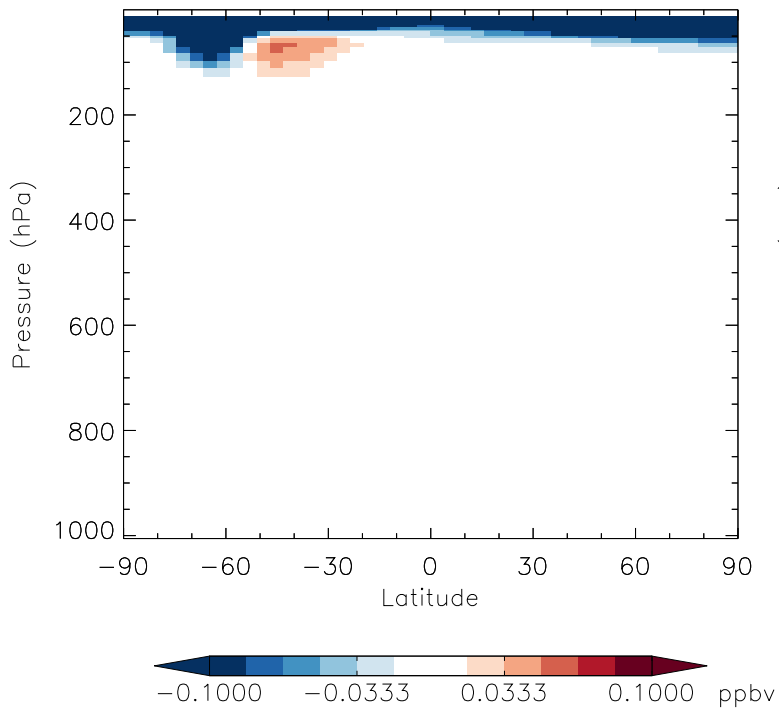
v11-01b-Run0 - v10-01i-geosfp-Run0 HCl - Zonal mean abs diff for Jul
