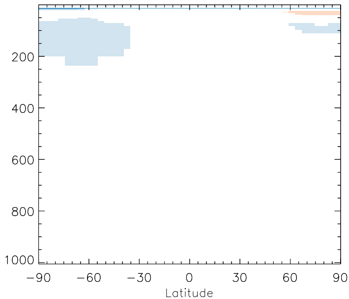
v11-01b-Run0 / v10-01i-geosfp-Run0 O3 - Zonal mean % diff for Jul
