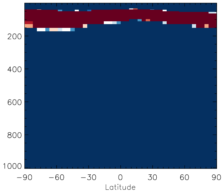
v11-01b-Run0 / v10-01i-geosfp-Run0 DST3 - Zonal mean % diff for Jul
