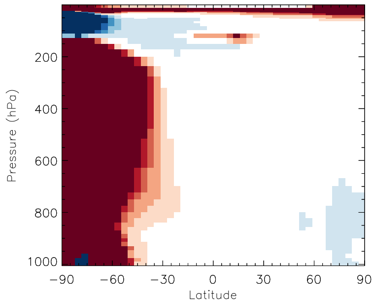
v11-01b-Run0 / v10-01i-geosfp-Run0 HN03 - Zonal mean % diff for Jul
