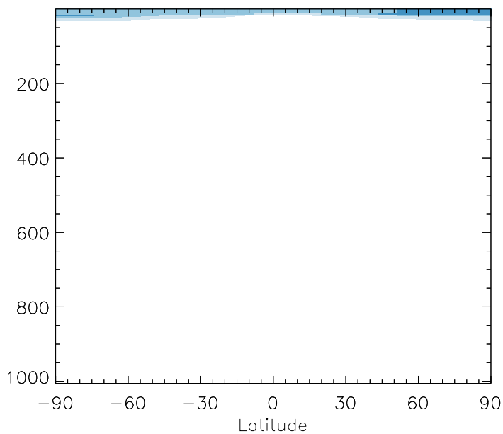
v11-01b-Run0 / v10-01i-geosfp-Run0 HCFC22 - Zonal mean % diff for Jul
