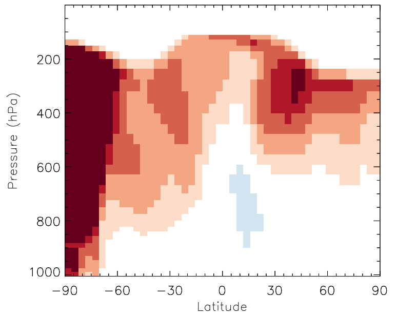
v11-01b-Run0 / v10-01-public-Run0 HBr - Zonal mean % diff for Jul
