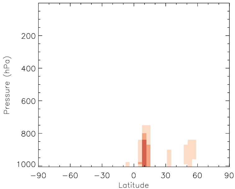
v11-01b-Run0 - v10-01i-geosp-Run0 IEPOX - Zonal mean abs diff for Jul
