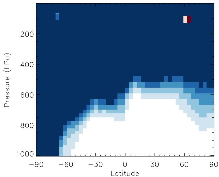
v11-01b-Run0 / v10-01-public-Run0 SO4s - Zonal mean % diff for Jul
