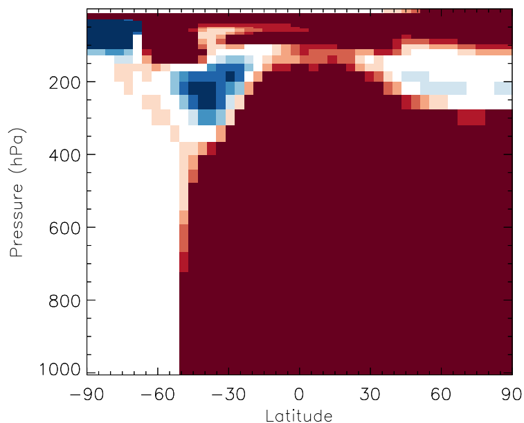
v11-01b-Run0 / v10-01i-geosfp-Run0 Cl2 - Zonal mean % diff for Jul
