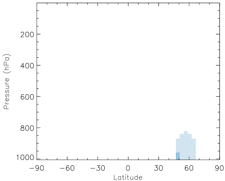
v11-01b-Run0 - v10-01i-geosfp-Run0 MEK - Zonal mean abs diff for Jul
