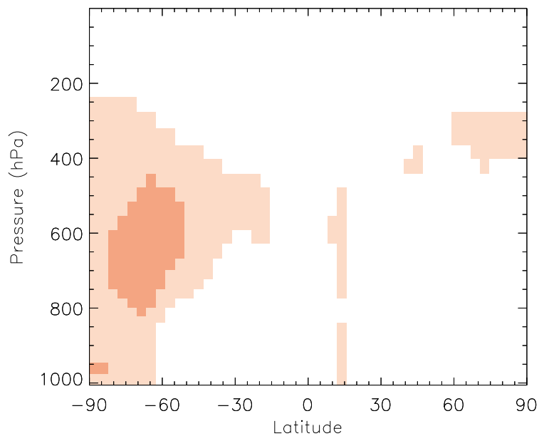
v11-01b-Run0 / v10-01-public-Run0 MPN - Zonal mean % diff for Jul
