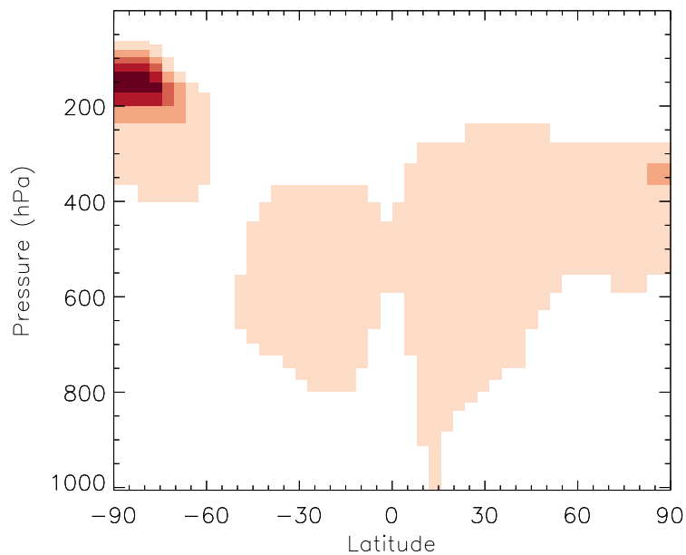
v11-01b-Run0 / v10-01-public-Run0 CIN03 - Zonal mean % diff for Jul
