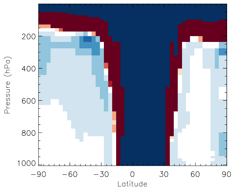
v11-01b-Run0 / v10-01i-geosp-Run0 MVK - Zonal mean % diff for Jul
