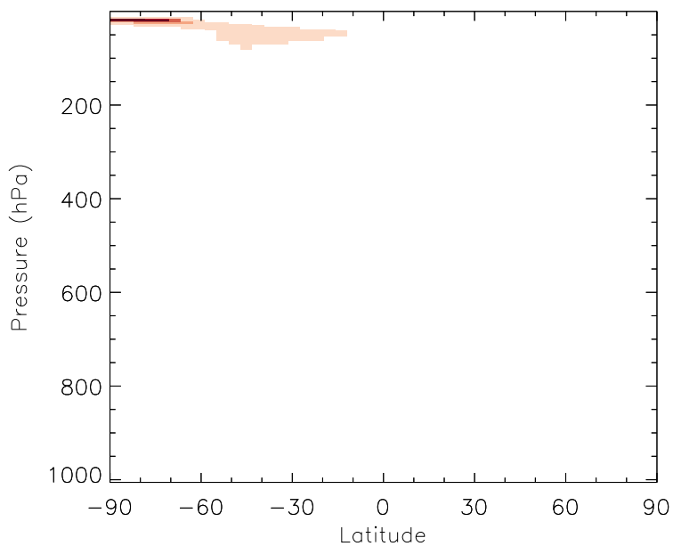
v11-01b-Run0 - v10-01i-geosp-Run0 HOBr - Zonal mean abs diff for Jul
