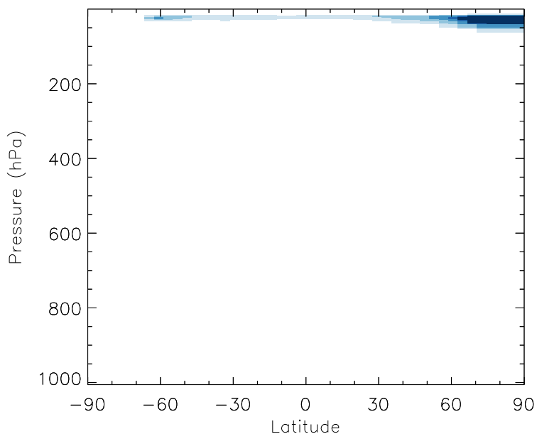
v11-01b-Run0 - v10-01i-geosp-Run0 NO - Zonal mean abs diff for Jul
