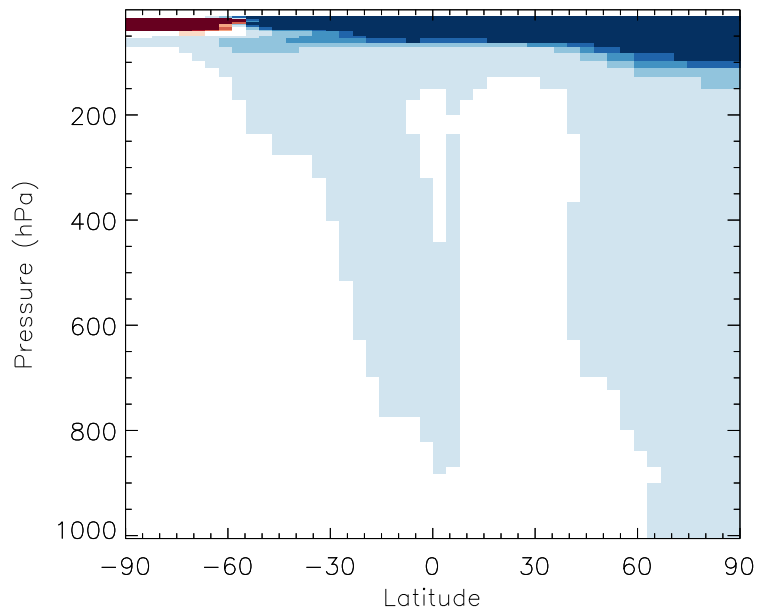
v11-01b-Run0 / v10-01i-geosfp-Run0 MEK - Zonal mean % diff for Jul
