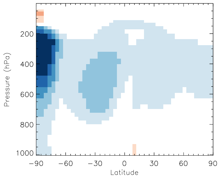
v11-01b-Run0 / v10-01-public-Run0 BrO - Zonal mean % diff for Jul
