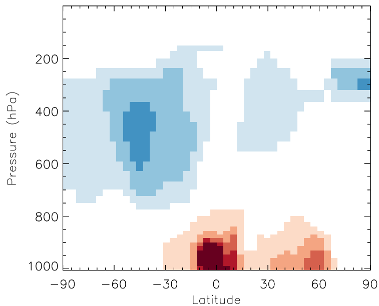
v11-01b-Run0 / v10-01-public-Run0 BrCl - Zonal mean % diff for Jul
