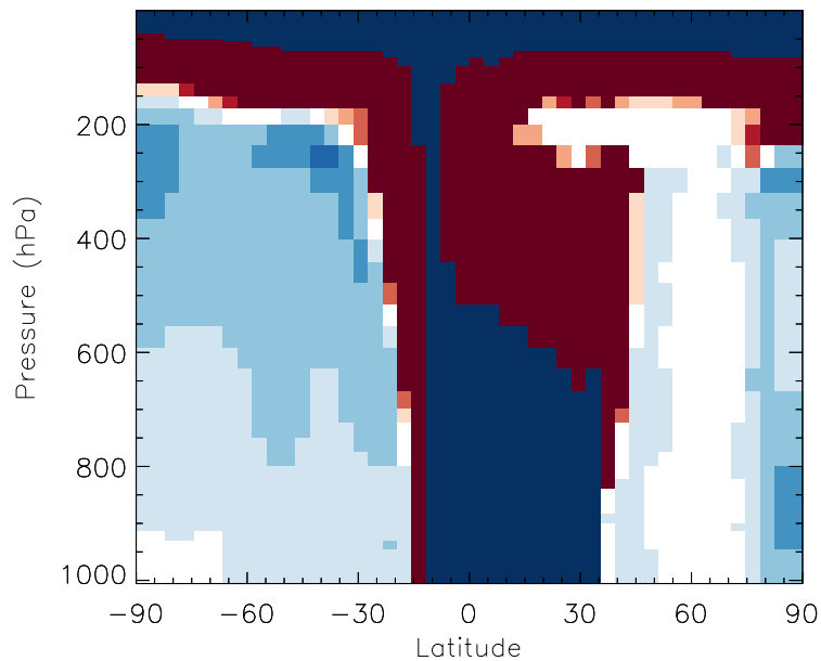
v11-01b-Run0 / v10-01i-geosfp-Run0 MACR - Zonal mean % diff for Jul
