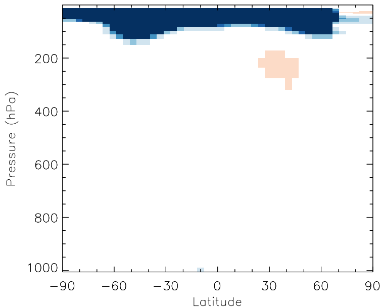
v11-01b-Run0 - v10-01i-geosfp-Run0 N2O5 - Zonal mean abs diff for Jul
