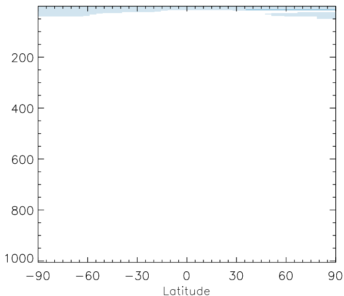
v11-01b-Run0 / v10-01i-geosfp-Run0 HCFCX - Zonal mean % diff for Jul
