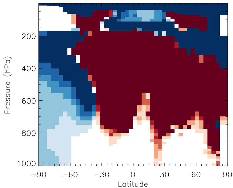
v11-01b-Run0 / v10-01-public-Run0 NIT - Zonal mean % diff for Jul
