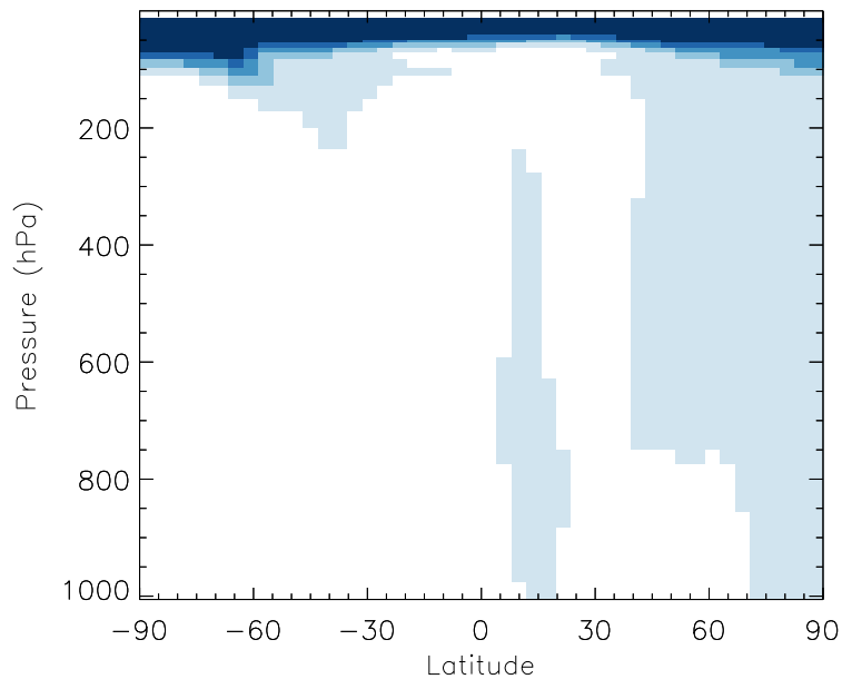
v11-01b-Run0 / v10-01i-geosp-Run0 ALD2 - Zonal mean % diff for Jul
