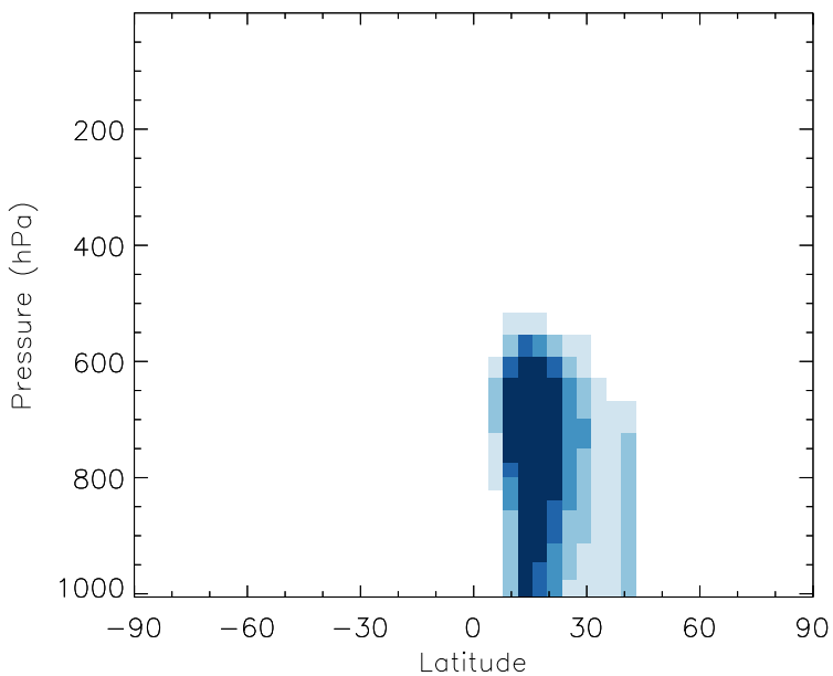
v11-01b-Run0 - v10-01-public-Run0 DST3 - Zonal mean abs diff for Jul
