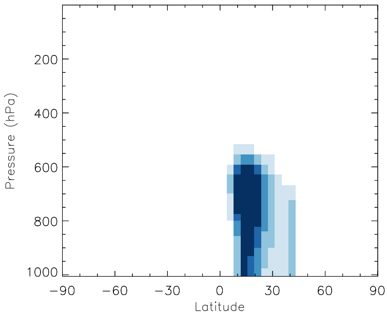
v11-01b-Run0 - v10-01i-geosfp-Run0 DST3 - Zonal mean abs diff for Jul
