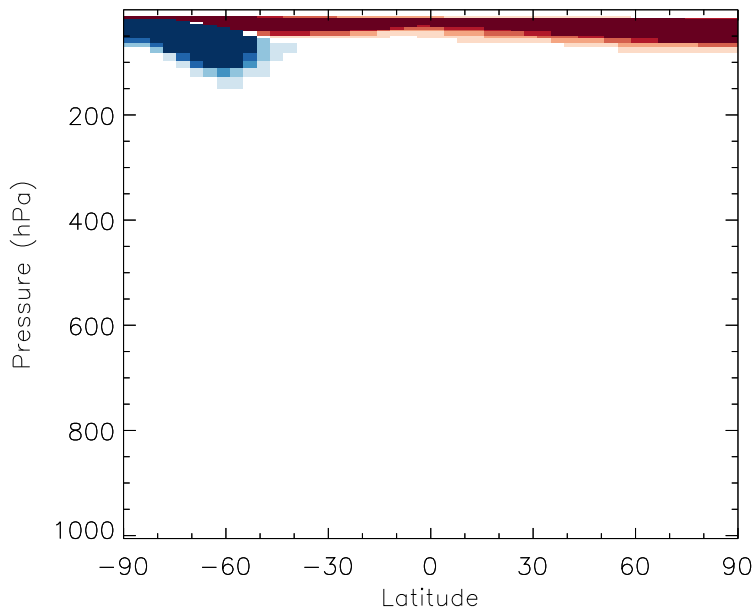
v11-01b-Run0 - v10-01i-geosfp-Run0 CIN03 - Zonal mean abs diff for Jul
