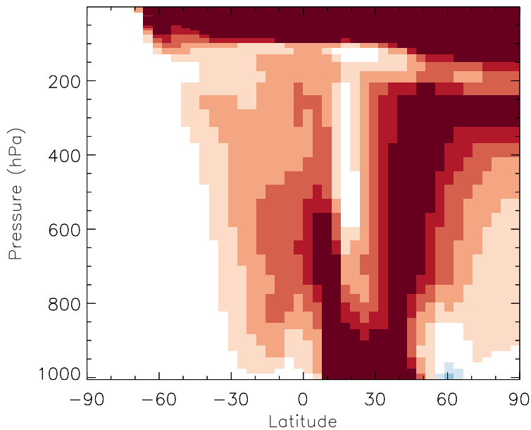
v11-01b-Run0 - v10-01i-geosp-Run0 OH - Zonal mean abs diff for Jul
