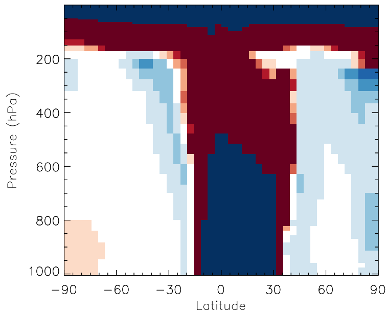
v11-01b-Run0 / v10-01i-geosfp-Run0 PMN - Zonal mean % diff for Jul
