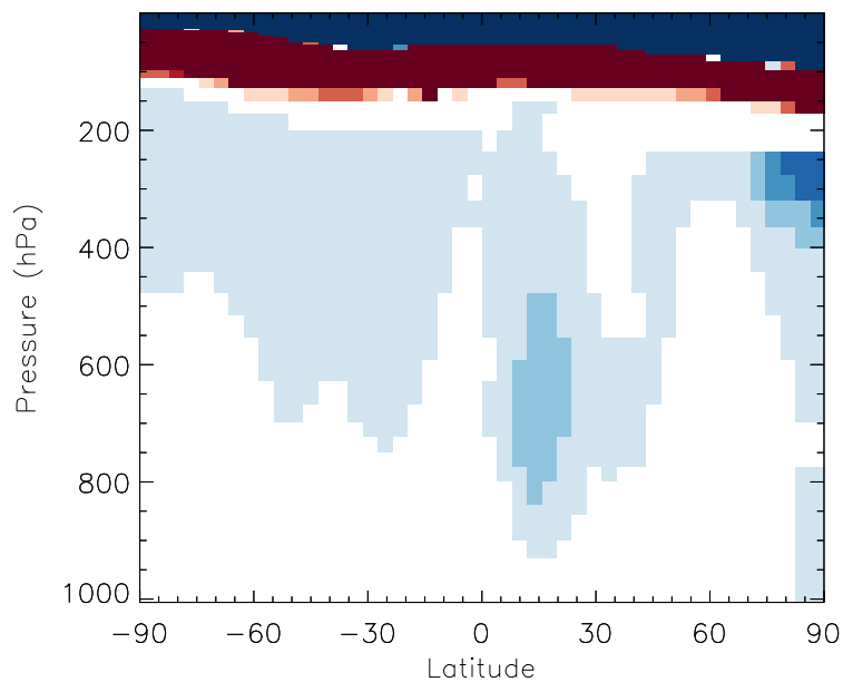
v11-01b-Run0 / v10-01-public-Run0 PRPE - Zonal mean % diff for Jul
