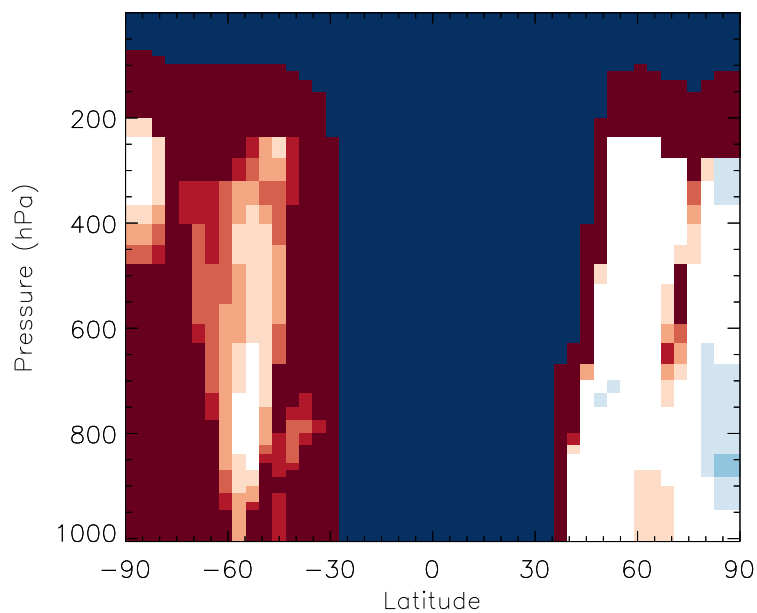
v11-01b-Run0 / v10-01i-geosp-Run0 MOBA - Zonal mean % diff for Jul
