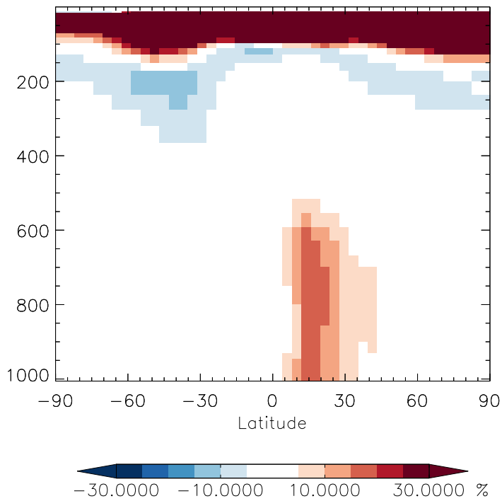
v11-01b-Run0 / v10-01i-geosp-Run0 MP - Zonal mean % diff for Jul
