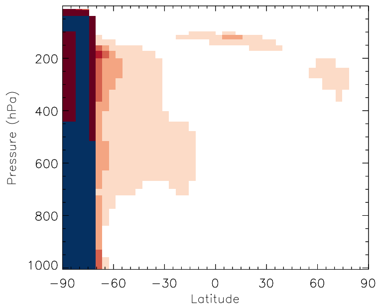
v11-01b-Run0 / v10-01-public-Run0 NO - Zonal mean % diff for Jul
