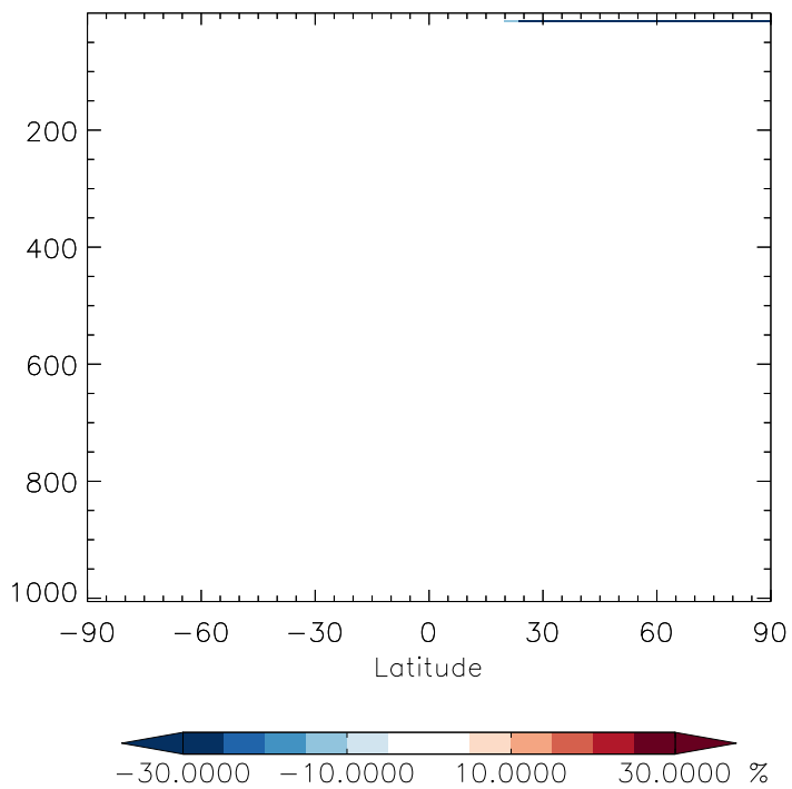
v11-01b-Run0 / v10-01-public-Run0 CH3Br - Zonal mean % diff for Jul
