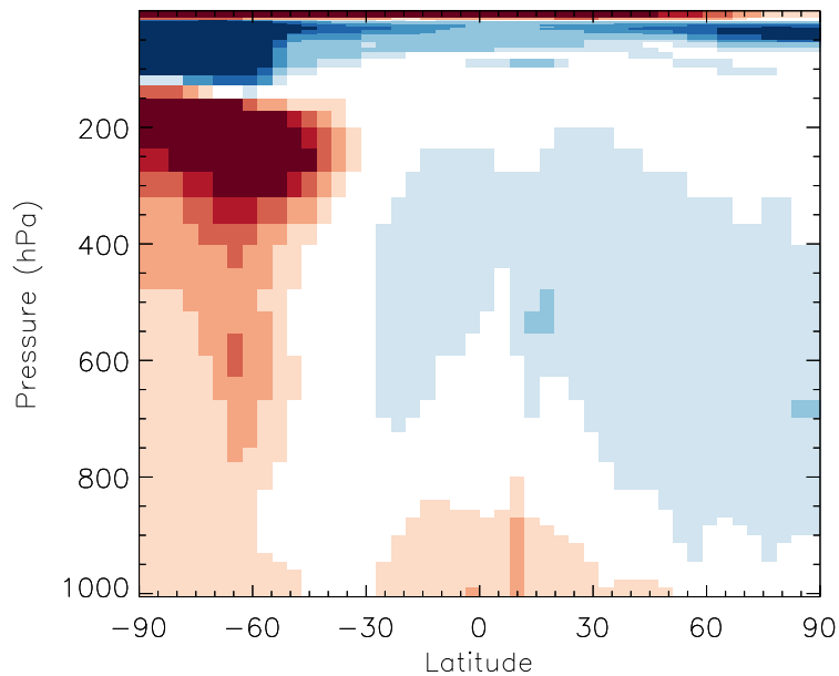
v11-01b-Run0 / v10-01i-geosfp-Run0 BrNO2 - Zonal mean % diff for Jul
