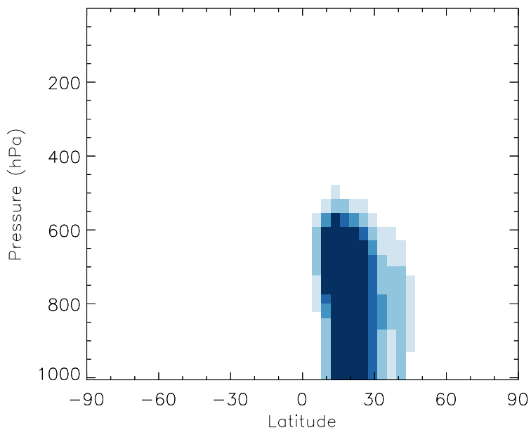
v11-01b-Run0 - v10-01-public-Run0 DST2 - Zonal mean abs diff for Jul
