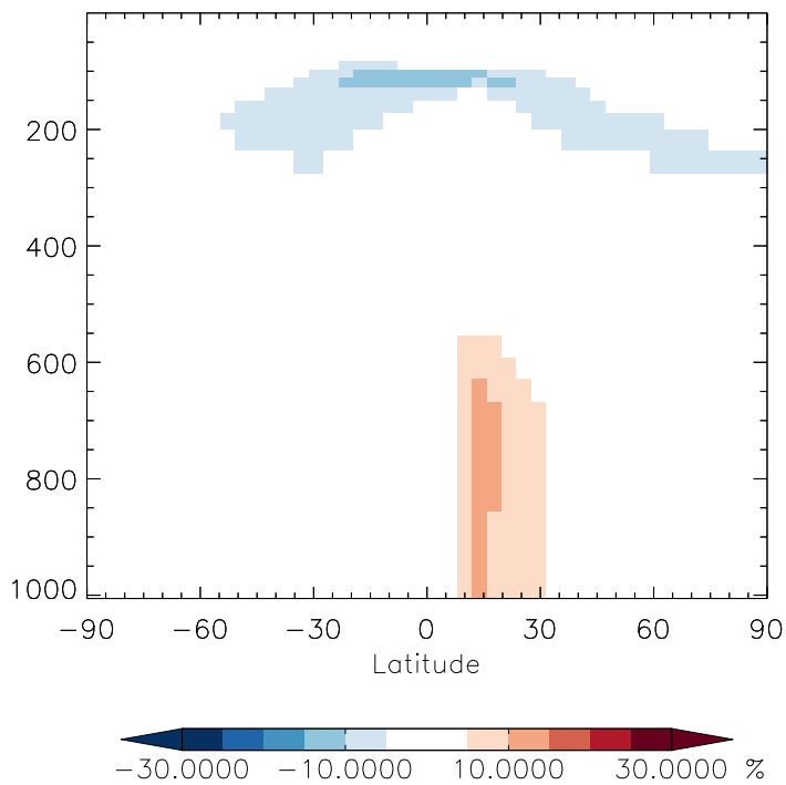
v11-01b-Run0 / v10-01-public-Run0 MP - Zonal mean % diff for Jul
