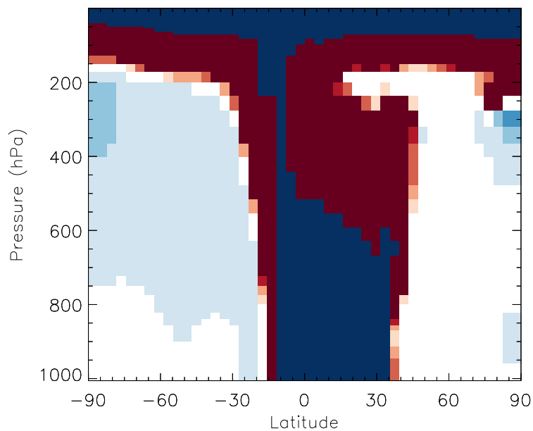
v11-01b-Run0 / v10-01-public-Run0 MACR - Zonal mean % diff for Jul
