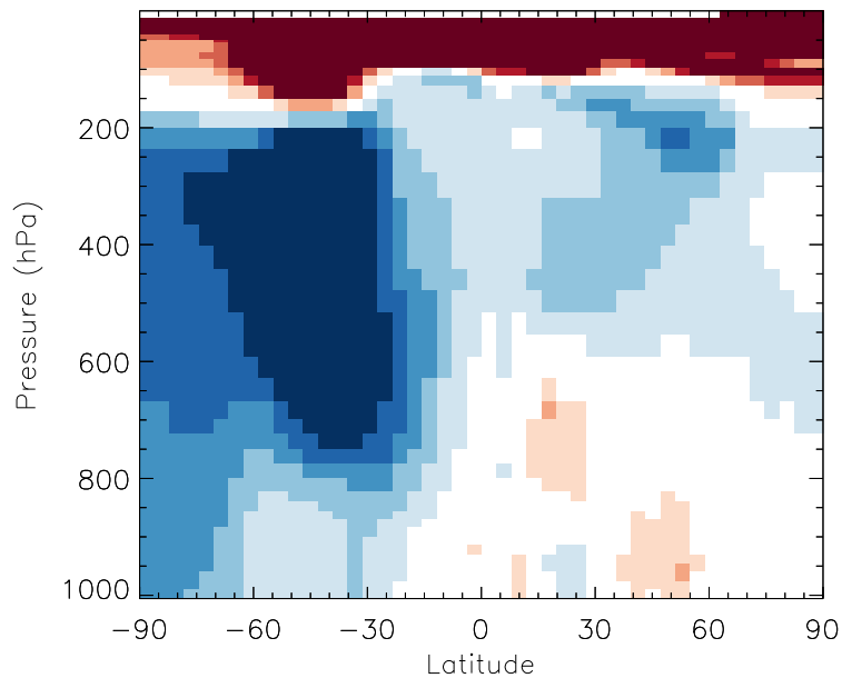
v11-01b-Run0 / v10-01i-geosfp-Run0 OCIO - Zonal mean % diff for Jul
