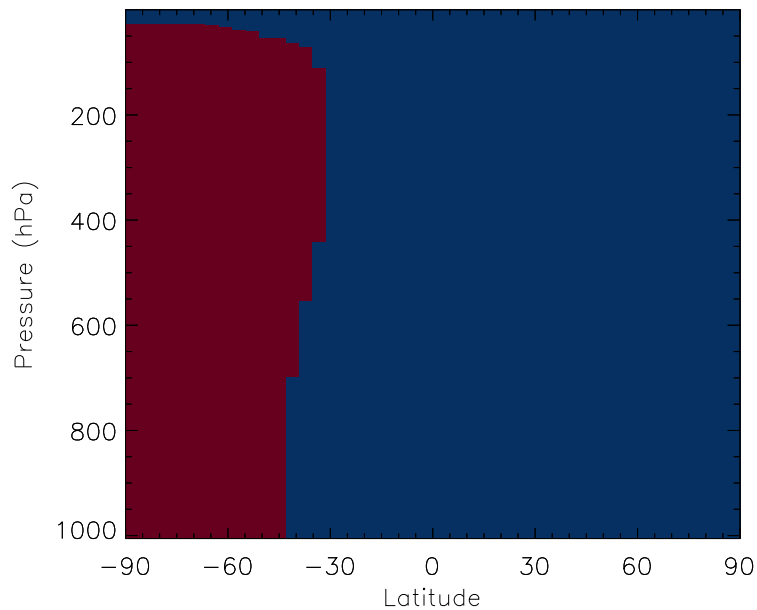
v11-01b-Run0 / v10-01i-geosfp-Run0 CIN02 - Zonal mean % diff for Jul
