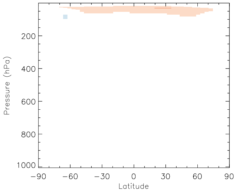
v11-01b-Run0 - v10-01i-geosfp-Run0 MPN - Zonal mean abs diff for Jul
