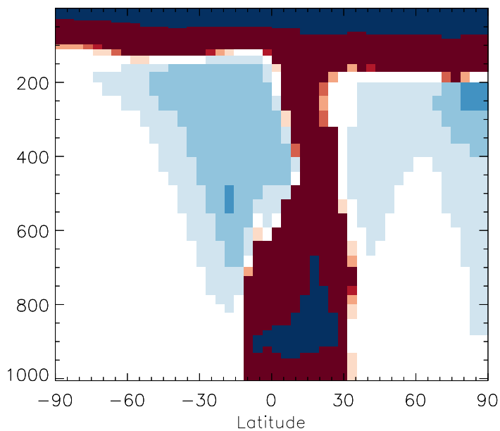
v11-01b-Run0 / v10-01-public-Run0 IEPOX - Zonal mean % diff for Jul
