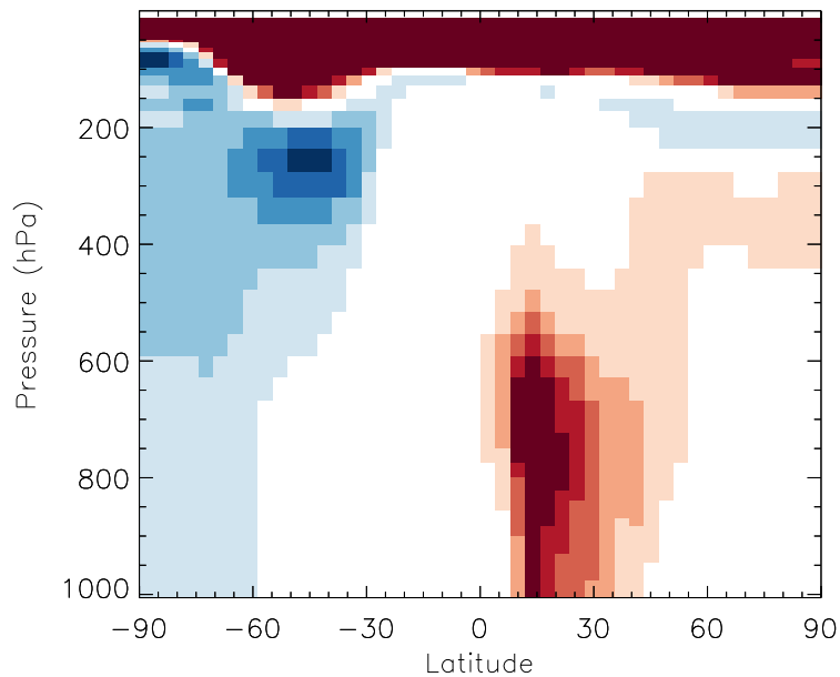
v11-01b-Run0 / v10-01i-geosfp-Run0 HOCl - Zonal mean % diff for Jul
