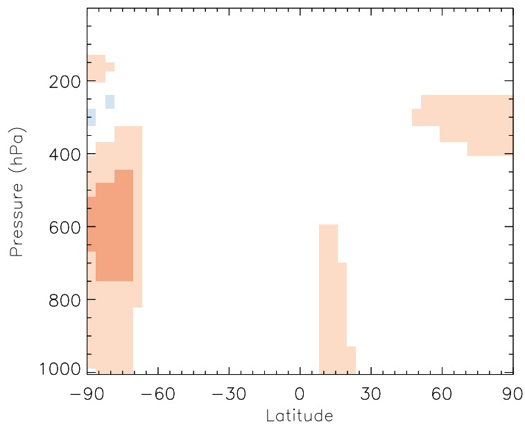
v11-01b-Run0 / v10-01-public-Run0 OH - Zonal mean % diff for Jul
