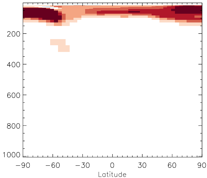
v11-01b-Run0 / v10-01i-geosp-Run0 CH2O - Zonal mean % diff for Jul
