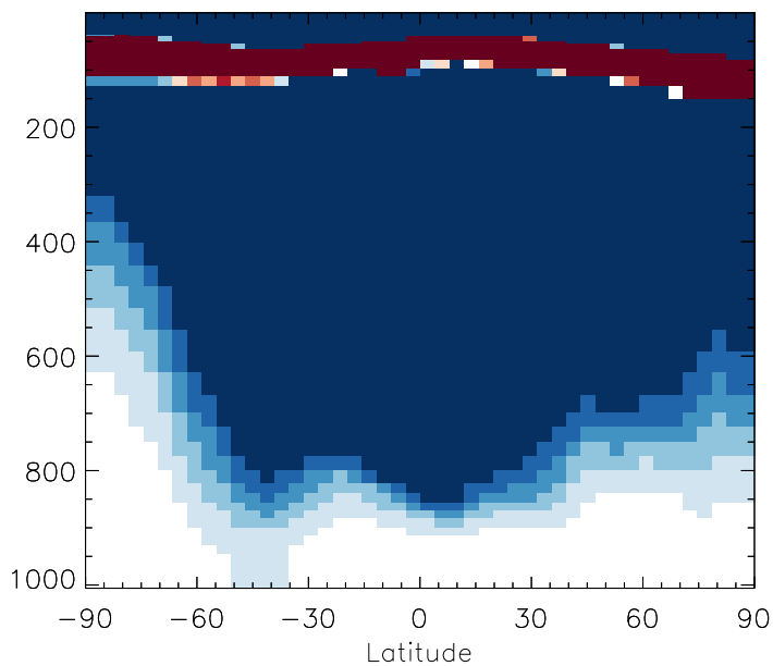
v11-01b-Run0 / v10-01-public-Run0 BCPO - Zonal mean % diff for Jul
