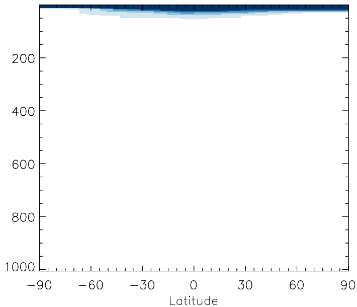
v11-01b-Run0 / v10-01i-geosfp-Run0 H1211 - Zonal mean % diff for Jul
