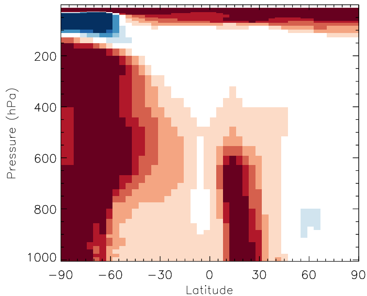
v11-01b-Run0 / v10-01i-geosfp-Run0 HN04 - Zonal mean % diff for Jul
