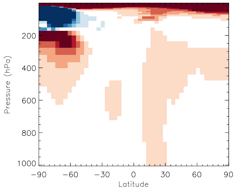
v11-01b-Run0 / v10-01i-geosfp-Run0 CIN03 - Zonal mean % diff for Jul
