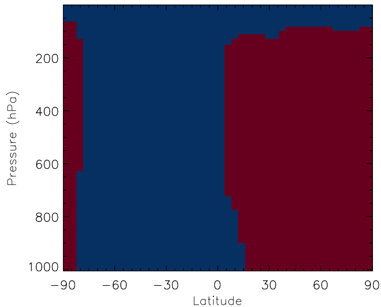
v11-01b-Run0 / v10-01i-geosfp-Run0 DST4 - Zonal mean % diff for Jul
