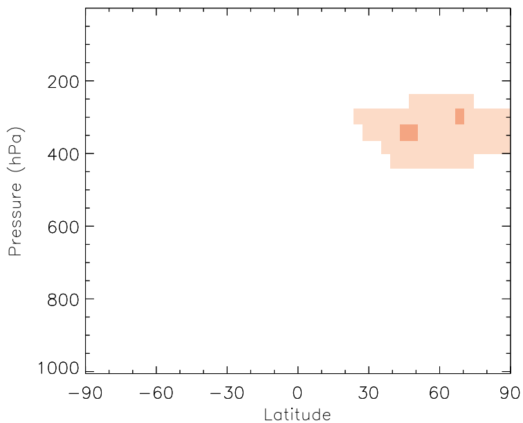
v11-01b-Run0 - v10-01-public-Run0 HN04 - Zonal mean abs diff for Jul
