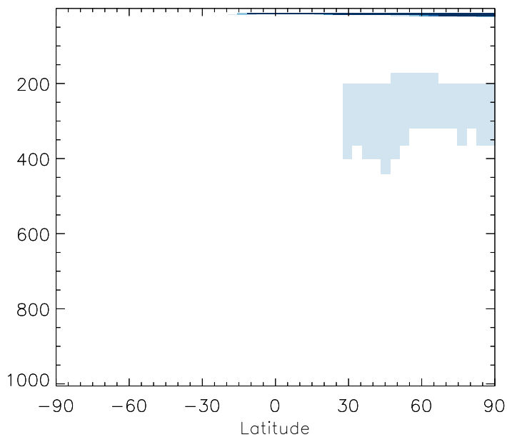
v11-01b-Run0 / v10-01-public-Run0 R4N2 - Zonal mean % diff for Jul
