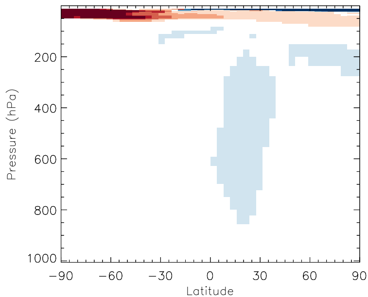
v11-01b-Run0 / v10-01-public-Run0 MEK - Zonal mean % diff for Jul
