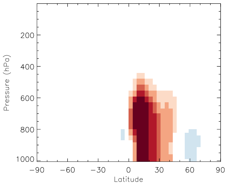
v11-01b-Run0 - v10-01-public-Run0 H2O2 - Zonal mean abs diff for Jul
