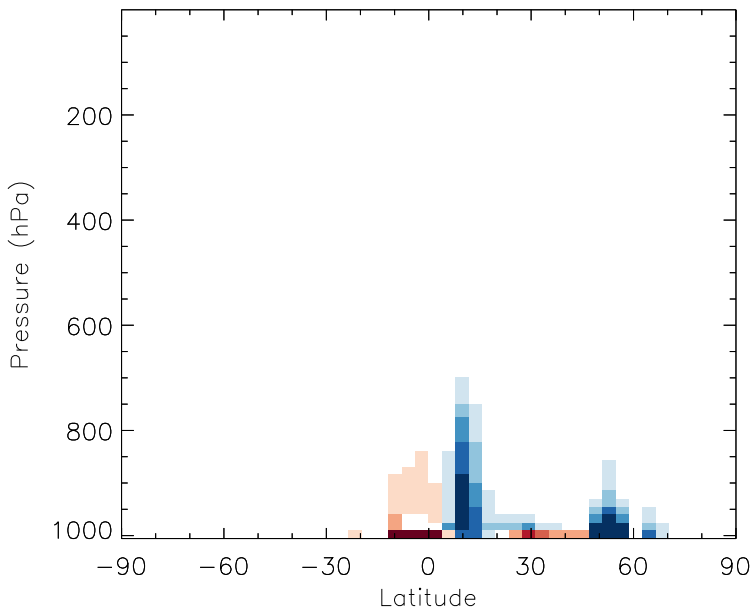
v11-01b-Run0 - v10-01i-geosp-Run0 PRPE - Zonal mean abs diff for Jul
