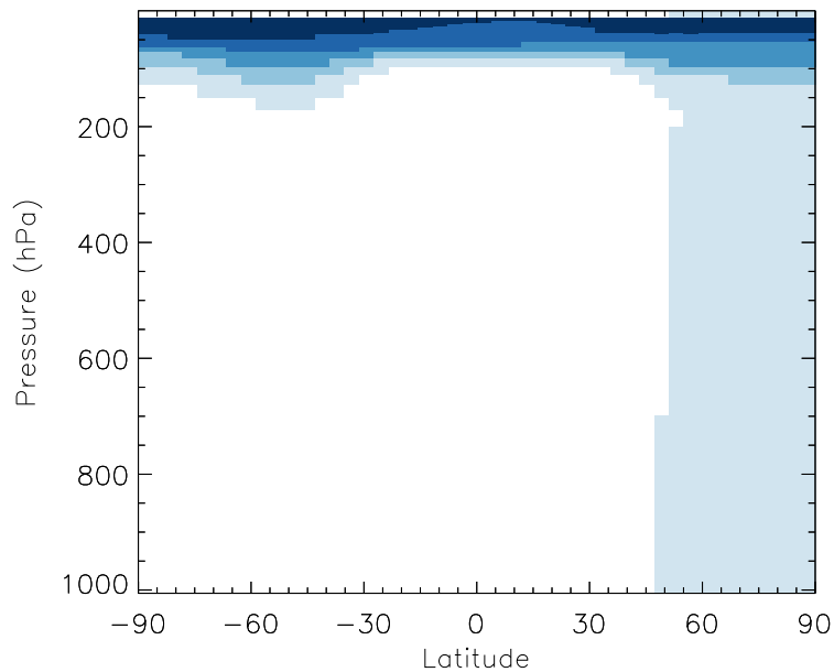
v11-01b-Run0 / v10-01i-geosfp-Run0 CO - Zonal mean % diff for Jul
