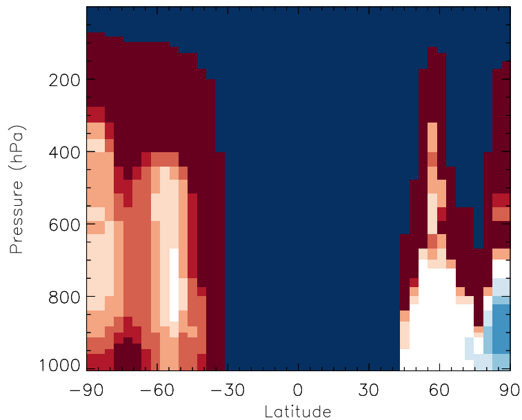
v11-01b-Run0 / v10-01i-geosp-Run0 ISOP - Zonal mean % diff for Jul
