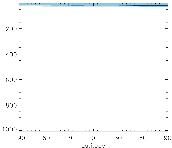
v11-01b-Run0 / v10-01i-geosfp-Run0 OCS - Zonal mean % diff for Jul
