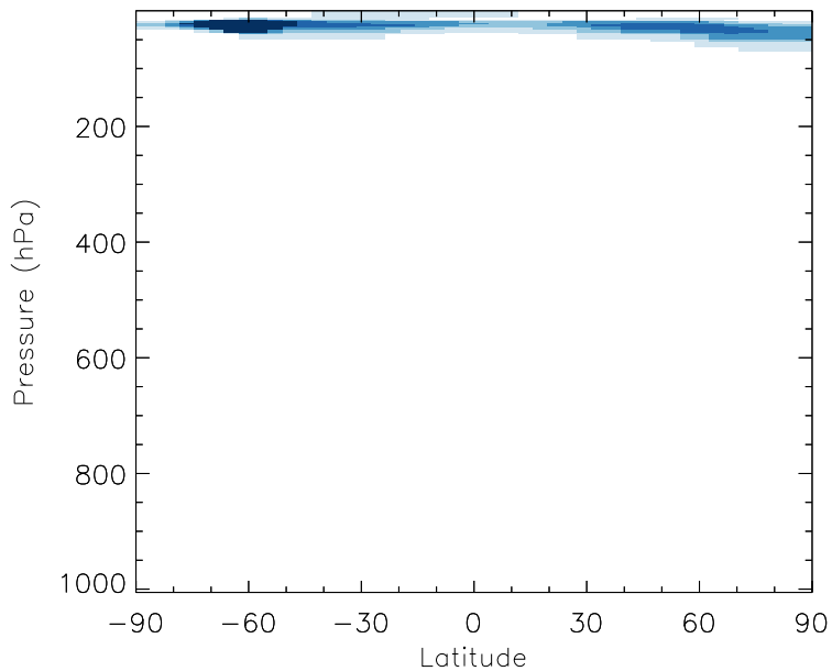
v11-01b-Run0 - v10-01i-geosfp-Run0 NO2 - Zonal mean abs diff for Jul
