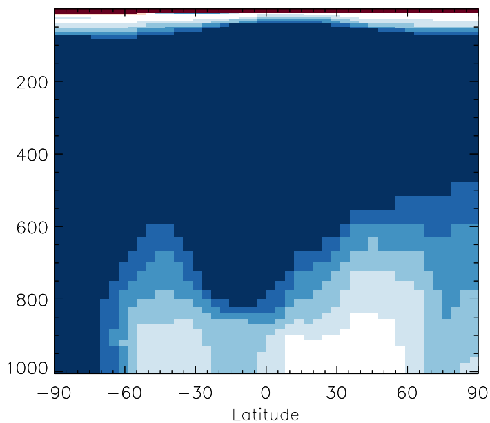
v11-01b-Run0 / v10-01i-geosp-Run0 BCPI - Zonal mean % diff for Jul
