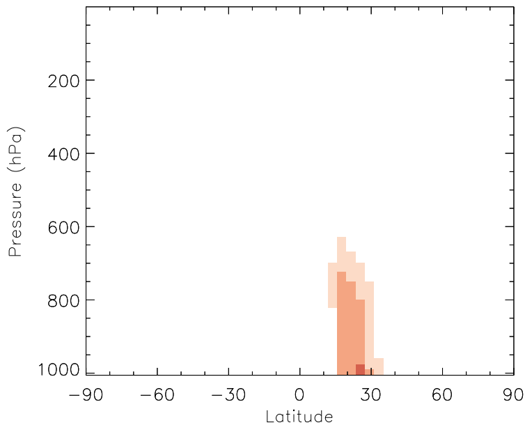
v11-01b-Run0 - v10-01i-geosfp-Run0 DST4 - Zonal mean abs diff for Jul
