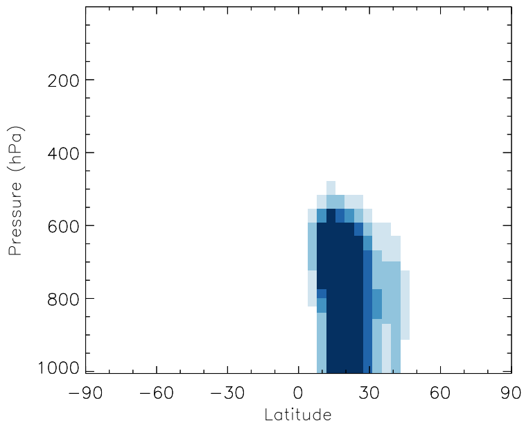
v11-01b-Run0 - v10-01i-geosfp-Run0 DST2 - Zonal mean abs diff for Jul
