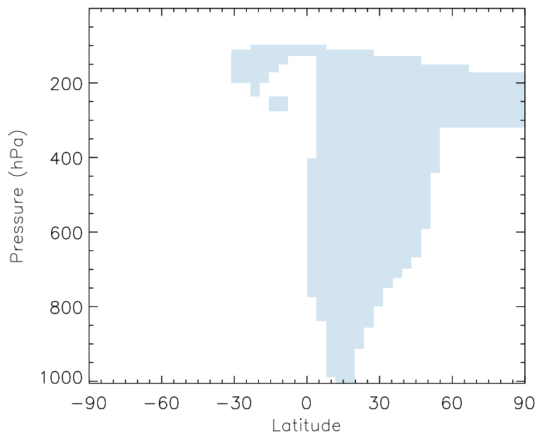
v11-01b-Run0 / v10-01-public-Run0 ALD2 - Zonal mean % diff for Jul
