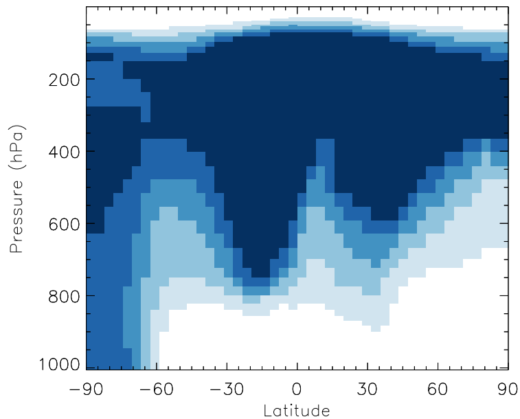
v11-01b-Run0 / v10-01i-geosfp-Run0 MSA - Zonal mean % diff for Jul
