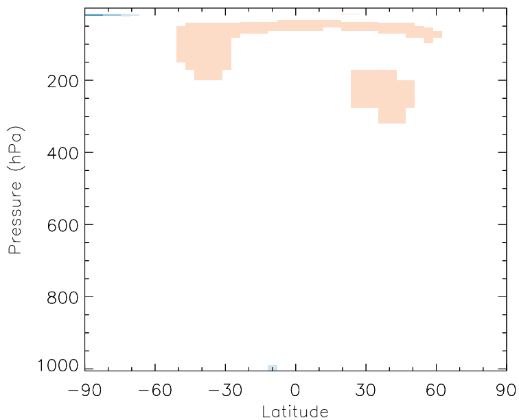
v11-01b-Run0 - v10-01-public-Run0 N2O5 - Zonal mean abs diff for Jul
