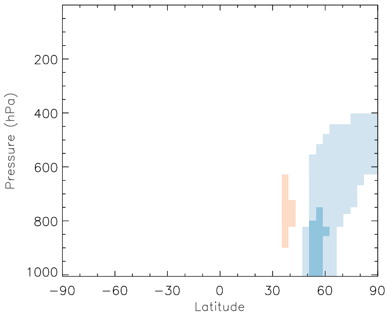
v11-01b-Run0 - v10-01i-geosfp-Run0 PPN - Zonal mean abs diff for Jul
