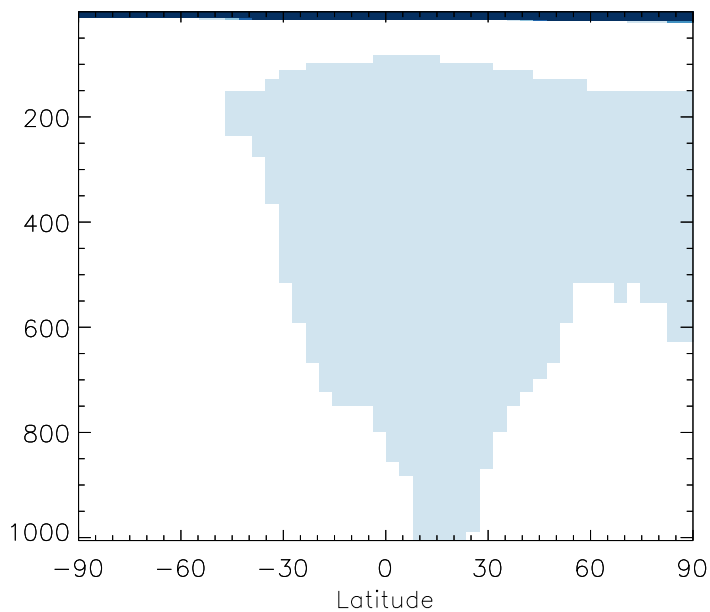
v11-01b-Run0 / v10-01-public-Run0 C3H8 - Zonal mean % diff for Jul
