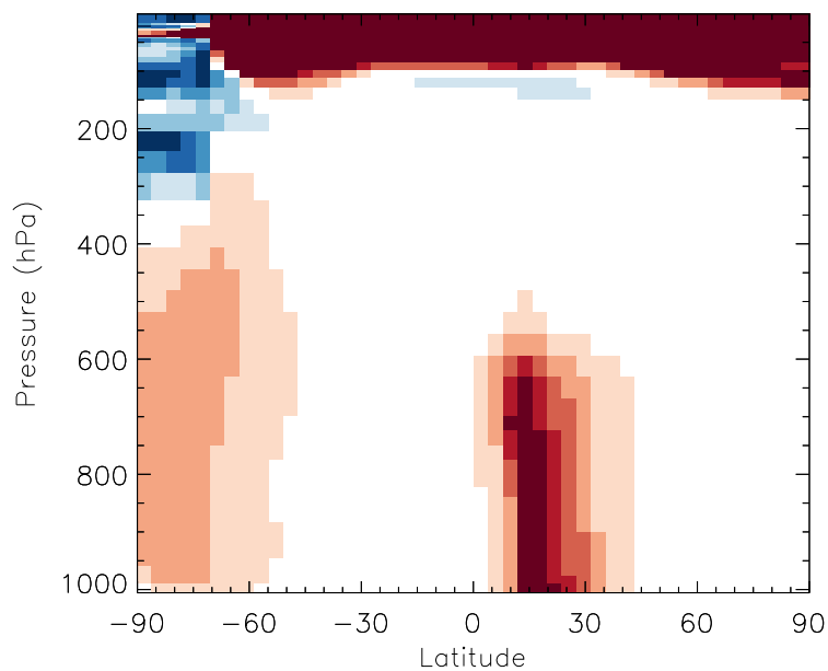
v11-01b-Run0 / v10-01i-geosfp-Run0 HO2 - Zonal mean % diff for Jul
