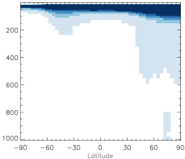
v11-01b-Run0 / v10-01i-geosp-Run0 R4N2 - Zonal mean % diff for Jul
