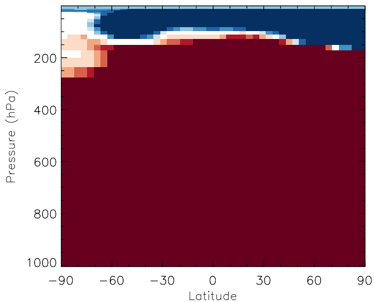
v11-01b-Run0 - v10-01-public-Run0 H2O - Zonal mean abs diff for Jul
