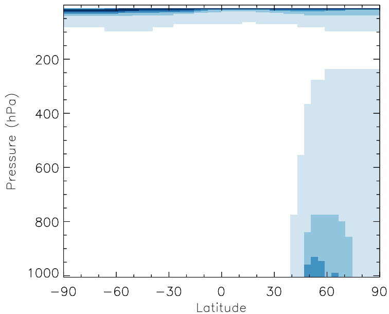
v11-01b-Run0 - v10-01i-geosfp-Run0 CO - Zonal mean abs diff for Jul
