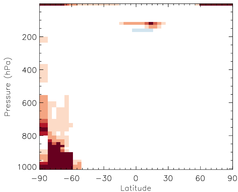
v11-01b-Run0 / v10-01-public-Run0 HN03 - Zonal mean % diff for Jul
