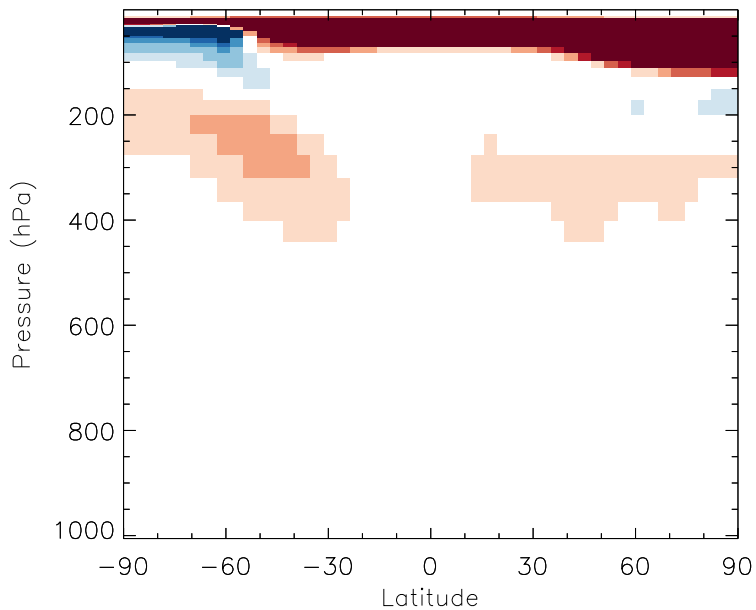
v11-01b-Run0 - v10-01i-geosfp-Run0 HN04 - Zonal mean abs diff for Jul
