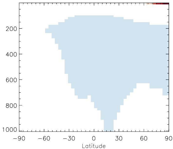
v11-01b-Run0 / v10-01-public-Run0 C2H6 - Zonal mean % diff for Jul
