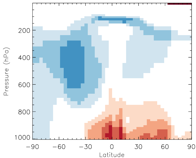
v11-01b-Run0 / v10-01-public-Run0 OCIO - Zonal mean % diff for Jul
