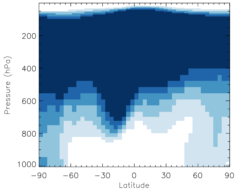
v11-01b-Run0 / v10-01i-geosp-Run0 NH4 - Zonal mean % diff for Jul
