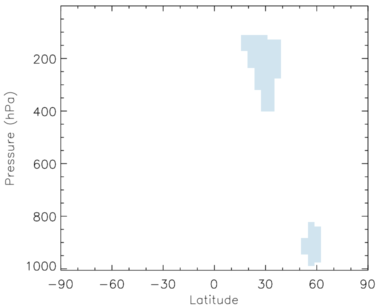
v11-01b-Run0 - v10-01-public-Run0 PPN - Zonal mean abs diff for Jul
