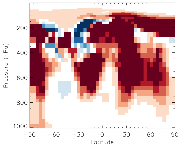
v11-01b-Run0 / v10-01-public-Run0 NH3 - Zonal mean % diff for Jul
