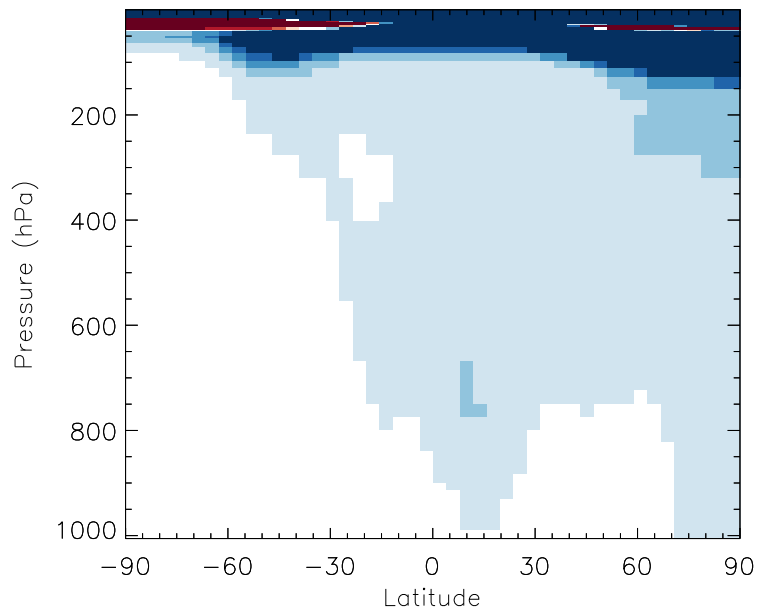
v11-01b-Run0 / v10-01i-geosp-Run0 ALK4 - Zonal mean % diff for Jul
