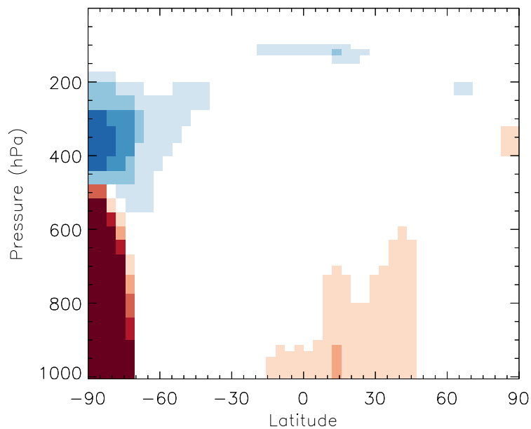
v11-01b-Run0 / v10-01-public-Run0 ClO - Zonal mean % diff for Jul
