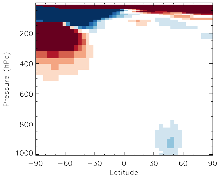
v11-01b-Run0 - v10-01i-geosfp-Run0 HN03 - Zonal mean abs diff for Jul
