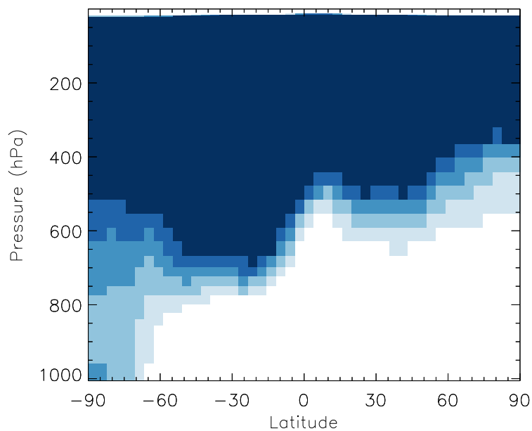
v11-01b-Run0 / v10-01i-geosp-Run0 SALA - Zonal mean % diff for Jul
