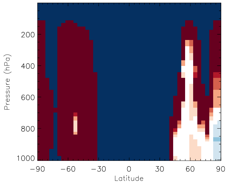
v11-01b-Run0 / v10-01i-geosfp-Run0 ISOPN - Zonal mean % diff for Jul
