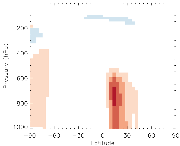
v11-01b-Run0 / v10-01-public-Run0 HO2 - Zonal mean % diff for Jul
