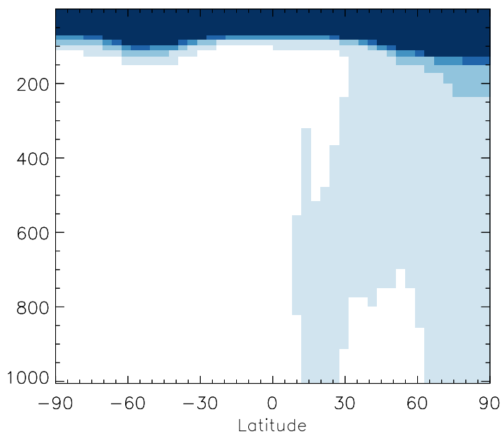
v11-01b-Run0 / v10-01i-geosp-Run0 C3H8 - Zonal mean % diff for Jul
