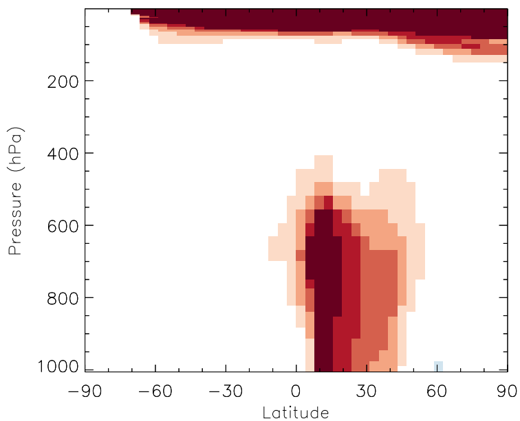
v11-01b-Run0 - v10-01i-geosfp-Run0 HO2 - Zonal mean abs diff for Jul
