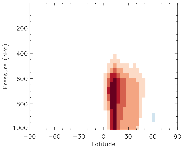
v11-01b-Run0 - v10-01-public-Run0 HO2 - Zonal mean abs diff for Jul
