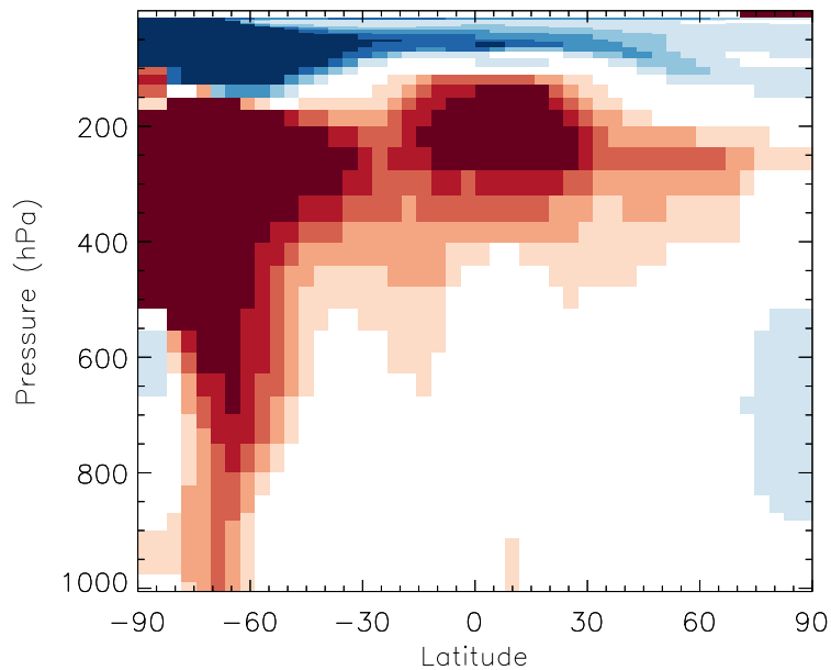
v11-01b-Run0 / v10-01i-geosfp-Run0 BrNO3 - Zonal mean % diff for Jul
