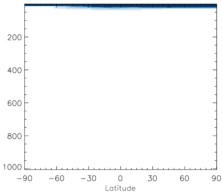
v11-01b-Run0 / v10-01i-geosfp-Run0 CCl4 - Zonal mean % diff for Jul
