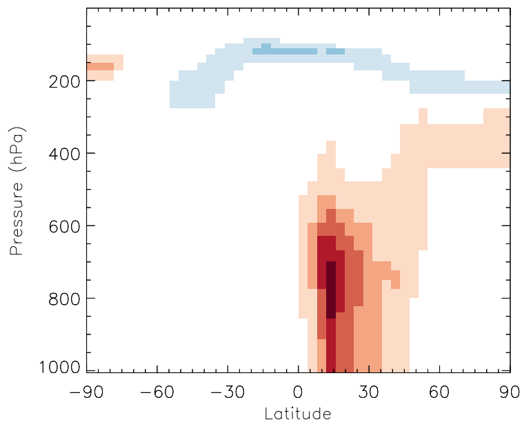
v11-01b-Run0 / v10-01-public-Run0 HOCl - Zonal mean % diff for Jul
