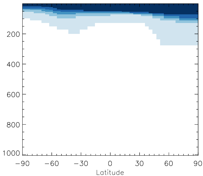
v11-01b-Run0 / v10-01i-geosfp-Run0 CHBr3 - Zonal mean % diff for Jul
