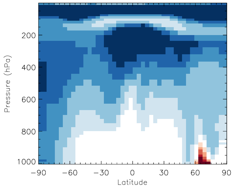
v11-01b-Run0 / v10-01i-geosp-Run0 SO2 - Zonal mean % diff for Jul
