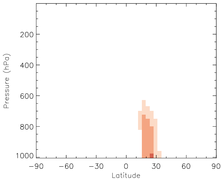
v11-01b-Run0 - v10-01-public-Run0 DST4 - Zonal mean abs diff for Jul
