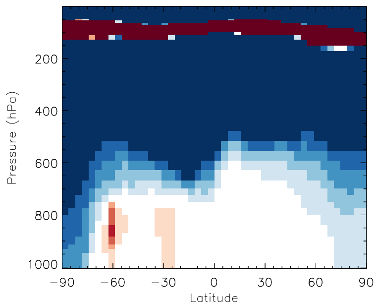
v11-01b-Run0 / v10-01i-geosfp-Run0 NITs - Zonal mean % diff for Jul
