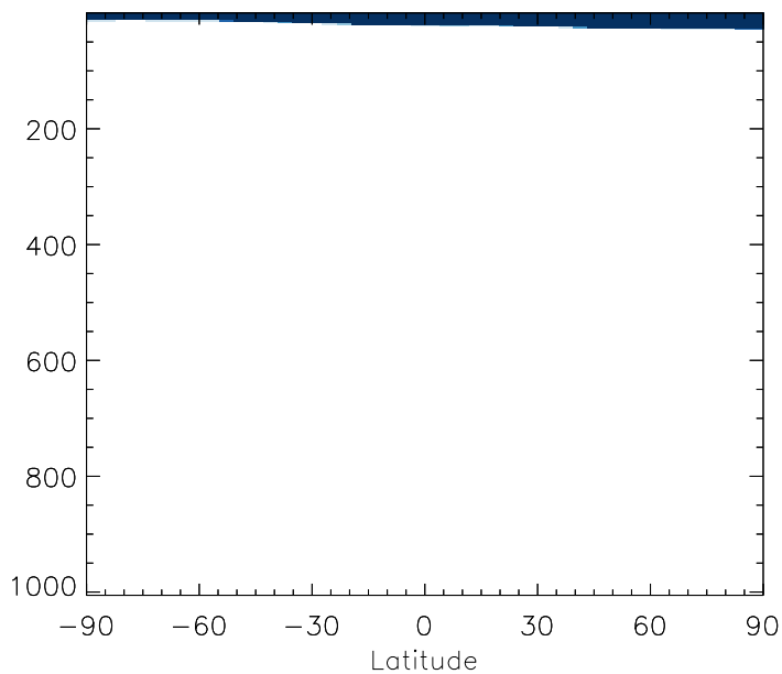
v11-01b-Run0 / v10-01-public-Run0 CHBr3 - Zonal mean % diff for Jul
