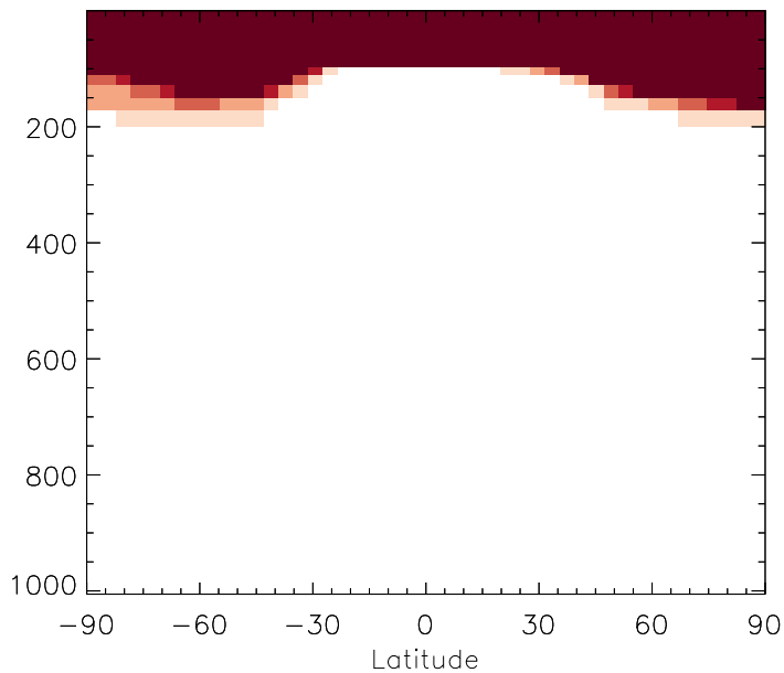
v11-01b-Run0 / v10-01i-geosfp-Run0 H2O - Zonal mean % diff for Jul
