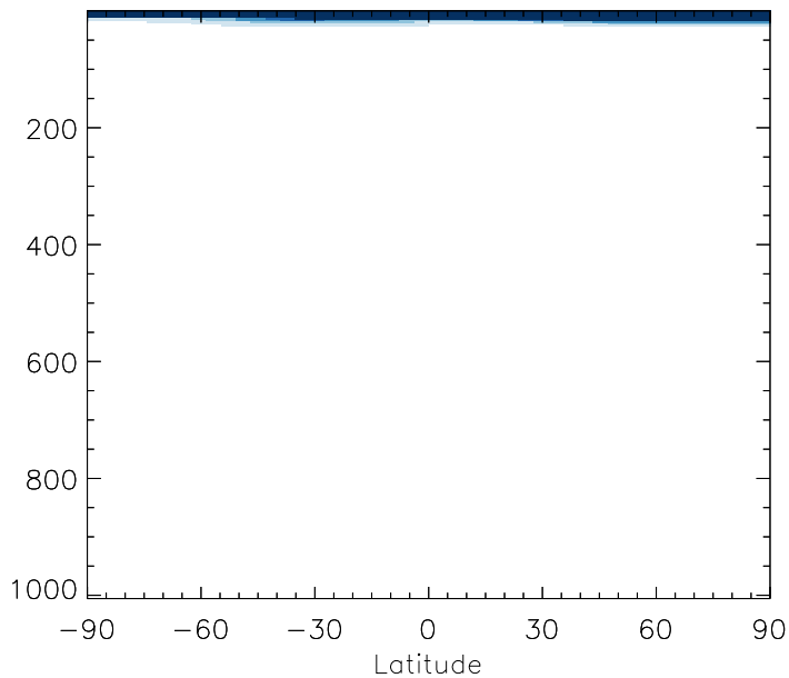
v11-01b-Run0 / v10-01i-geosfp-Run0 H1301 - Zonal mean % diff for Jul
