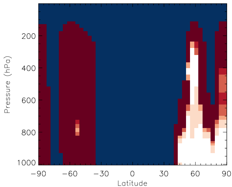
v11-01b-Run0 / v10-01-public-Run0 ISOPN - Zonal mean % diff for Jul
