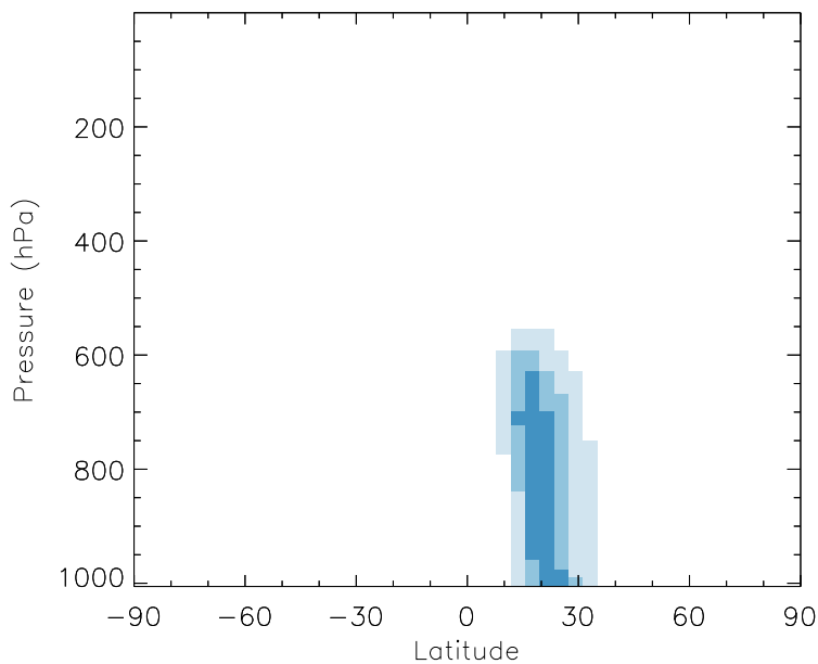
v11-01b-Run0 - v10-01-public-Run0 DST1 - Zonal mean abs diff for Jul
