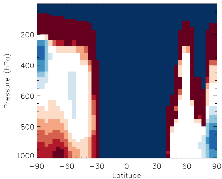
v11-01b-Run0 / v10-01i-geosfp-Run0 RIP - Zonal mean % diff for Jul
