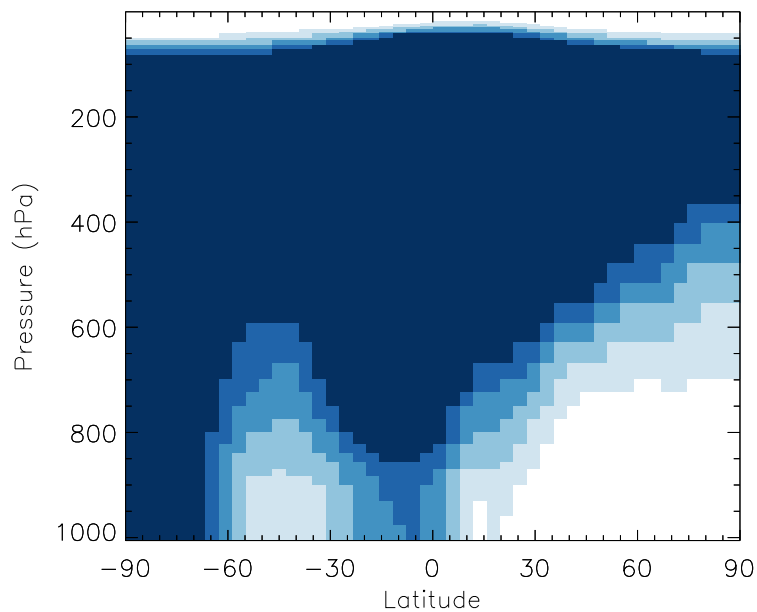
v11-01b-Run0 / v10-01-public-Run0 OCPI - Zonal mean % diff for Jul
