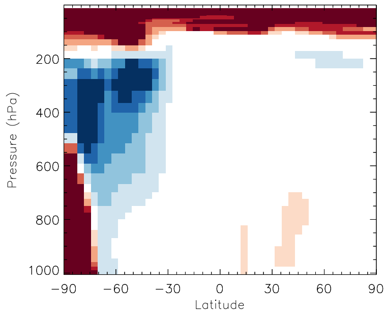
v11-01b-Run0 / v10-01i-geosfp-Run0 ClO - Zonal mean % diff for Jul
