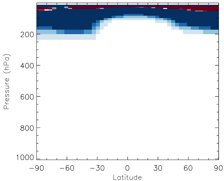
v11-01b-Run0 - v10-01i-geosfp-Run0 O3 - Zonal mean abs diff for Jul
