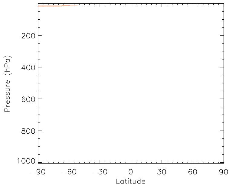
v11-01b-Run0 / v10-01-public-Run0 PAN - Zonal mean % diff for Jul
