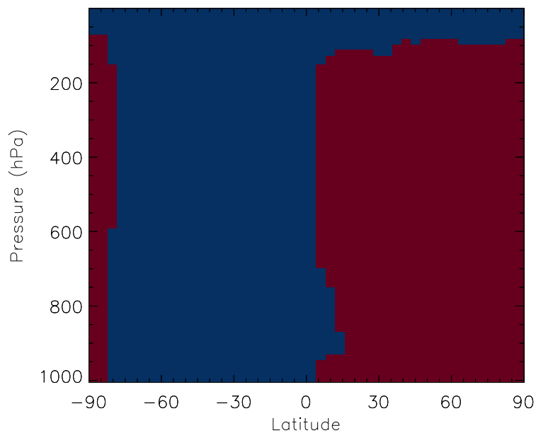
v11-01b-Run0 / v10-01-public-Run0 DST4 - Zonal mean % diff for Jul
