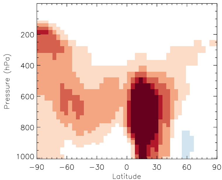
v11-01b-Run0 / v10-01-public-Run0 NO3 - Zonal mean % diff for Jul
