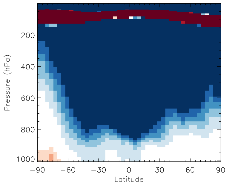
v11-01b-Run0 / v10-01-public-Run0 OCPO - Zonal mean % diff for Jul
