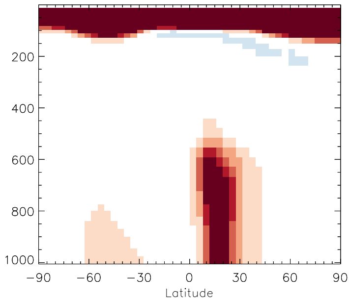
v11-01b-Run0 / v10-01i-geosfp-Run0 H2O2 - Zonal mean % diff for Jul
