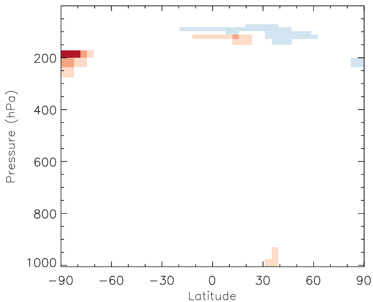
v11-01b-Run0 - v10-01-public-Run0 HN03 - Zonal mean abs diff for Jul
