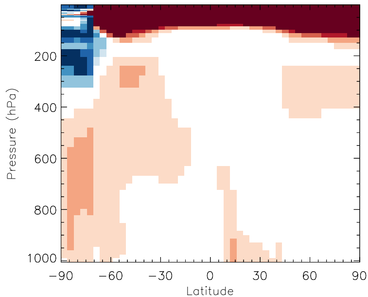
v11-01b-Run0 / v10-01i-geosp-Run0 OH - Zonal mean % diff for Jul
