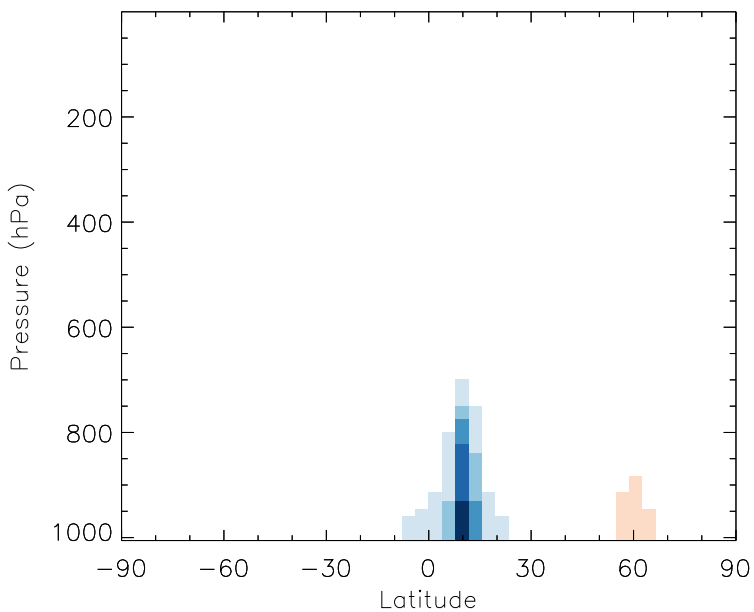
v11-01b-Run0 - v10-01-public-Run0 PRPE - Zonal mean abs diff for Jul
