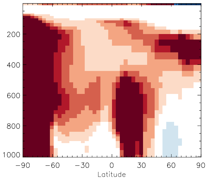
v11-01b-Run0 / v10-01-public-Run0 N2O5 - Zonal mean % diff for Jul
