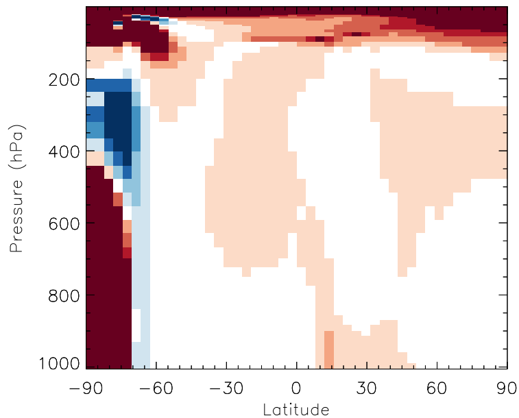
v11-01b-Run0 / v10-01i-geosfp-Run0 ClOO - Zonal mean % diff for Jul
