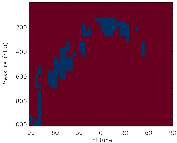
v11-01b-Run0 - v10-01i-geosfp-Run0 H2O - Zonal mean abs diff for Jul
