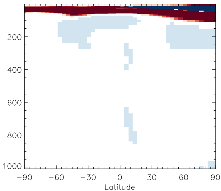
v11-01b-Run0 / v10-01i-geosfp-Run0 PROPNN - Zonal mean % diff for Jul
