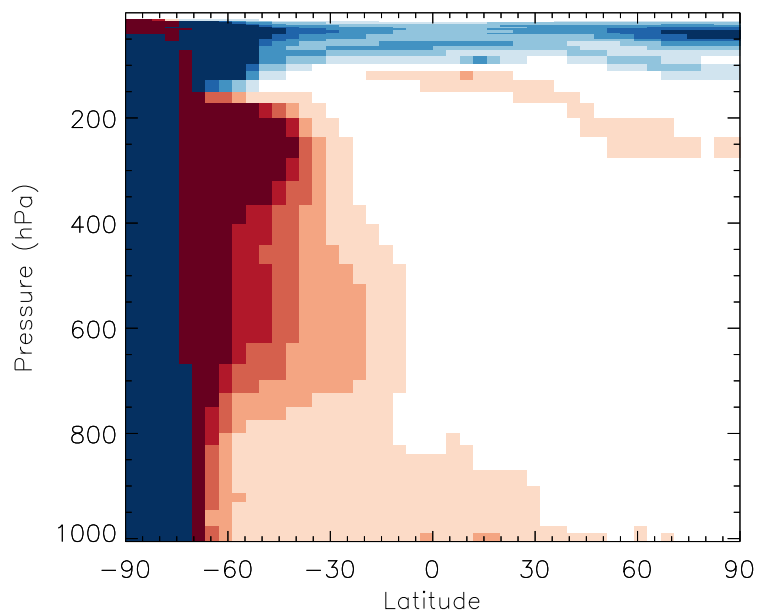
v11-01b-Run0 / v10-01i-geosp-Run0 NO - Zonal mean % diff for Jul
