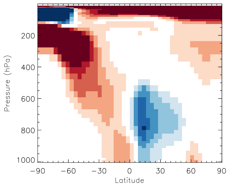
v11-01b-Run0 / v10-01i-geosfp-Run0 HN02 - Zonal mean % diff for Jul
