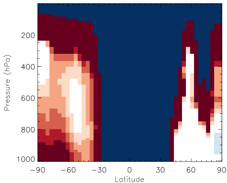
v11-01b-Run0 / v10-01-public-Run0 RIP - Zonal mean % diff for Jul
