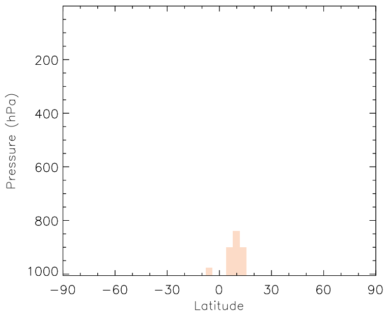
v11-01b-Run0 - v10-01-public-Run0 IEPOX - Zonal mean abs diff for Jul
