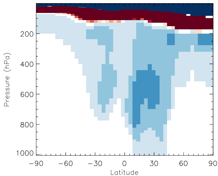
v11-01b-Run0 / v10-01-public-Run0 DMS - Zonal mean % diff for Jul
