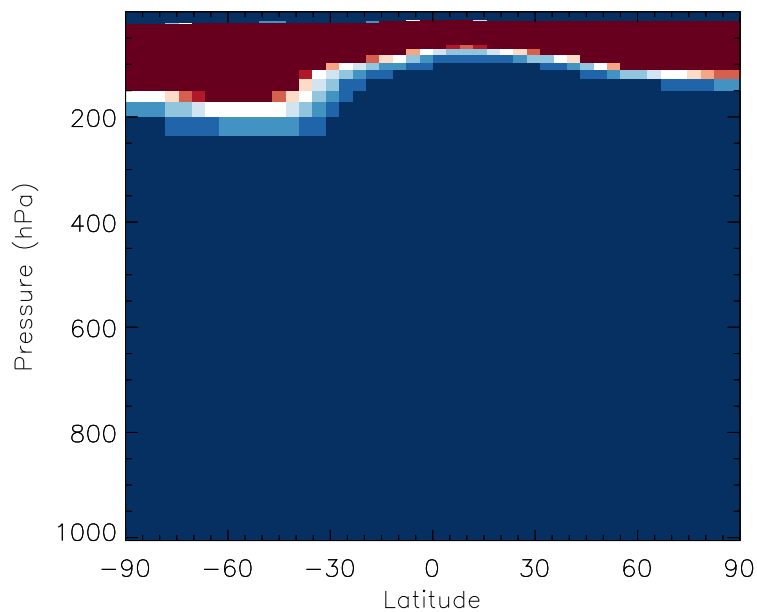
v11-01b-Run0 / v10-01-public-Run0 DST1 - Zonal mean % diff for Jul
