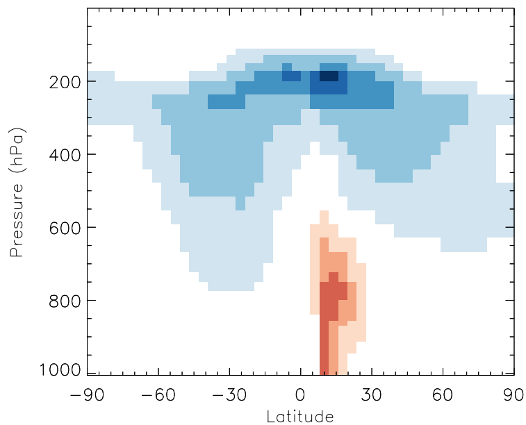
v11-01b-Run0 / v10-01-public-Run0 HOBr - Zonal mean % diff for Jul
