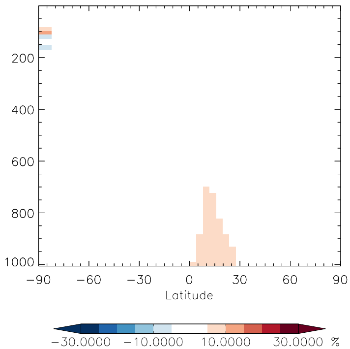
v11-01b-Run0 / v10-01-public-Run0 HCl - Zonal mean % diff for Jul
