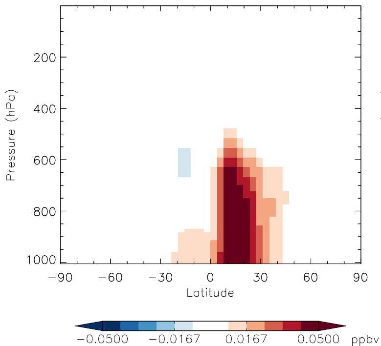
v11-01b-Run0 - v10-01-public-Run0 MP - Zonal mean abs diff for Jul
