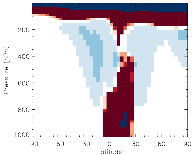
v11-01b-Run0 / v10-01-public-Run0 GLYC - Zonal mean % diff for Jul
