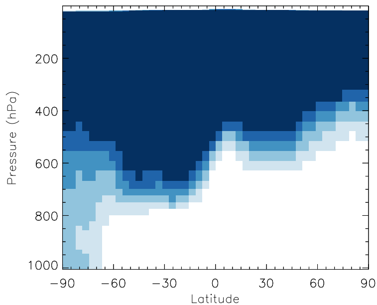
v11-01b-Run0 / v10-01-public-Run0 SALA - Zonal mean % diff for Jul
