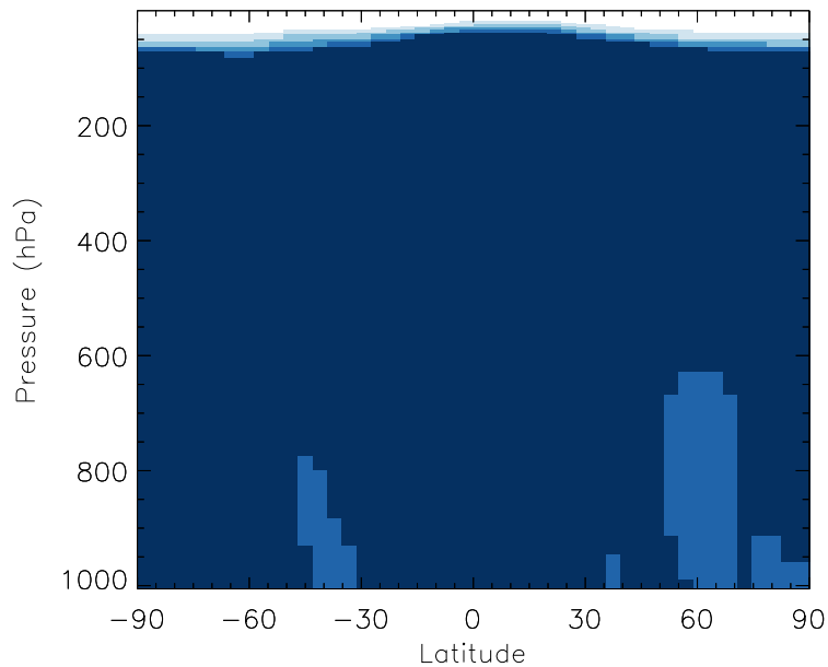
v11-01b-Run0 / v10-01i-geosp-Run0 OCPI - Zonal mean % diff for Jul
