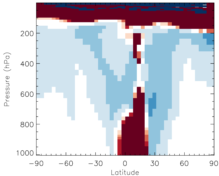
v11-01b-Run0 / v10-01i-geosp-Run0 MMN - Zonal mean % diff for Jul
