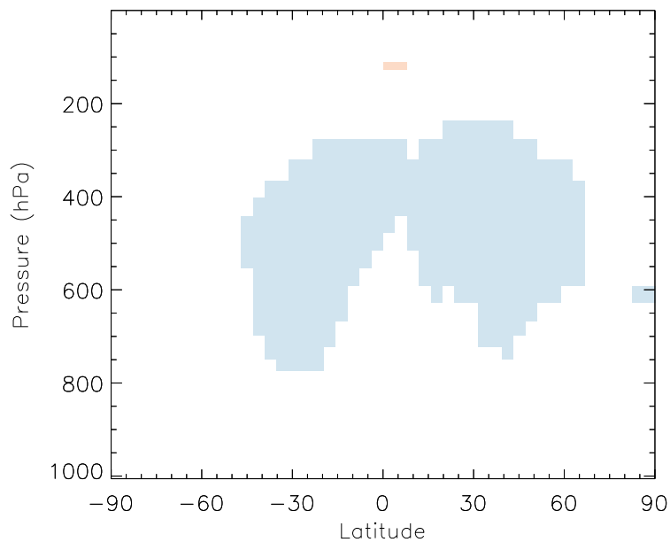
v11-01b-Run0 / v10-01-public-Run0 BrNO2 - Zonal mean % diff for Jul
