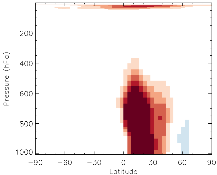
v11-01b-Run0 - v10-01i-geosfp-Run0 H2O2 - Zonal mean abs diff for Jul
