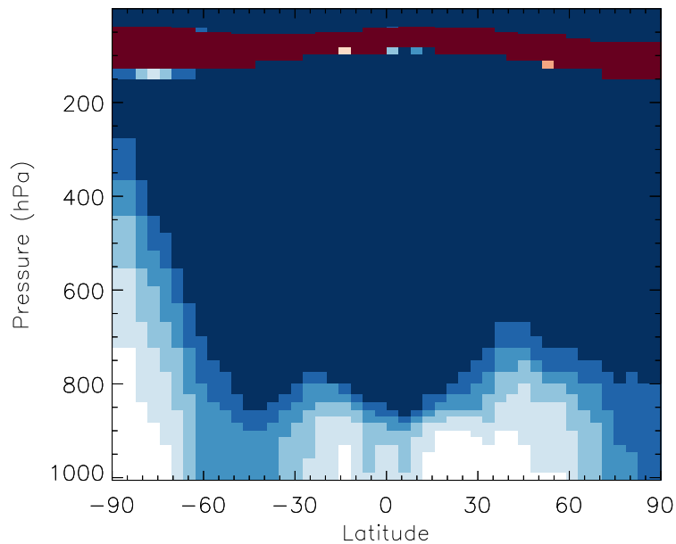
v11-01b-Run0 / v10-01i-geosfp-Run0 OCPO - Zonal mean % diff for Jul
