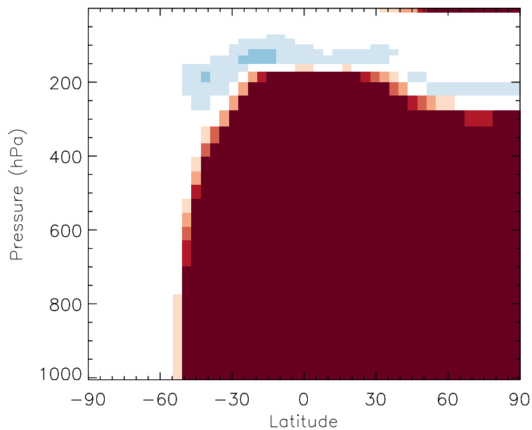
v11-01b-Run0 / v10-01-public-Run0 Cl2 - Zonal mean % diff for Jul
