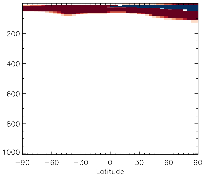
v11-01b-Run0 / v10-01-public-Run0 PROPNN - Zonal mean % diff for Jul
