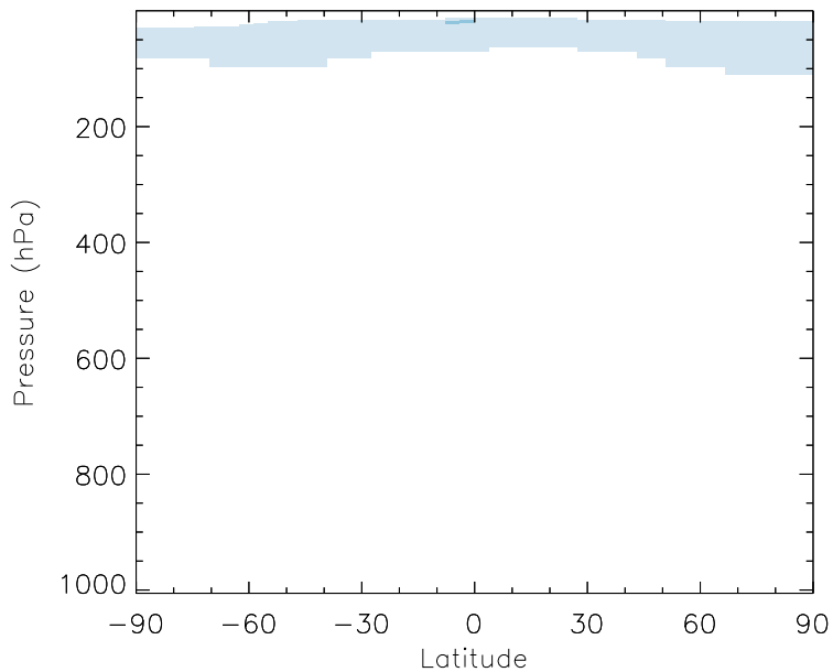
v11-01b-Run0 - v10-01i-geosfp-Run0 CH3Cl - Zonal mean abs diff for Jul
