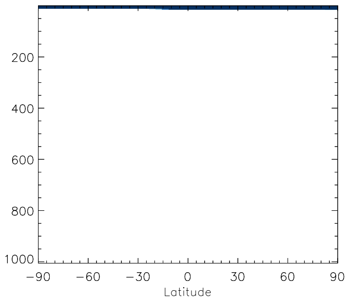
v11-01b-Run0 / v10-01-public-Run0 H1211 - Zonal mean % diff for Jul
