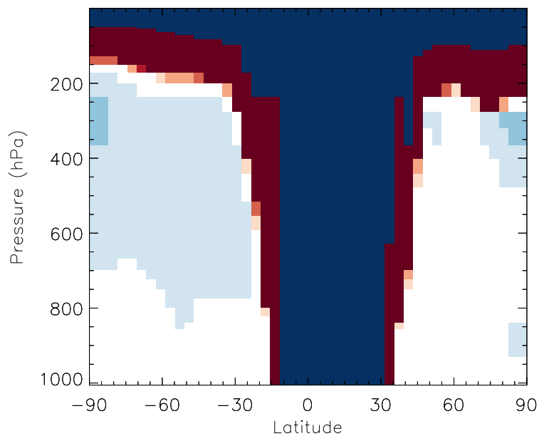
v11-01b-Run0 / v10-01-public-Run0 MVK - Zonal mean % diff for Jul
