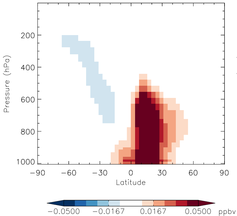
v11-01b-Run0 - v10-01i-geosp-Run0 MP - Zonal mean abs diff for Jul
