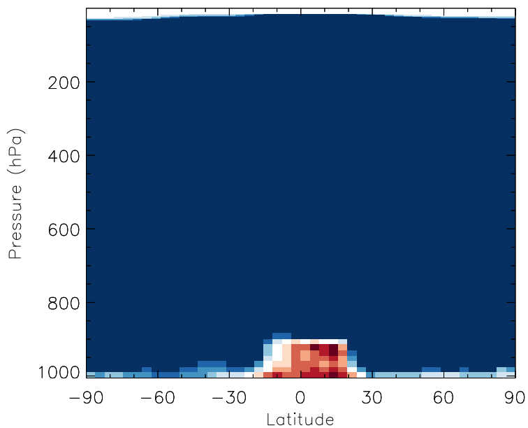
v11-01b-Run0 - v10-01-public-Run0 N2O - Zonal mean abs diff for Jul
