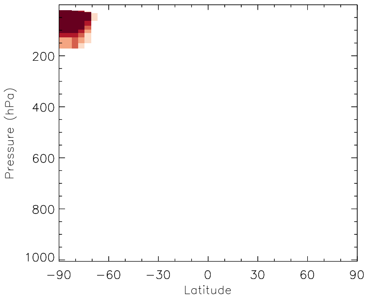
v11-01b-Run0 - v10-01i-geosp-Run0 NIT - Zonal mean abs diff for Jul
