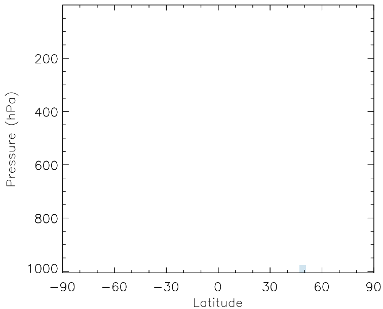
v11-01b-Run0 - v10-01i-geosfp-Run0 OCPO - Zonal mean abs diff for Jul
