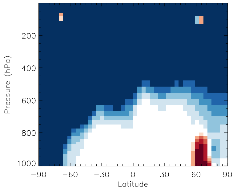
v11-01b-Run0 / v10-01i-geosfp-Run0 SO4s - Zonal mean % diff for Jul
