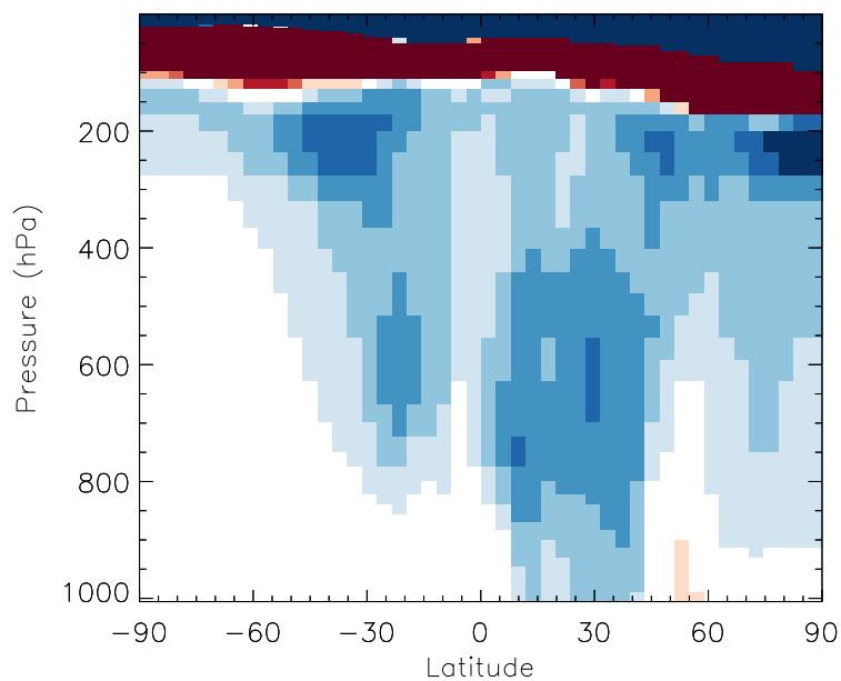
v11-01b-Run0 / v10-01i-geosfp-Run0 DMS - Zonal mean % diff for Jul
