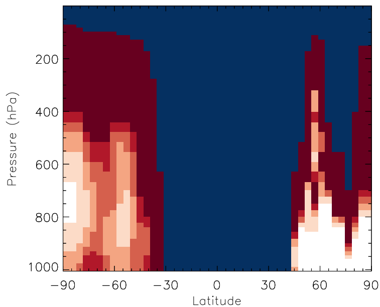
v11-01b-Run0 / v10-01-public-Run0 ISOP - Zonal mean % diff for Jul
