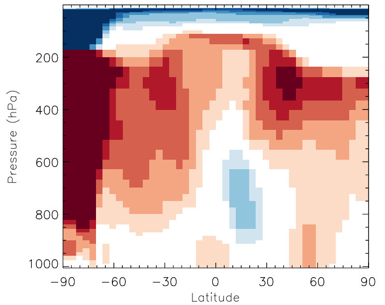
v11-01b-Run0 / v10-01i-geosp-Run0 HBr - Zonal mean % diff for Jul
