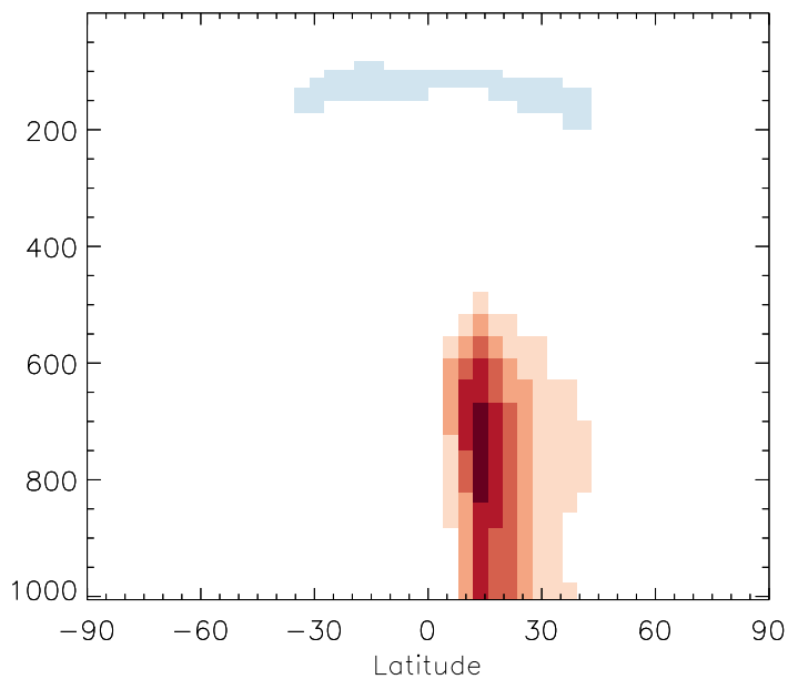
v11-01b-Run0 / v10-01-public-Run0 H2O2 - Zonal mean % diff for Jul
