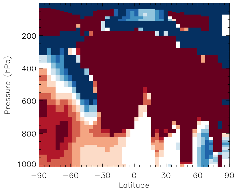
v11-01b-Run0 / v10-01i-geosp-Run0 NIT - Zonal mean % diff for Jul
