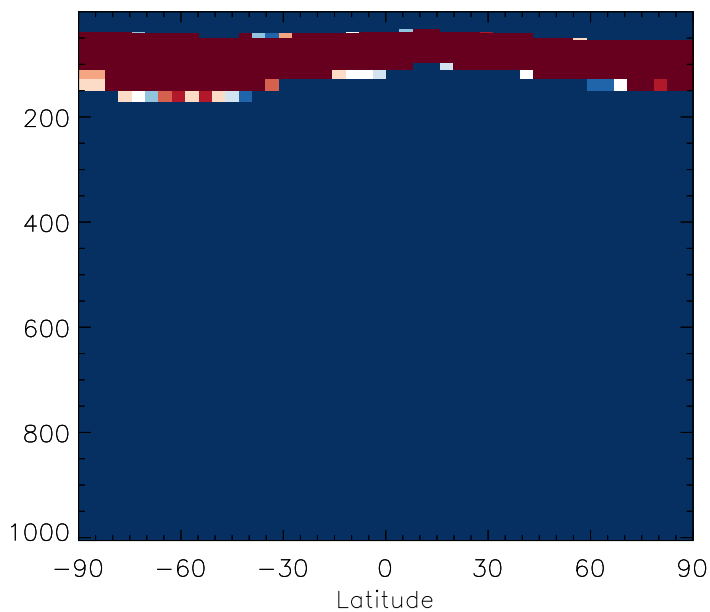
v11-01b-Run0 / v10-01-public-Run0 DST3 - Zonal mean % diff for Jul
