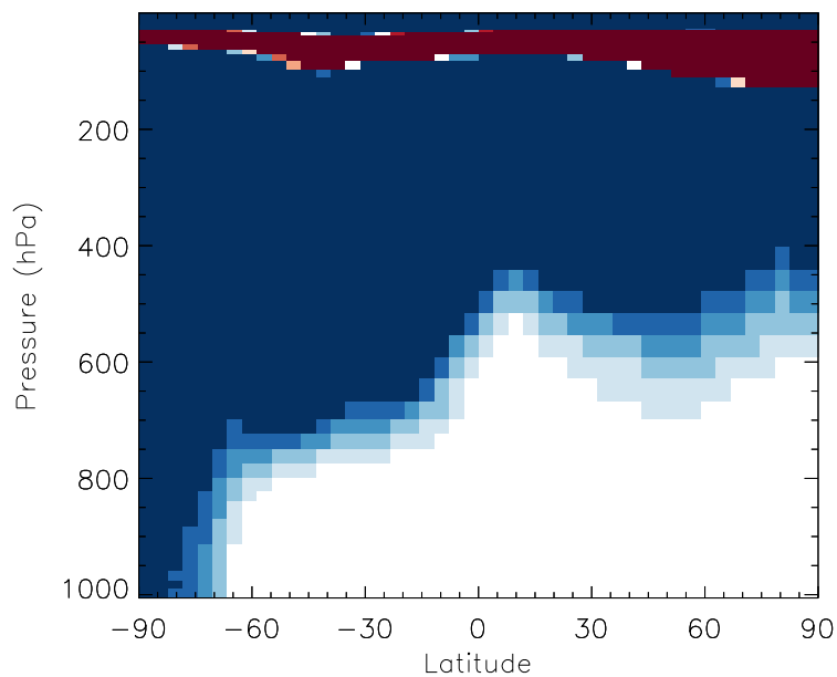
v11-01b-Run0 / v10-01-public-Run0 SALC - Zonal mean % diff for Jul
