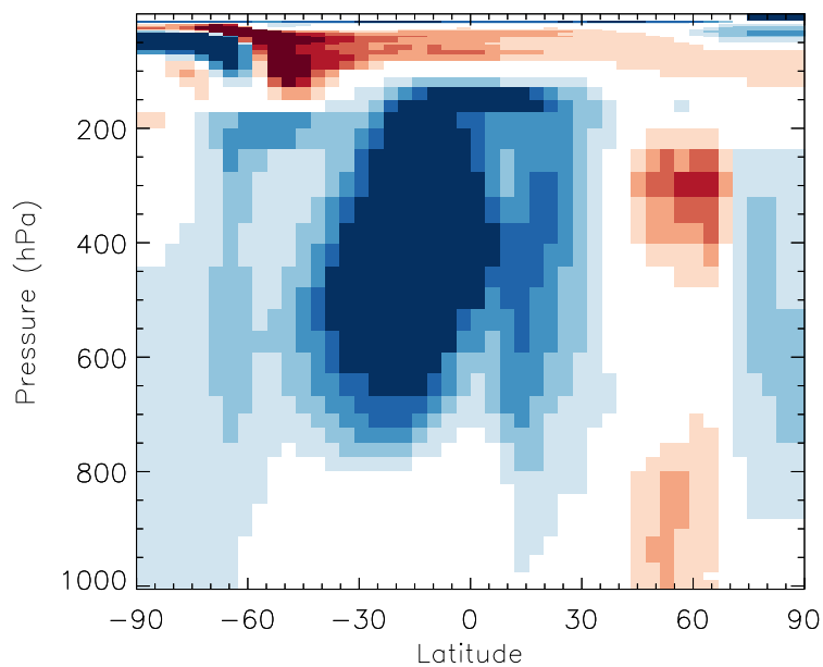
v11-01b-Run0 / v10-01i-geosp-Run0 Br2 - Zonal mean % diff for Jul
