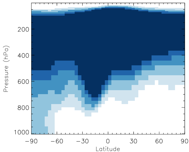
v11-01b-Run0 / v10-01-public-Run0 NH4 - Zonal mean % diff for Jul
