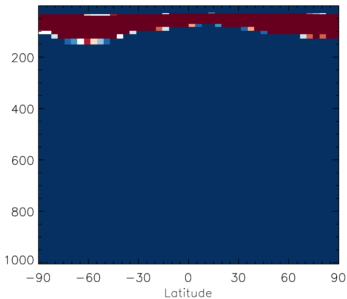
v11-01b-Run0 / v10-01-public-Run0 DST2 - Zonal mean % diff for Jul
