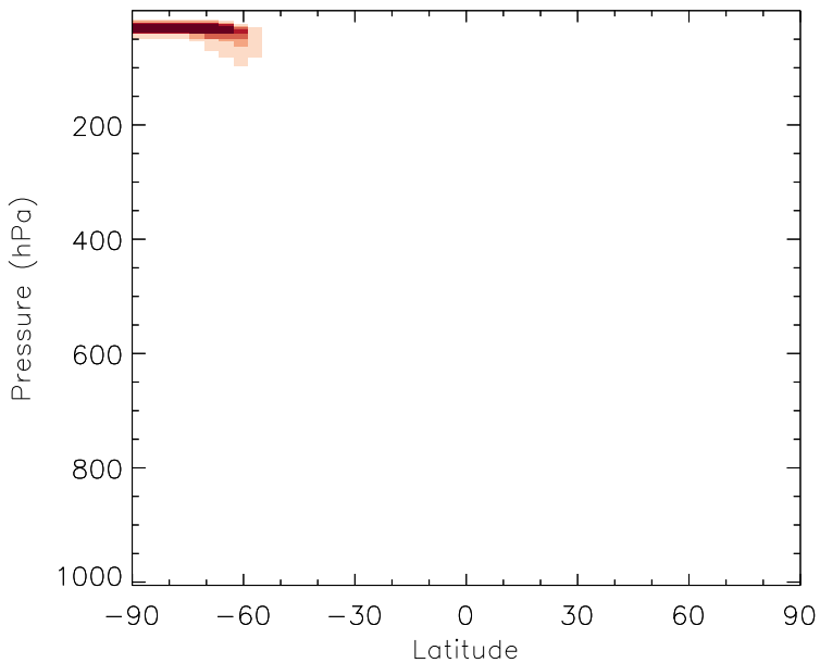
v11-01b-Run0 - v10-01i-geosfp-Run0 OCIO - Zonal mean abs diff for Jul
