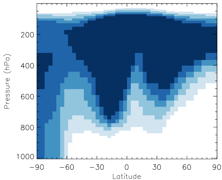
v11-01b-Run0 / v10-01-public-Run0 MSA - Zonal mean % diff for Jul
