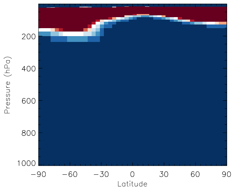
v11-01b-Run0 / v10-01i-geosfp-Run0 DST1 - Zonal mean % diff for Jul
