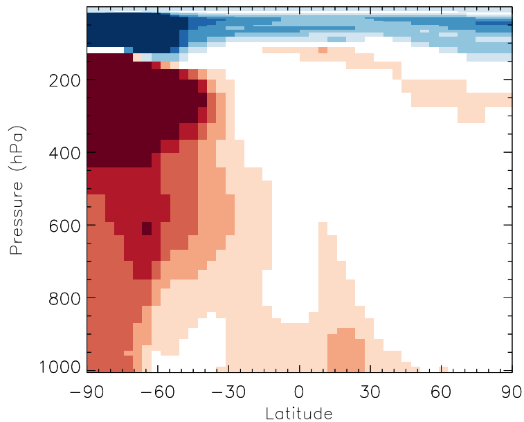
v11-01b-Run0 / v10-01i-geosfp-Run0 NO2 - Zonal mean % diff for Jul
