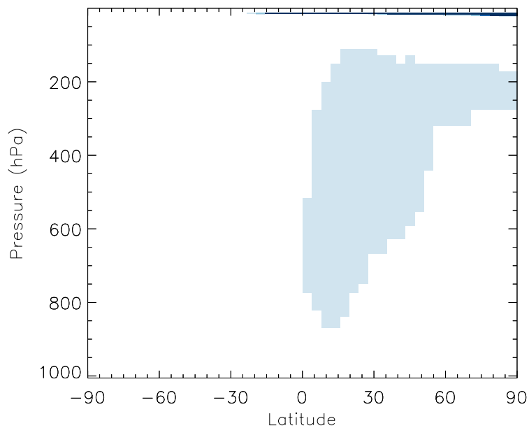
v11-01b-Run0 / v10-01-public-Run0 RCHO - Zonal mean % diff for Jul
