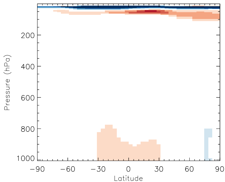
v11-01b-Run0 / v10-01i-geosfp-Run0 PAN - Zonal mean % diff for Jul
