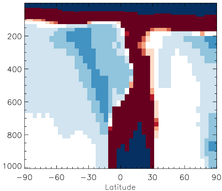
v11-01b-Run0 / v10-01i-geosp-Run0 IEPOX - Zonal mean % diff for Jul
