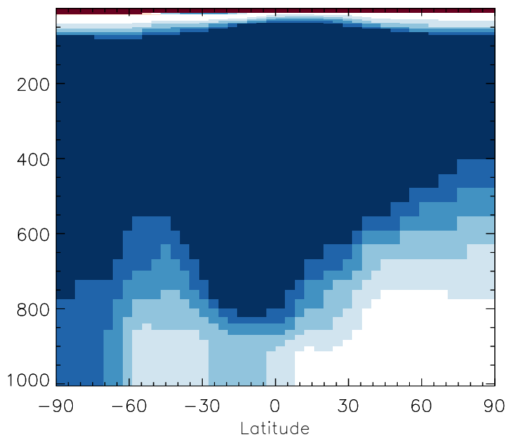
v11-01b-Run0 / v10-01-public-Run0 BCPI - Zonal mean % diff for Jul
