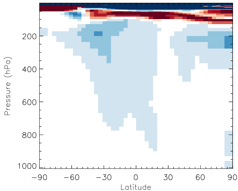
v11-01b-Run0 / v10-01i-geosfp-Run0 HAC - Zonal mean % diff for Jul
