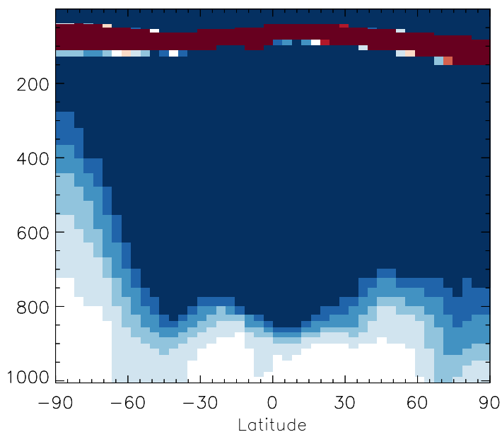
v11-01b-Run0 / v10-01i-geosp-Run0 BCPO - Zonal mean % diff for Jul
