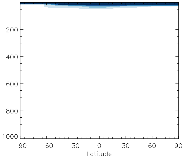
v11-01b-Run0 / v10-01i-geosfp-Run0 H2402 - Zonal mean % diff for Jul
