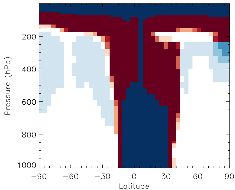
v11-01b-Run0 / v10-01-public-Run0 PMN - Zonal mean % diff for Jul
