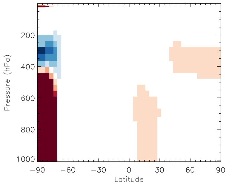
v11-01b-Run0 / v10-01-public-Run0 ClOO - Zonal mean % diff for Jul
