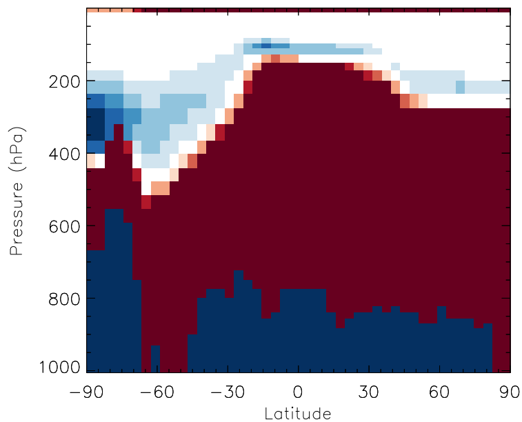
v11-01b-Run0 / v10-01-public-Run0 Cl2O2 - Zonal mean % diff for Jul
