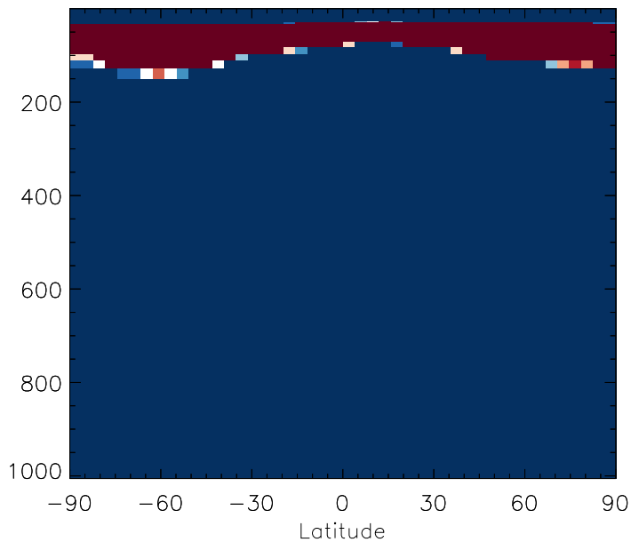
v11-01b-Run0 / v10-01i-geosfp-Run0 DST2 - Zonal mean % diff for Jul
