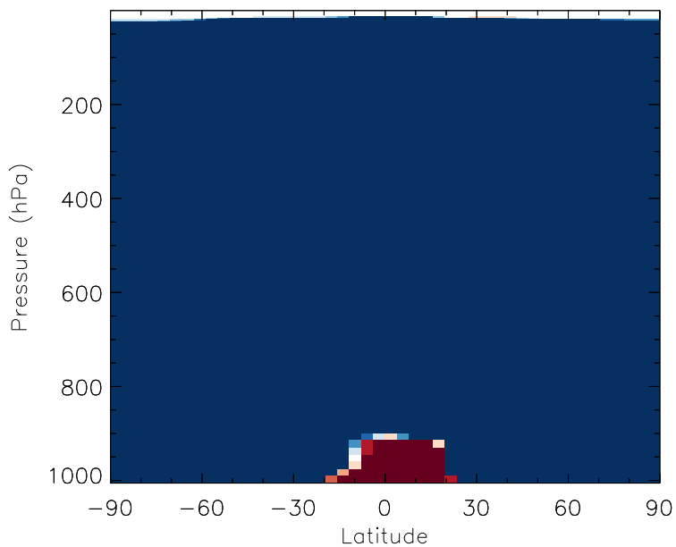
v11-01b-Run0 - v10-01-public-Run0 CH4 - Zonal mean abs diff for Jul
