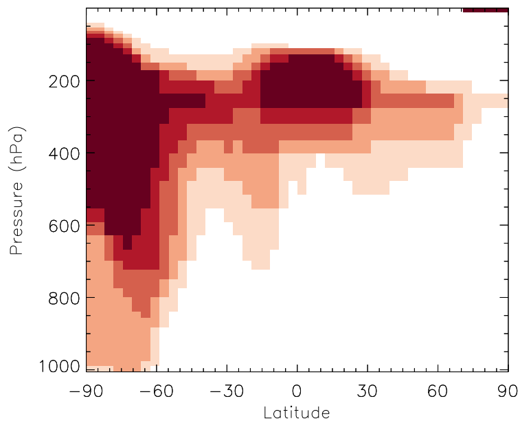
v11-01b-Run0 / v10-01-public-Run0 BrNO3 - Zonal mean % diff for Jul
