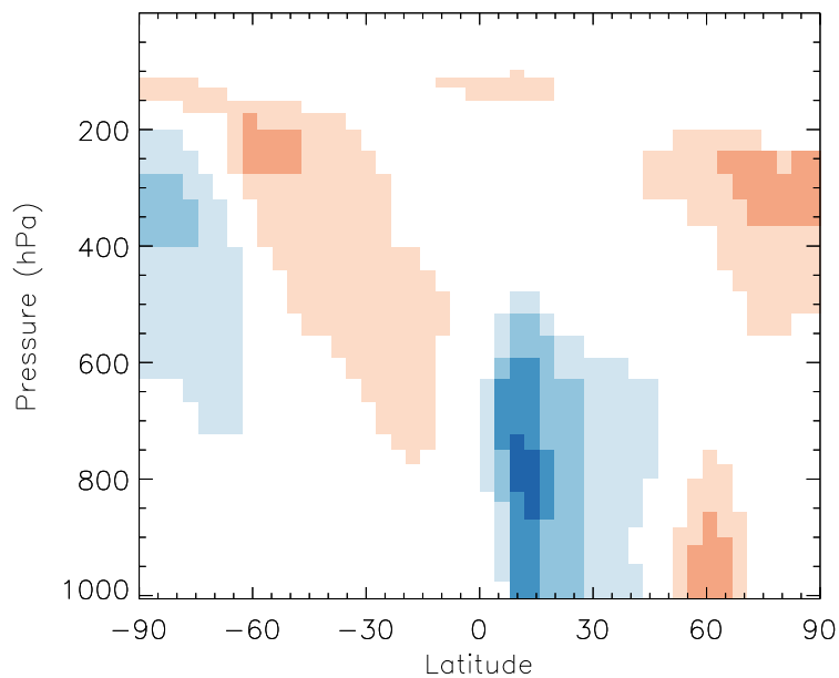
v11-01b-Run0 / v10-01-public-Run0 HN02 - Zonal mean % diff for Jul
