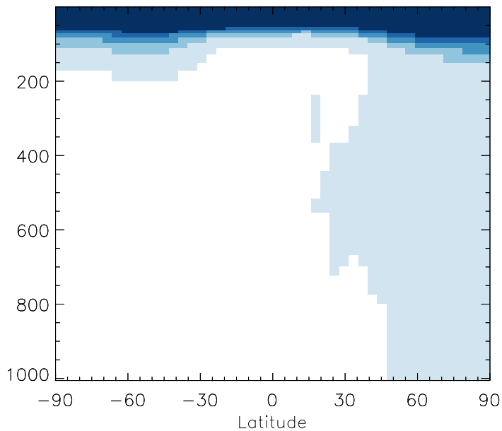
v11-01b-Run0 / v10-01i-geosp-Run0 C2H6 - Zonal mean % diff for Jul
