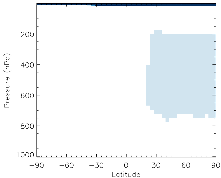
v11-01b-Run0 / v10-01-public-Run0 CH2Br2 - Zonal mean % diff for Jul
