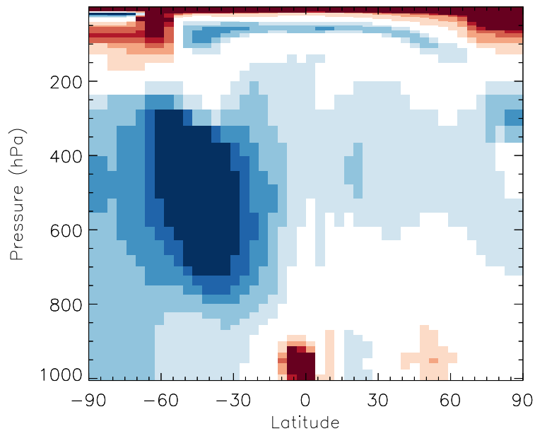
v11-01b-Run0 / v10-01i-geosfp-Run0 BrCl - Zonal mean % diff for Jul
