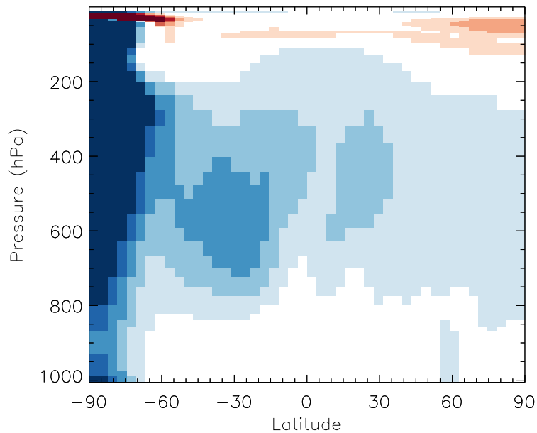
v11-01b-Run0 / v10-01i-geosfp-Run0 BrO - Zonal mean % diff for Jul
