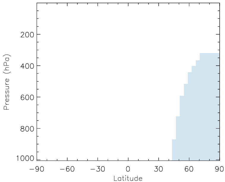
v11-01b-Run0 - v10-01i-geosp-Run0 C2H6 - Zonal mean abs diff for Jul
