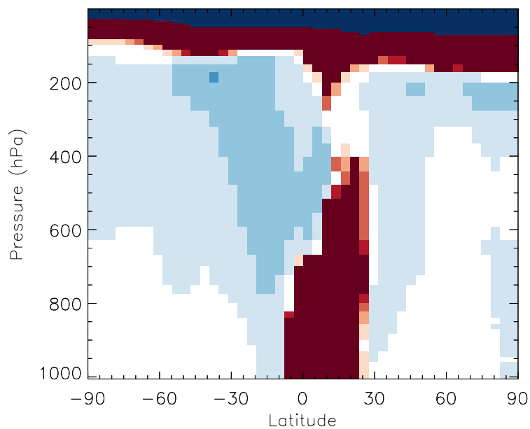
v11-01b-Run0 / v10-01i-geosp-Run0 GLYC - Zonal mean % diff for Jul
