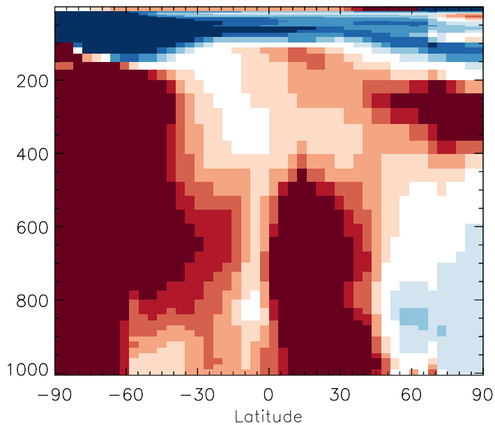
v11-01b-Run0 / v10-01i-geosfp-Run0 N2O5 - Zonal mean % diff for Jul
