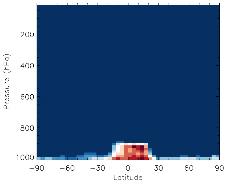
v11-01b-Run0 - v10-01i-geosfp-Run0 N2O - Zonal mean abs diff for Jul
