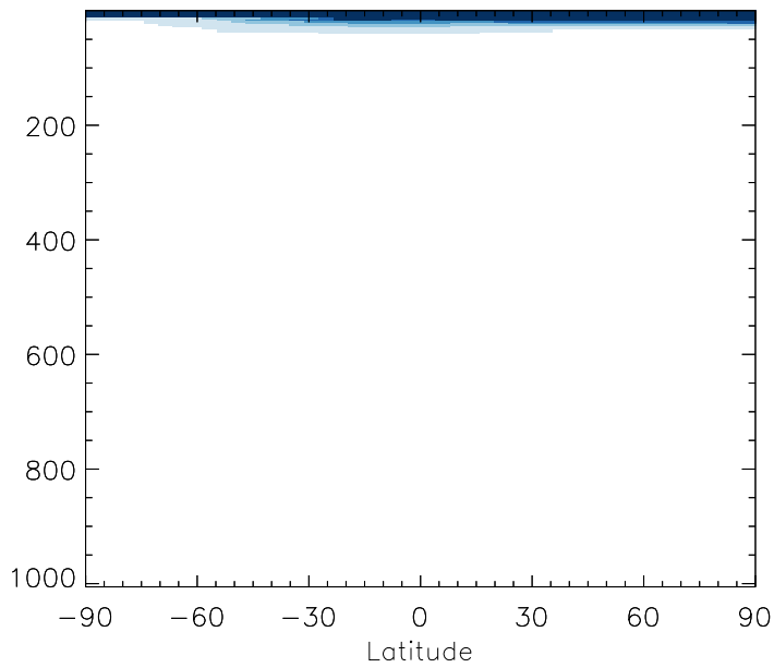
v11-01b-Run0 / v10-01i-geosfp-Run0 CH 3 CCl 3 - Zonal mean % diff for Jul
