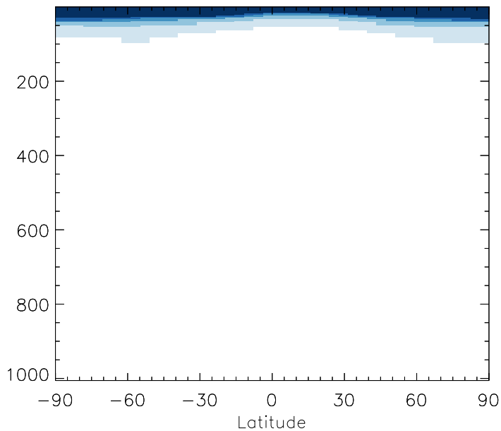
v11-01b-Run0 / v10-01i-geosfp-Run0 CH3Cl - Zonal mean % diff for Jul
