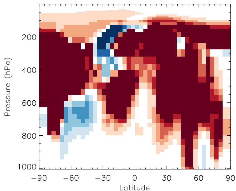
v11-01b-Run0 / v10-01i-geosfp-Run0 NH3 - Zonal mean % diff for Jul
