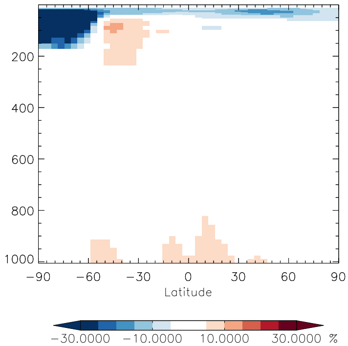
v11-01b-Run0 / v10-01i-geosfp-Run0 HCl - Zonal mean % diff for Jul
