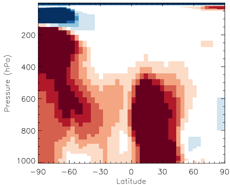
v11-01b-Run0 / v10-01i-geosfp-Run0 NO3 - Zonal mean % diff for Jul
