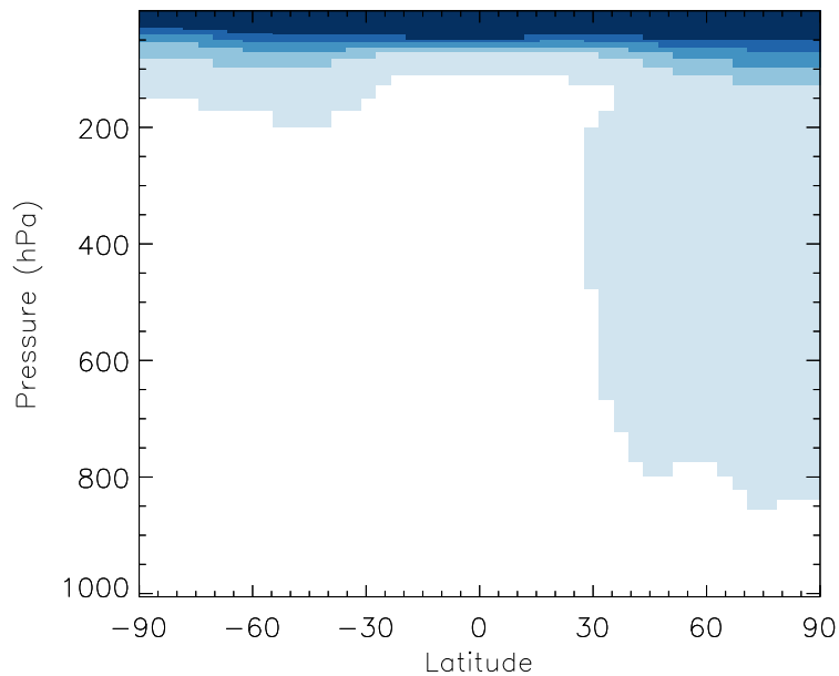
v11-01b-Run0 / v10-01i-geosp-Run0 CH2Br2 - Zonal mean % diff for Jul
