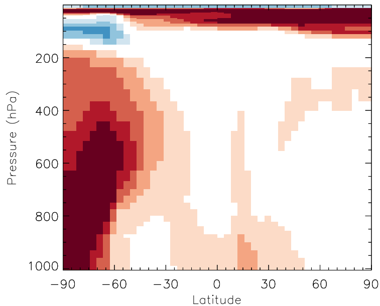
v11-01b-Run0 / v10-01i-geosfp-Run0 MPN - Zonal mean % diff for Jul
