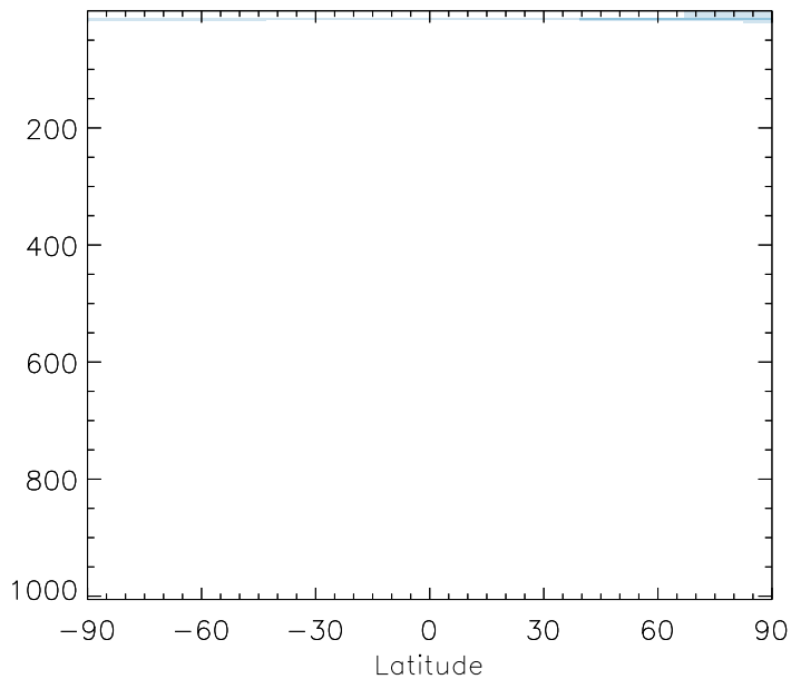
v11-01b-Run0 / v10-01i-geosfp-Run0 N2O - Zonal mean % diff for Jul
