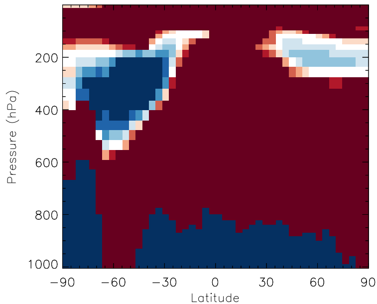
v11-01b-Run0 / v10-01i-geosfp-Run0 Cl2O2 - Zonal mean % diff for Jul
