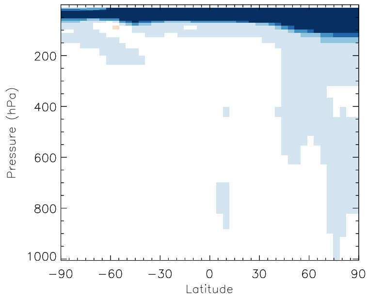
v11-01b-Run0 / v10-01i-geosp-Run0 RCHO - Zonal mean % diff for Jul
