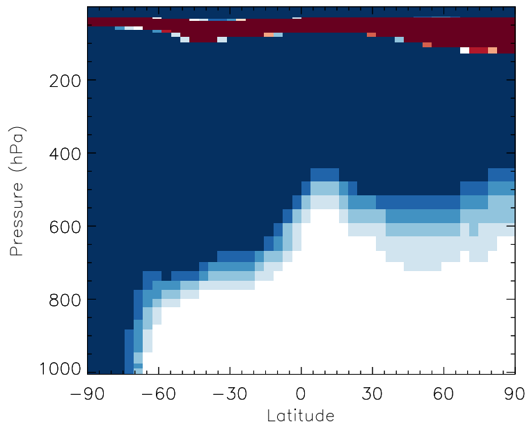
v11-01b-Run0 / v10-01i-geosfp-Run0 SALC - Zonal mean % diff for Jul
