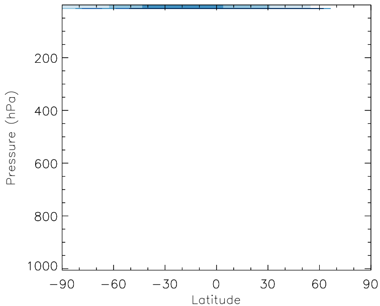
v11-01b-Run0 - v10-01i-geosfp-Run0 NO3 - Zonal mean abs diff for Jul
