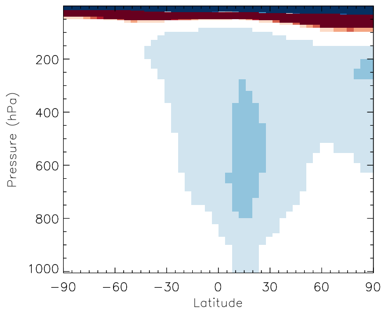
v11-01b-Run0 / v10-01-public-Run0 ALK4 - Zonal mean % diff for Jul
