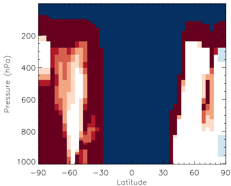
v11-01b-Run0 / v10-01-public-Run0 MOBA - Zonal mean % diff for Jul
