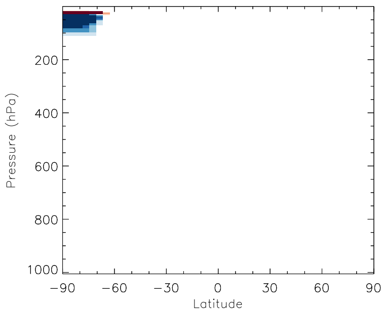
v11-01b-Run0 - v10-01i-geosfp-Run0 Cl2 - Zonal mean abs diff for Jul
