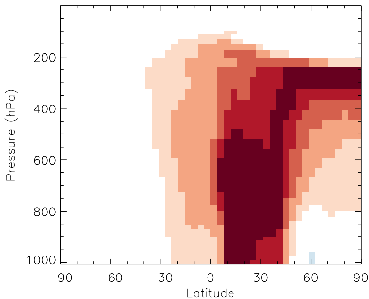
v11-01b-Run0 - v10-01-public-Run0 OH - Zonal mean abs diff for Jul
