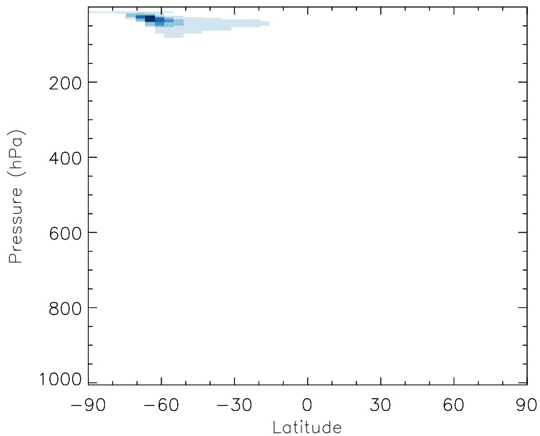
v11-01b-Run0 - v10-01i-geosfp-Run0 BrNO3 - Zonal mean abs diff for Jul
