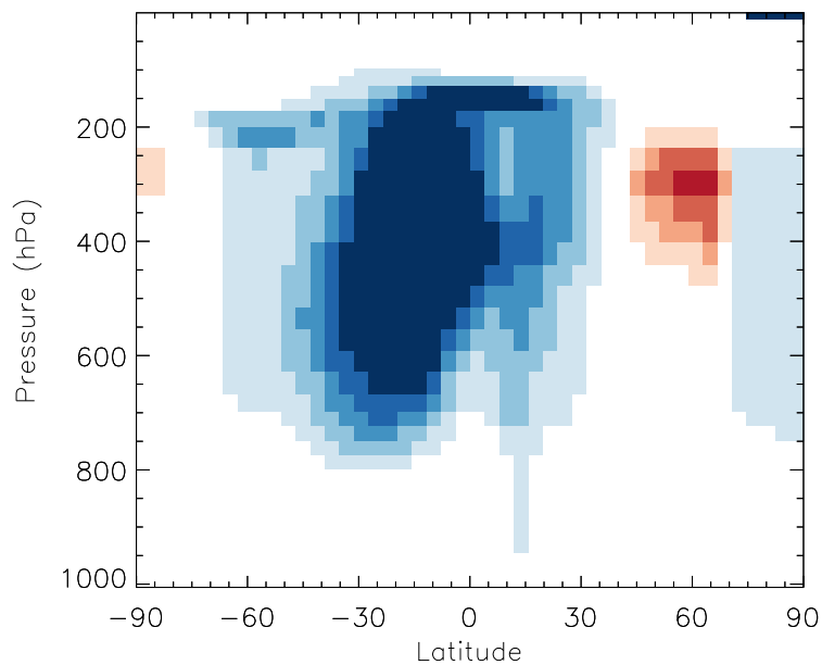
v11-01b-Run0 / v10-01-public-Run0 Br2 - Zonal mean % diff for Jul
