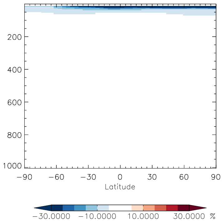
v11-01b-Run0 / v10-01i-geosfp-Run0 CH3Br - Zonal mean % diff for Jul
