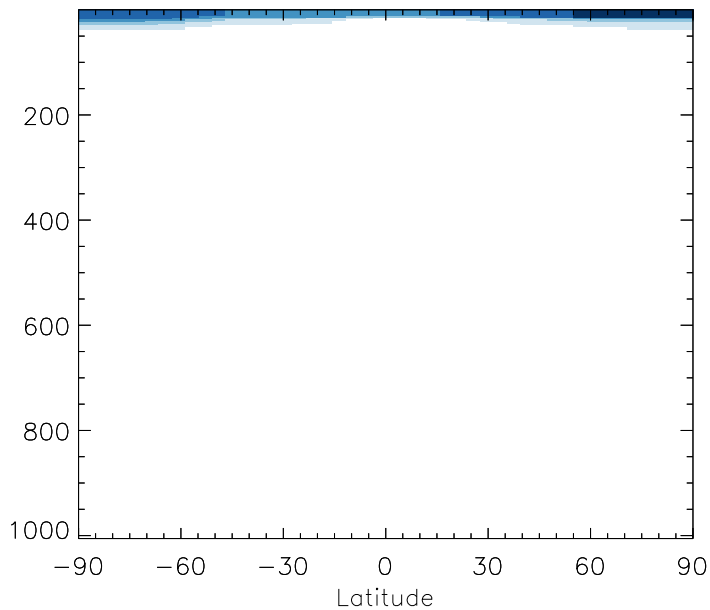
v11-01b-Run0 / v10-01i-geosfp-Run0 CH4 - Zonal mean % diff for Jul
