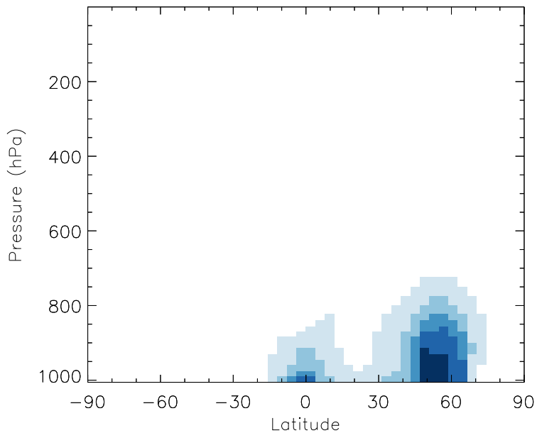
v11-01b-Run0 - v10-01i-geosp-Run0 OCPI - Zonal mean abs diff for Jul
