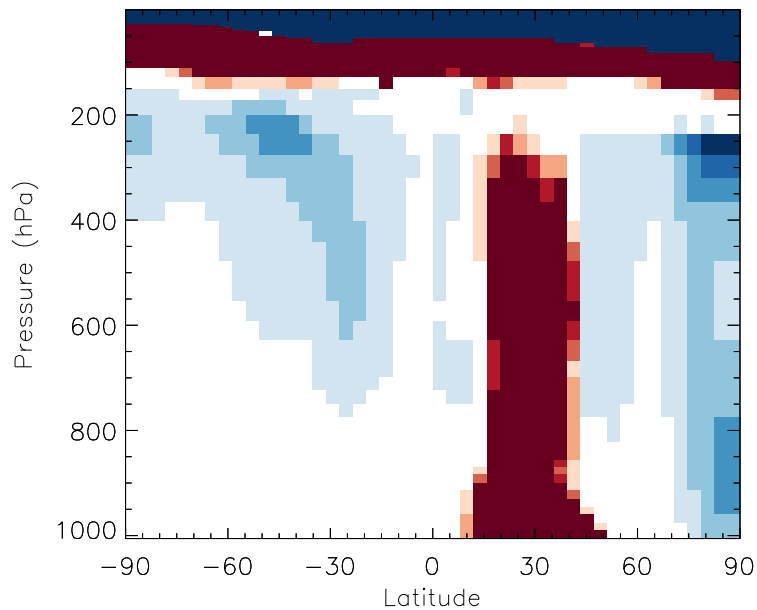
v11-01b-Run0 / v10-01i-geosp-Run0 PRPE - Zonal mean % diff for Jul
