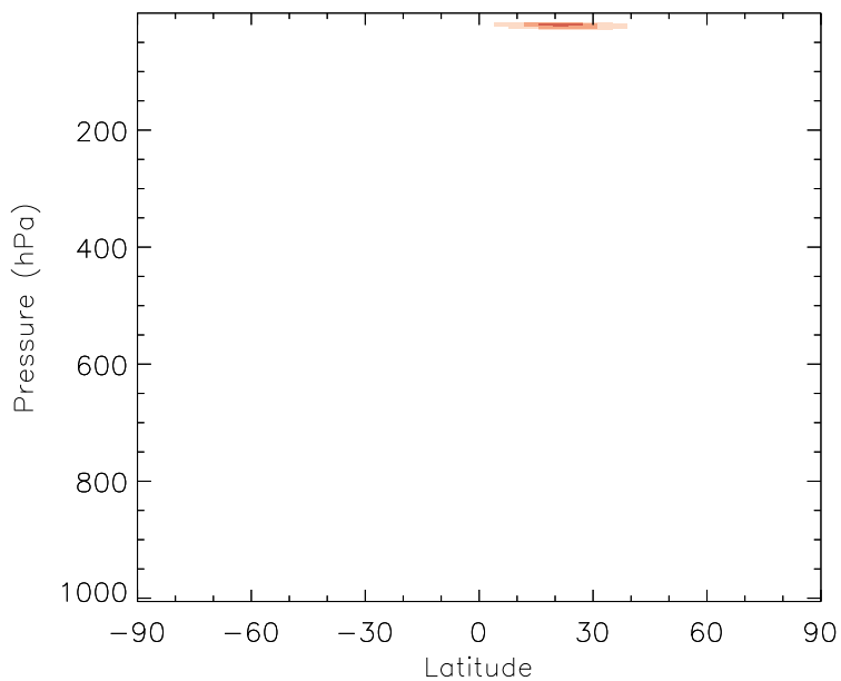
v11-01b-Run0 - v10-01-public-Run0 O3 - Zonal mean abs diff for Jul
