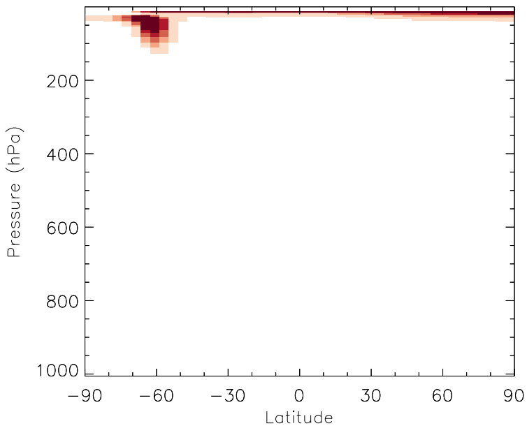
v11-01b-Run0 - v10-01i-geosfp-Run0 ClO - Zonal mean abs diff for Jul
