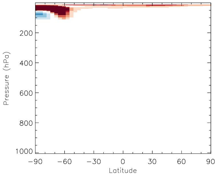
v11-01b-Run0 - v10-01i-geosfp-Run0 HOCl - Zonal mean abs diff for Jul
