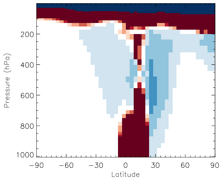
v11-01b-Run0 / v10-01-public-Run0 MMN - Zonal mean % diff for Jul
