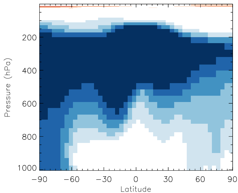
v11-01b-Run0 / v10-01i-geosfp-Run0 SO4 - Zonal mean % diff for Jul
