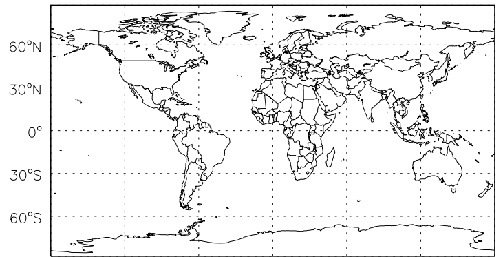
Abs Diff @ 500 hPa - Rn
