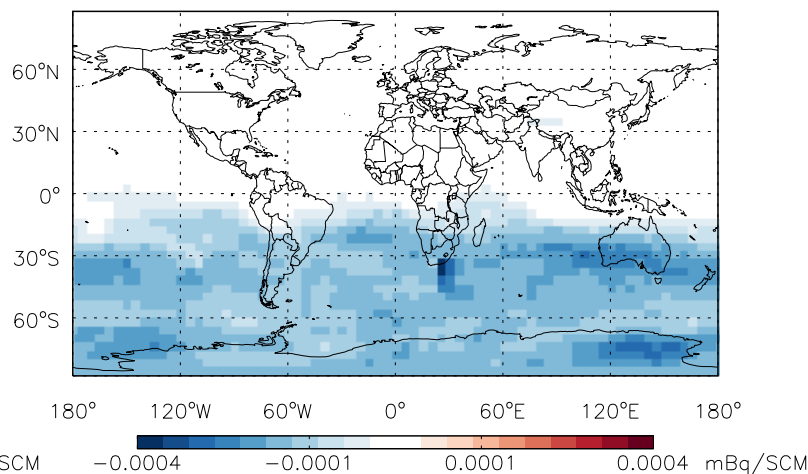
Abs Diff @ 500 hPa - Be7
