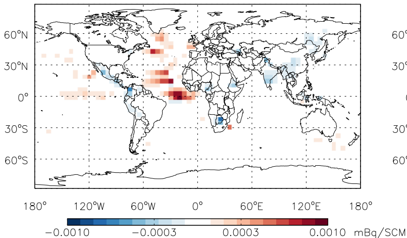
Abs Diff @ Surface - Pb
