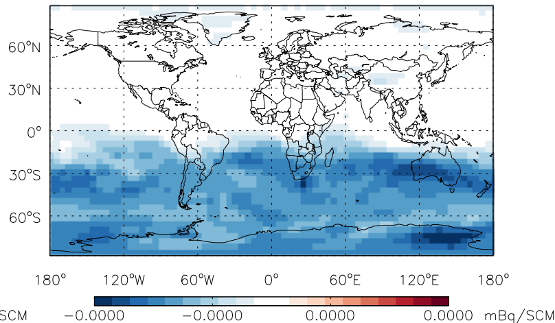
Abs Diff @ 500 hPa - Pb
