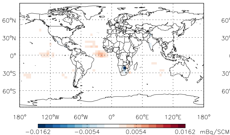
Abs Diff @ Surface - Be7
