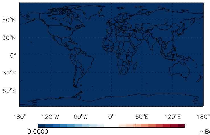
Abs Diff @ Surface - Rn
