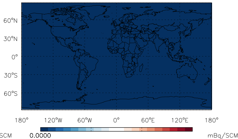
Abs Diff @ 500 hPa - Rn
