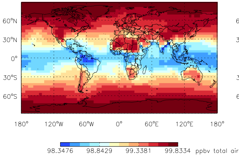
Tracer Map @ Surface - PASV - Apr
