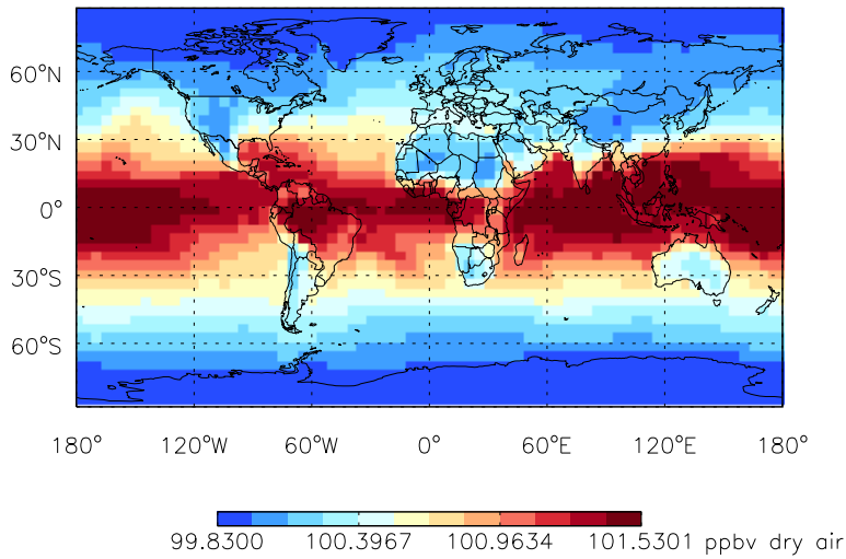
Tracer Map @ Surface - PASV - Apr
