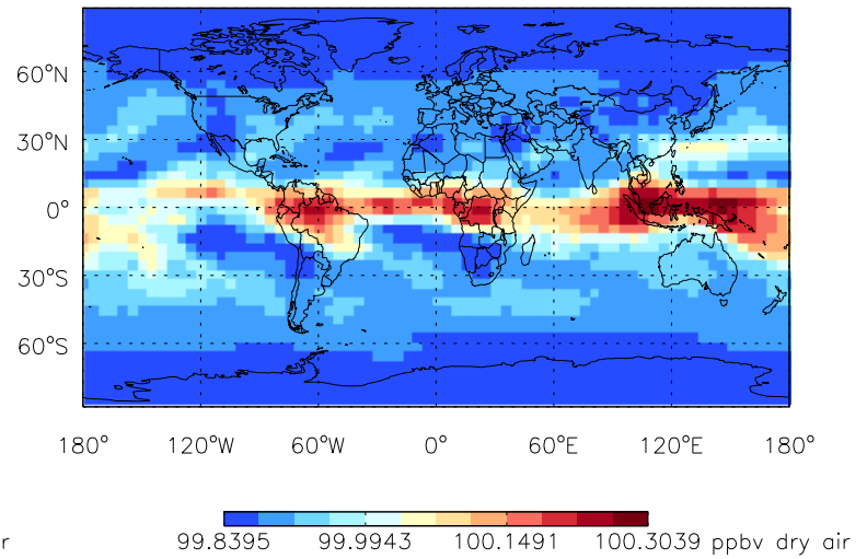
Tracer Map @ 500 hPa - PASV - Apr
