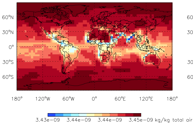
Tracer Map @ Surface - PASV - Apr
