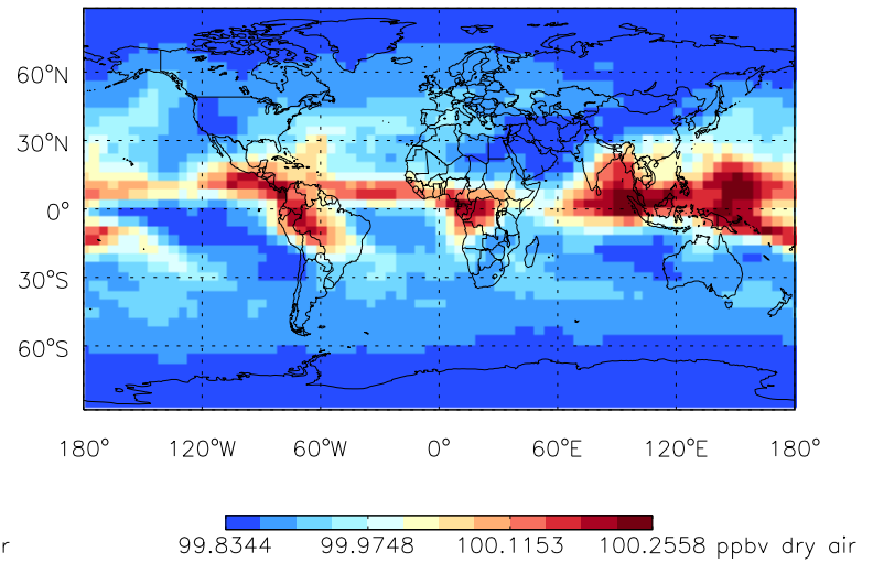
Tracer Map @ 500 hPa - PASV - Oct
