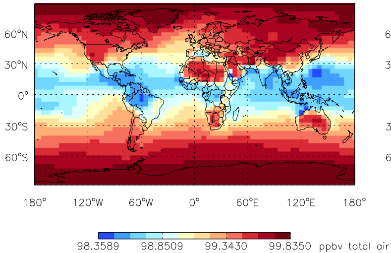
Tracer Map @ Surface - PASV - Oct
