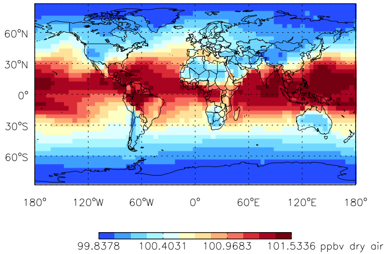
Tracer Map @ Surface - PASV - Oct
