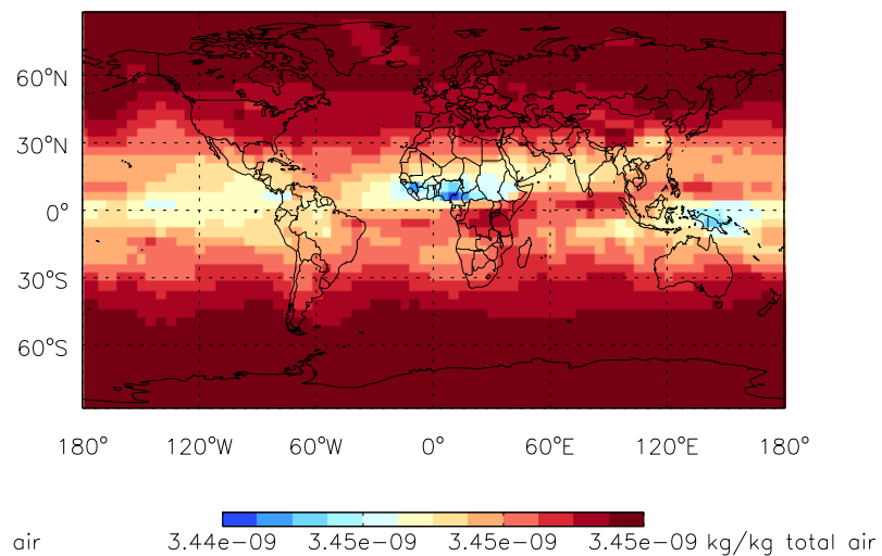
Tracer Map @ 500 hPa - PASV - Apr
