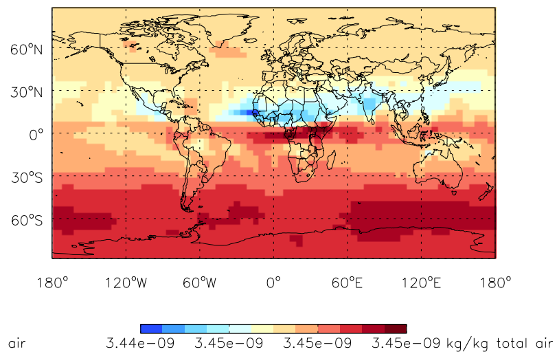
Tracer Map @ 500 hPa - PASV - Oct
