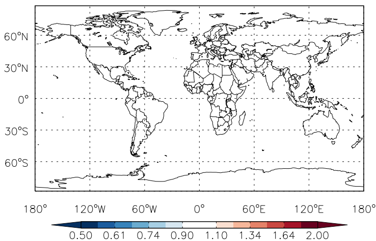
Ratio @ Surface for Be7
