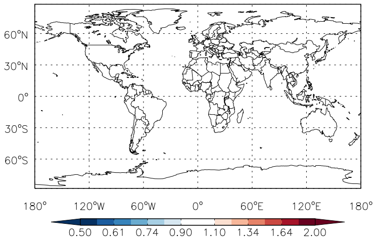
Ratio @ Surface for Pb
