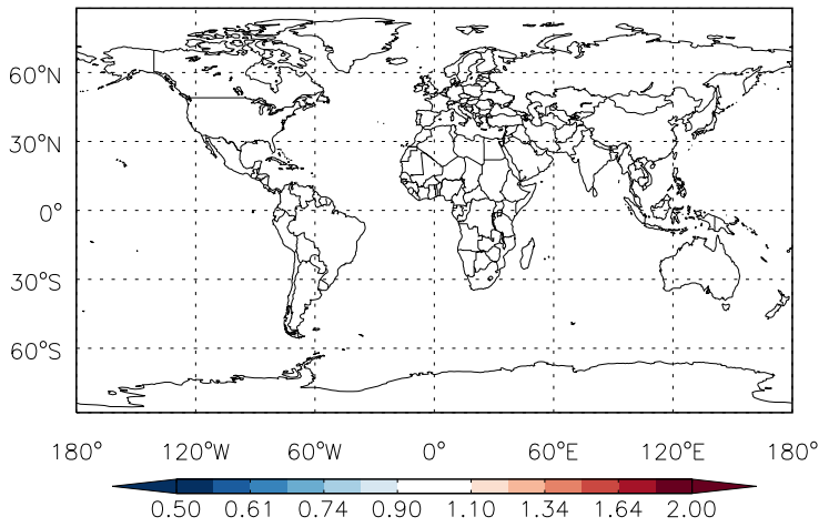
Ratio @ Surface for Rn
