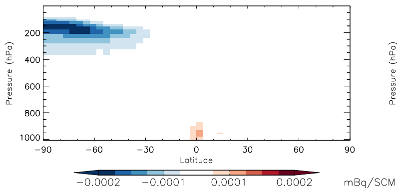
Zonal mean abs diff: Pb
