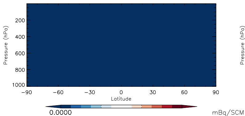
Zonal mean abs diff: Rn
