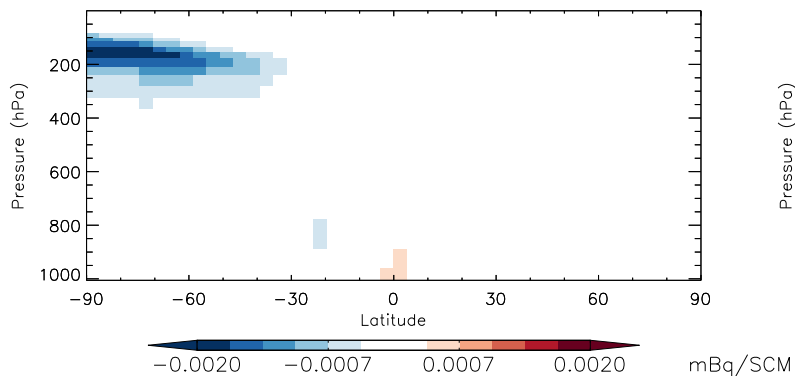
Zonal mean abs diff: Be7
