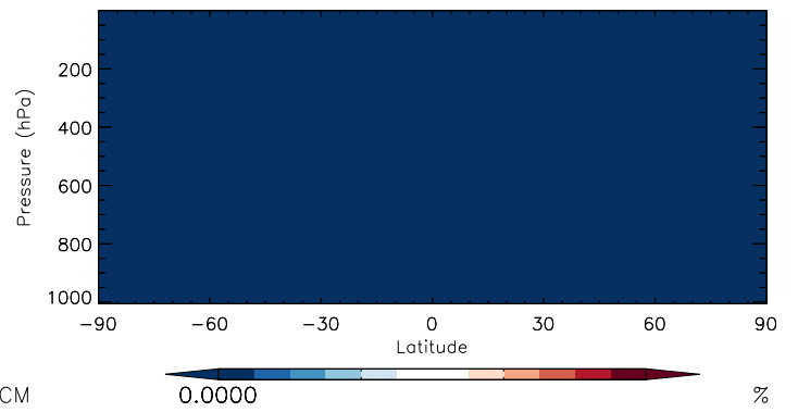
Zonal mean % diff: Rn
