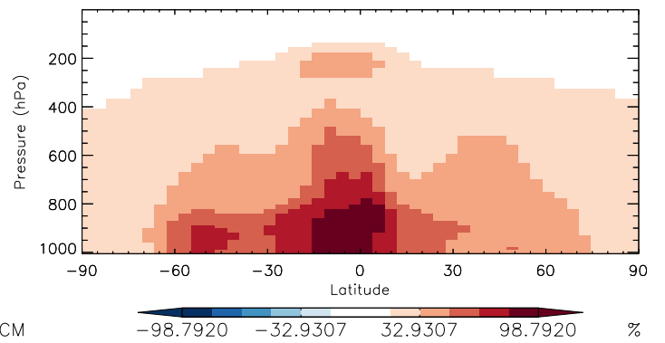
Zonal mean % diff: Be7
