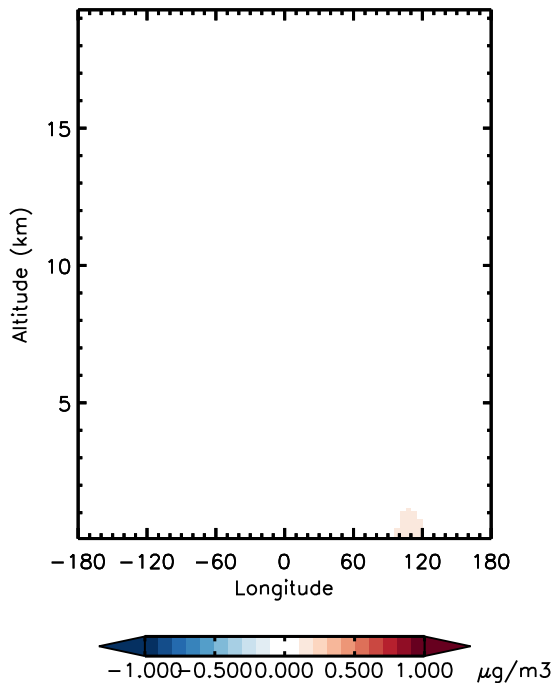
v11-01d-Run0 - v11-01b-Run0 SALA - Diff along 15S for Jan
