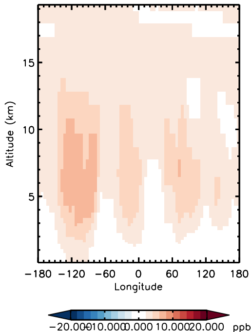
v11-01d-Run0 - v11-01b-Run0 O3 - Diff along 15S for Jan
