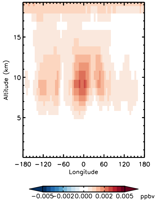
v11-01d-Run0 - v10-01-public-Run0 N2O5 - Diff along 15S for Jan
