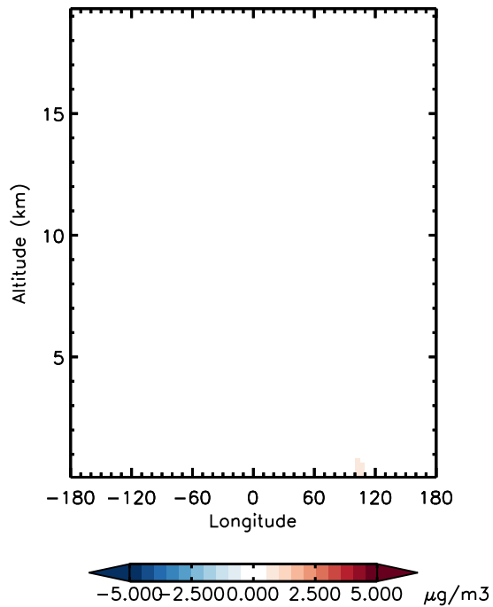
v11-01d-Run0 - v10-01-public-Run0 DST4 - Diff along 42N for Jan
