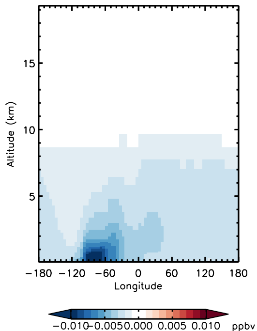
v11-01d-Run0 - v11-01b-Run0 R4N2 - Diff along 42N for Jan
