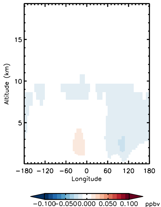
v11-01d-Run0 - v11-01b-Run0 H2O2 - Diff along 42N for Jan
