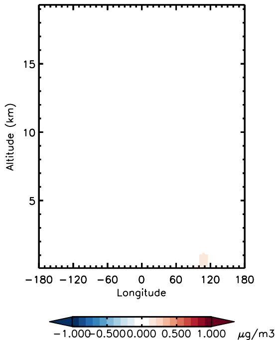
v11-01d-Run0 - v10-01-public-Run0 SALA - Diff along 15S for Jan
