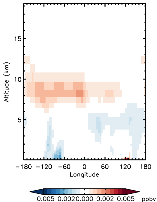
v11-01d-Run0 - v11-01b-Run0 HNO 4 - Diff along 42N for Jan
