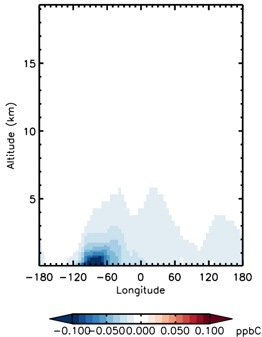
v11-01d-Run0 - v10-01-public-Run0 MEK - Diff along 42N for Jan
