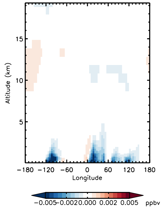
v11-01d-Run0 - v11-01b-Run0 N2O5 - Diff along 42N for Jan
