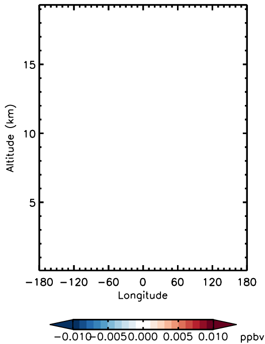
v11-01d-Run0 - v10-01-public-Run0 CH2Br2 - Diff along 15S for Jan
