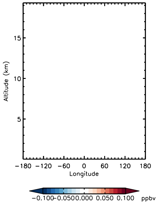
v11-01d-Run0 - v10-01-public-Run0 H1211 - Diff along 15S for Jan
