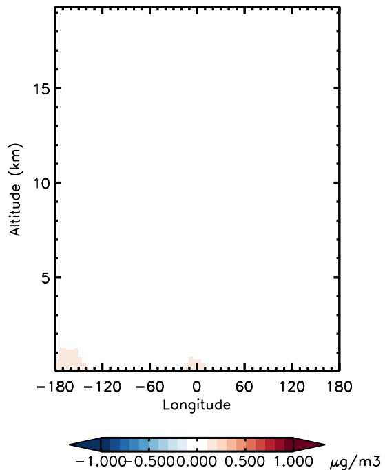
v11-01d-Run0 - v10-01-public-Run0 SALA - Diff along 42N for Jan
