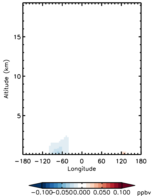
v11-01d-Run0 - v10-01-public-Run0 PAN - Diff along 42N for Jan
