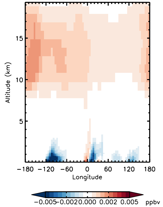
v11-01d-Run0 - v10-01-public-Run0 N2O5 - Diff along 42N for Jan
