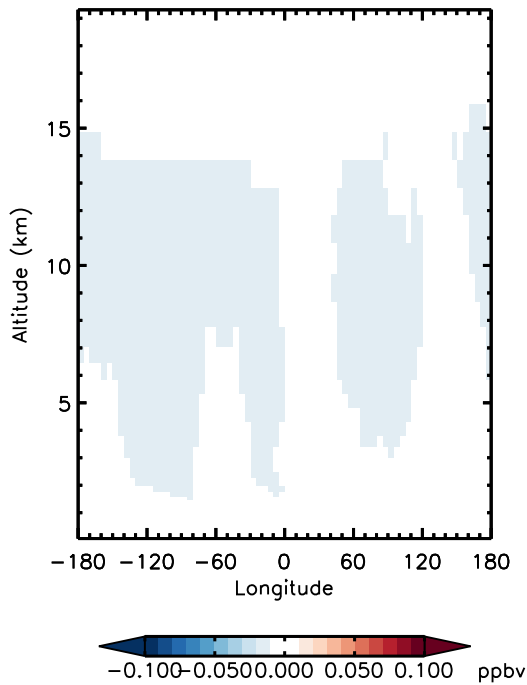
v11-01d-Run0 - v10-01-public-Run0 CH3Cl - Diff along 15S for Jan
