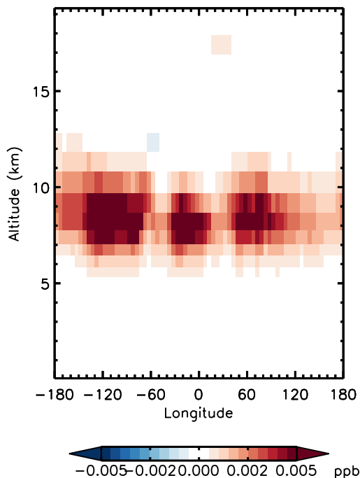
v11-01d-Run0 - v11-01b-Run0 HNO 4 - Diff along 15S for Jan
