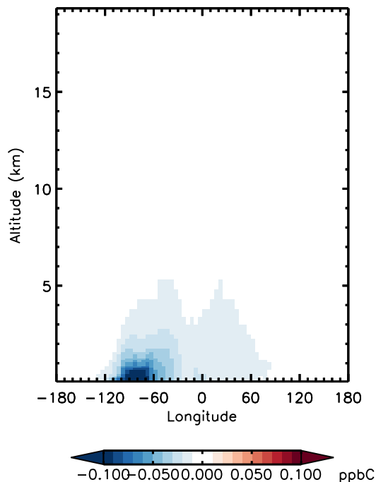
v11-01d-Run0 - v11-01b-Run0 MEK - Diff along 42N for Jan
