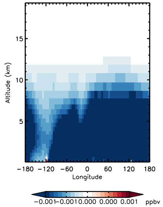
v11-01d-Run0 - v11-01b-Run0 PPN - Diff along 42N for Jan
