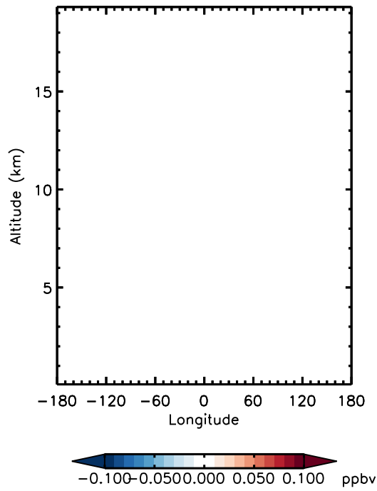
v11-01d-Run0 - v11-01b-Run0 H1301 - Diff along 15S for Jan
