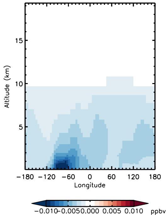
v11-01d-Run0 - v10-01-public-Run0 R4N2 - Diff along 42N for Jan
