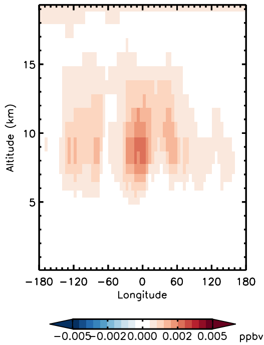
v11-01d-Run0 - v11-01b-Run0 N2O5 - Diff along 15S for Jan
