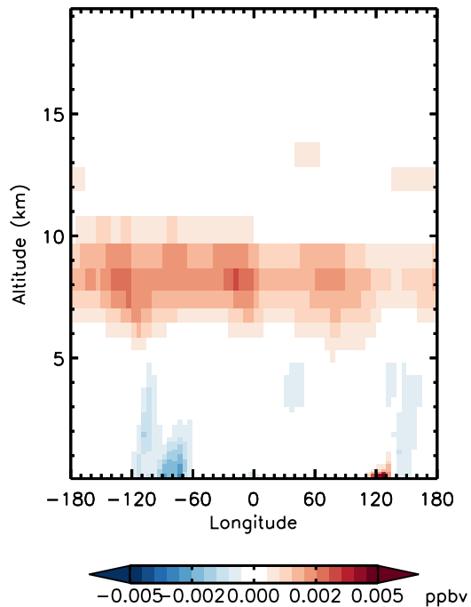
v11-01d-Run0 - v10-01-public-Run0 HNO 4 - Diff along 42N for Jan
