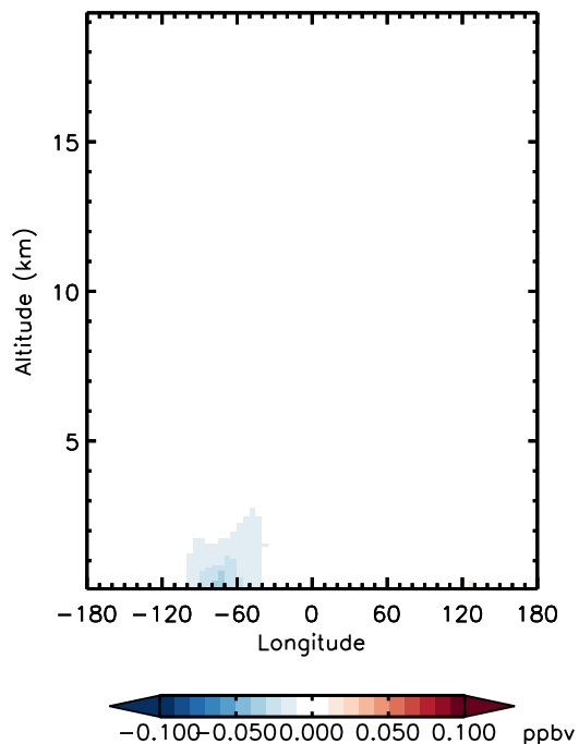
v11-01d-Run0 - v11-01b-Run0 PAN - Diff along 42N for Jan
