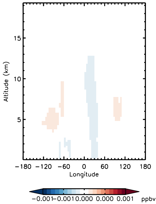
v11-01d-Run0 - v11-01b-Run0 PPN - Diff along 15S for Jan
