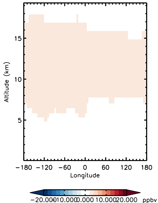
v11-01d-Run0 - v11-01b-Run0 O3 - Diff along 42N for Jan
