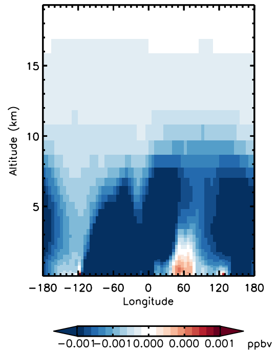
v11-01d-Run0 - v10-01-public-Run0 PPN - Diff along 42N for Jan
