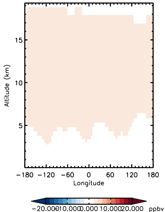
v11-01d-Run0 - v10-01-public-Run0 O3 - Diff along 42N for Jan
