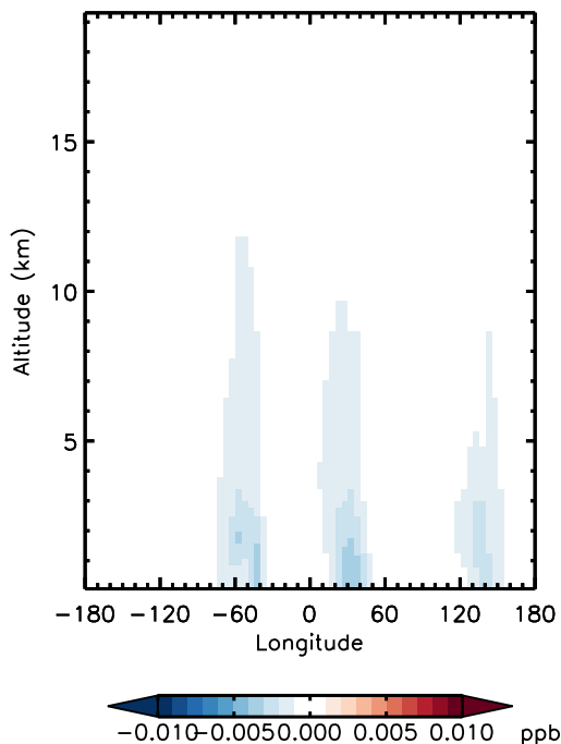
v11-01d-Run0 - v11-01b-Run0 R4N2 - Diff along 15S for Jan
