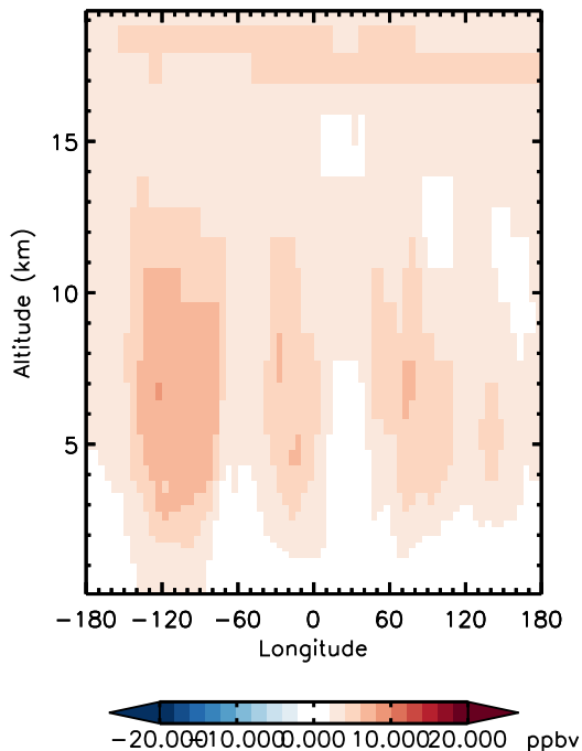
v11-01d-Run0 - v10-01-public-Run0 O3 - Diff along 15S for Jan
