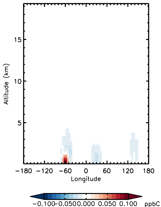
v11-01d-Run0 - v11-01b-Run0 MEK - Diff along 15S for Jan
