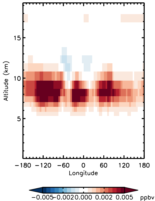
v11-01d-Run0 - v10-01-public-Run0 HNO 4 - Diff along 15S for Jan
