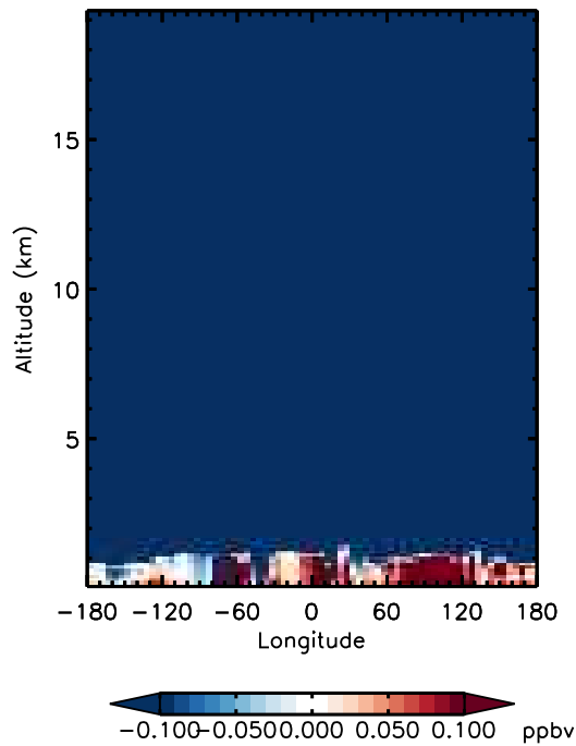
v11-01d-Run0 - v10-01-public-Run0 N2O - Diff along 15S for Jan
