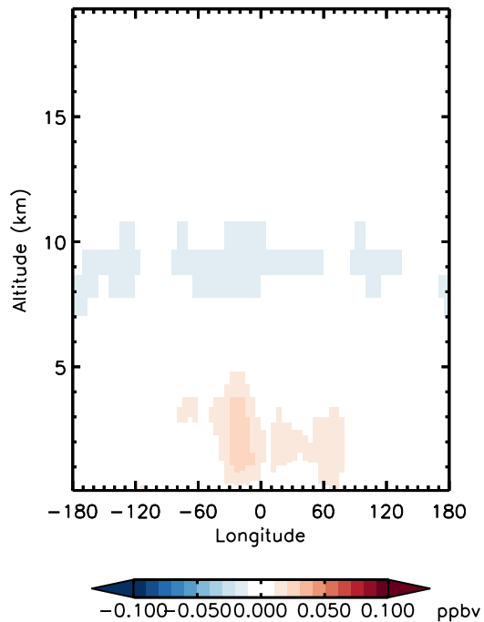
v11-01d-Run0 - v10-01-public-Run0 H2O2 - Diff along 42N for Jan
