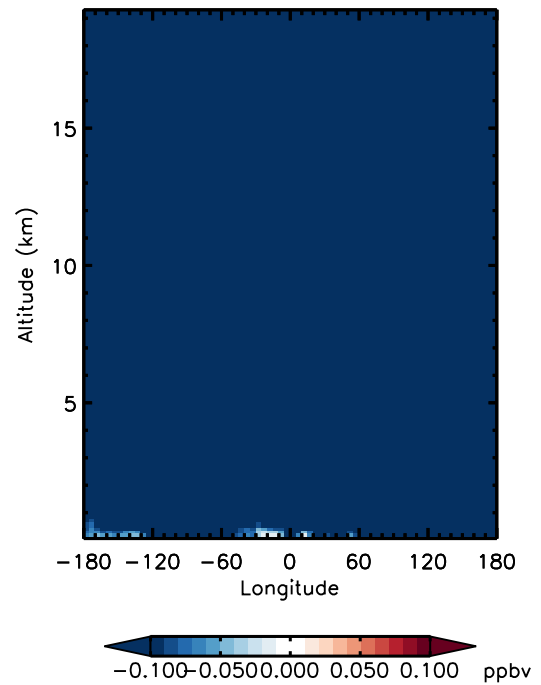
v11-01d-Run0 - v10-01-public-Run0 N2O - Diff along 42N for Jan
