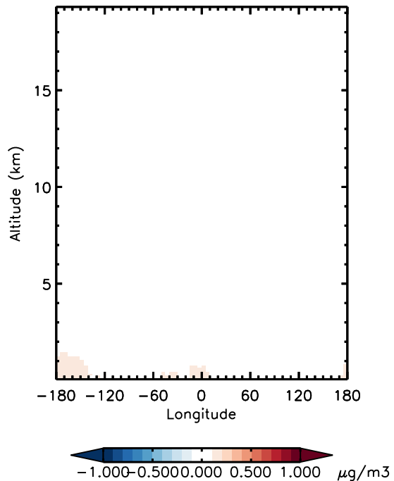
v11-01d-Run0 - v11-01b-Run0 SALA - Diff along 42N for Jan
