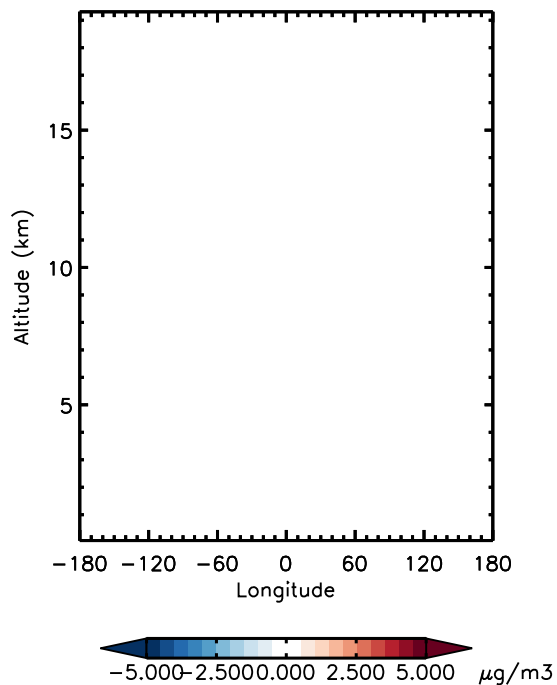
v11-01d-Run0 - v11-01b-Run0 DST4 - Diff along 42N for Jan
