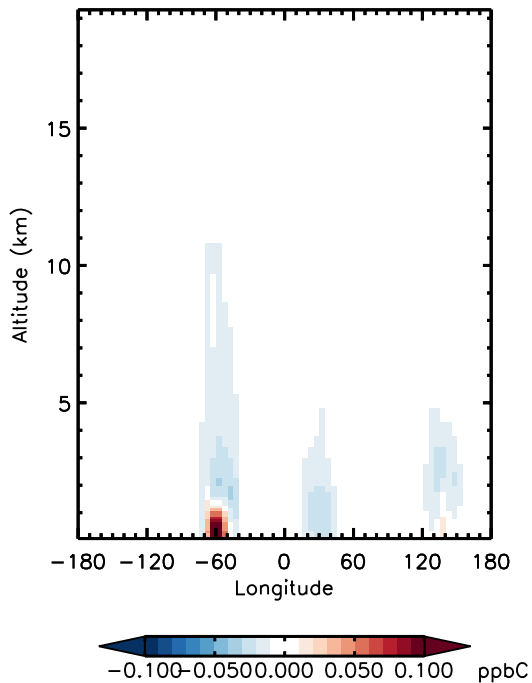
v11-01d-Run0 - v10-01-public-Run0 MEK - Diff along 15S for Jan
