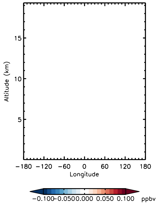
v11-01d-Run0 - v10-01-public-Run0 H1301 - Diff along 15S for Jan
