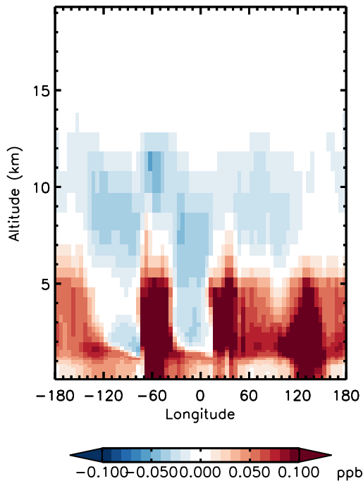
v11-01d-Run0 - v10-01-public-Run0 H2O2 - Diff along 15S for Jan
