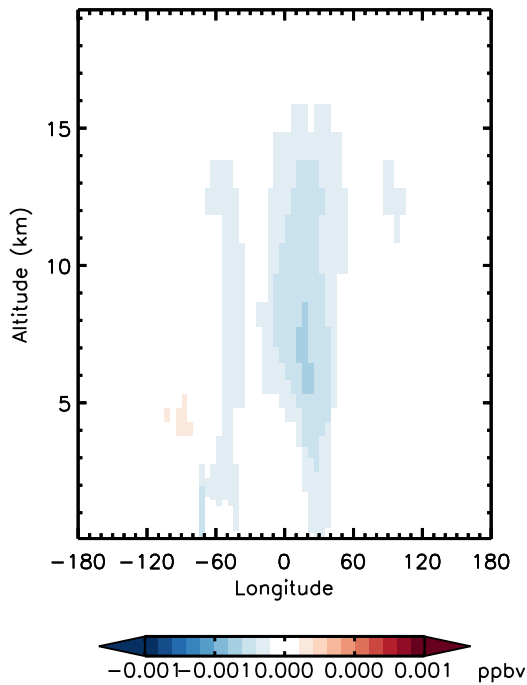
v11-01d-Run0 - v10-01-public-Run0 PPN - Diff along 15S for Jan
