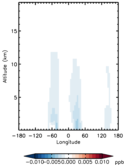
v11-01d-Run0 - v10-01-public-Run0 R4N2 - Diff along 15S for Jan
