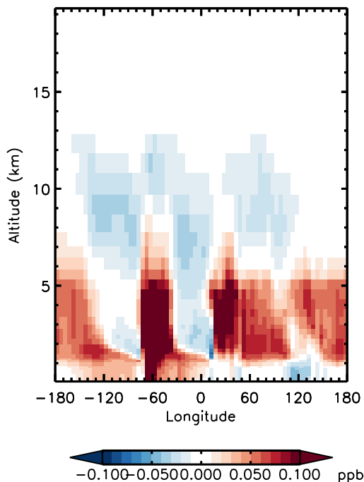
v11-01d-Run0 - v11-01b-Run0 H2O2 - Diff along 15S for Jan
