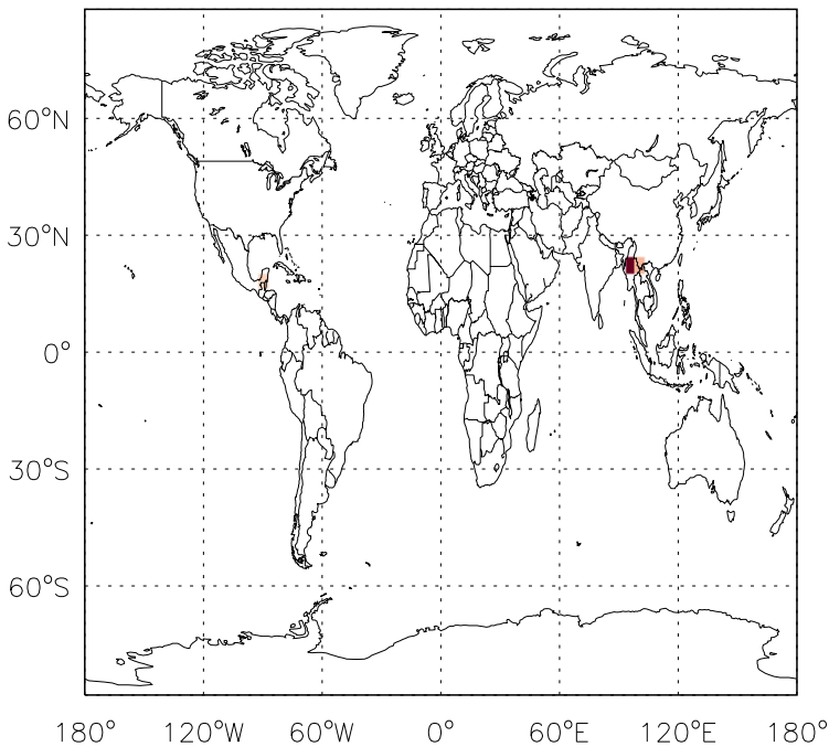
v11-01d-Run1 - v10-01-public-Run0 CH2O biomass emissions for Apr
