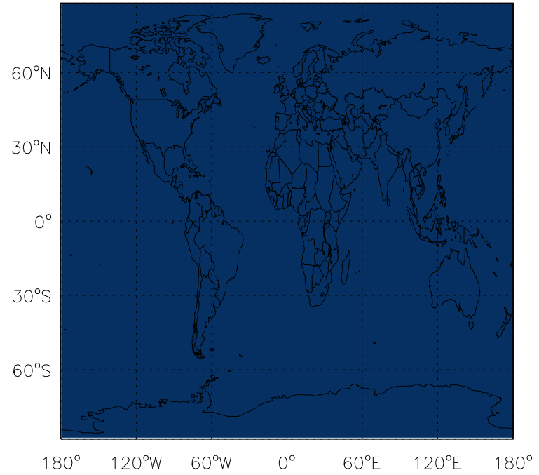
v11-01d-Run1 - v11-01b-Run0 C2H6 anthro+biofuel emissions for Apr
