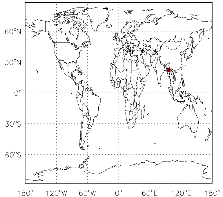
v11-01d-Run1 - v11-01b-Run0 CH2O biomass emissions for Apr
