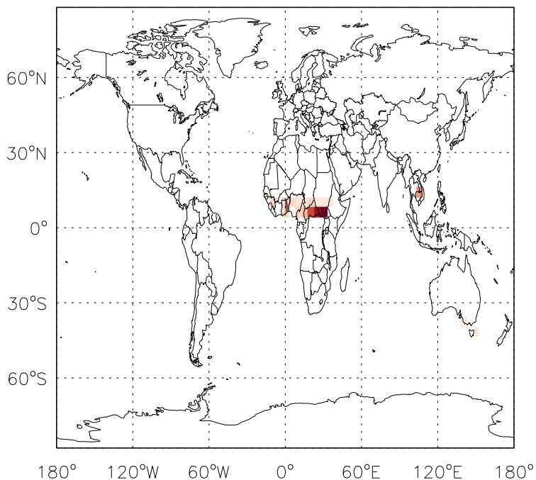
v11-01d-Run1 - v10-01-public-Run0 CH2O biomass emissions for Jan
