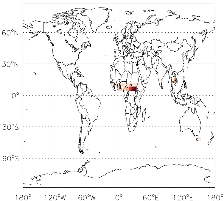
v11-01d-Run1 - v11-01b-Run0 CH2O biomass emissions for Jan
