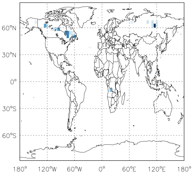
v11-01d-Run1 - v10-01-public-Run0 CH2O biomass emissions for Jul
