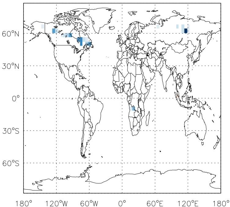
v11-01d-Run1 - v11-01b-Run0 CH2O biomass emissions for Jul
