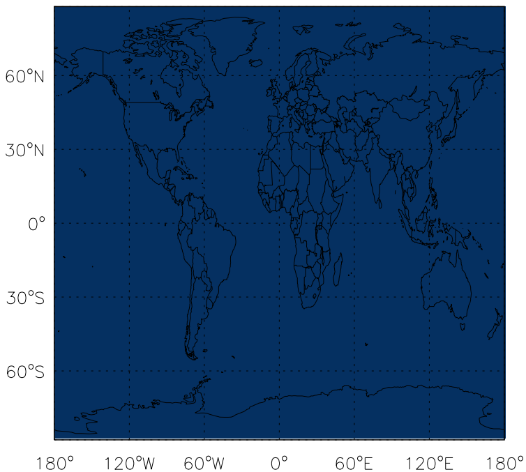
v11-01d-Run1 - v10-01-public-Run0 C2H6 anthro+biofuel emissions for Jul
