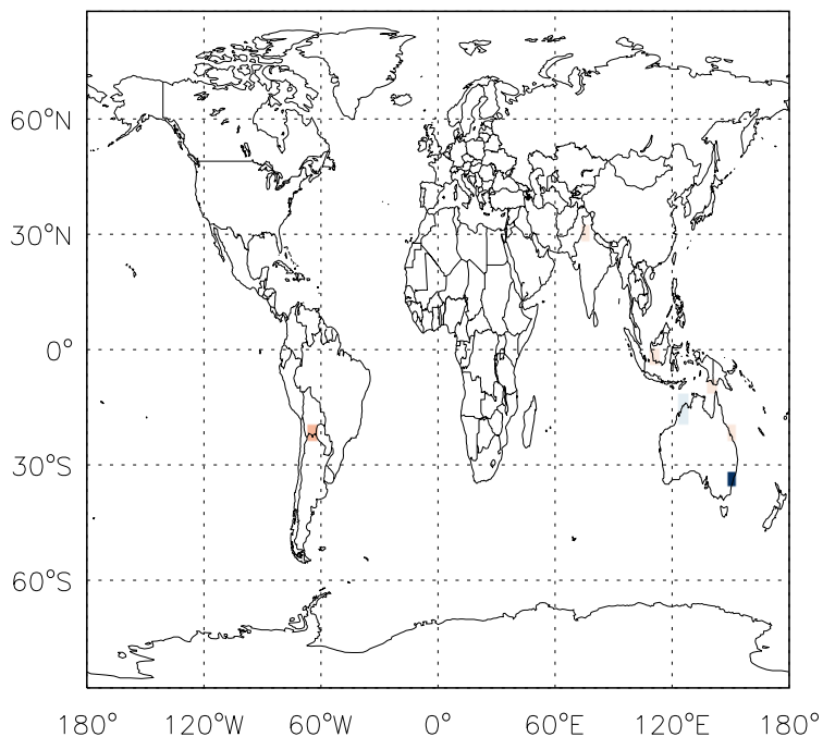
v11-01d-Run1 - v10-01-public-Run0 CH2O biomass emissions for Oct
