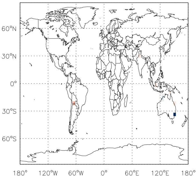
v11-01d-Run1 - v11-01b-Run0 CH2O biomass emissions for Oct
