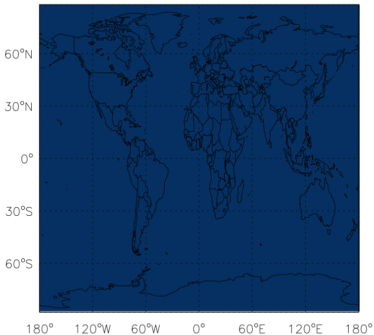
v11-01d-Run1 - v10-01-public-Run0 C2H6 anthro+biofuel emissions for Oct
