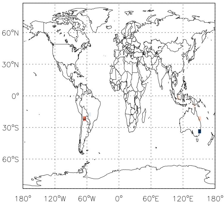
v11-01d-Run1 - v11-01b-Run0 C3H8 biomass emissions for Oct
