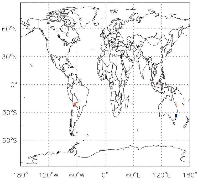
v11-01d-Run1 - v10-01-public-Run0 C3H8 biomass emissions for Oct
