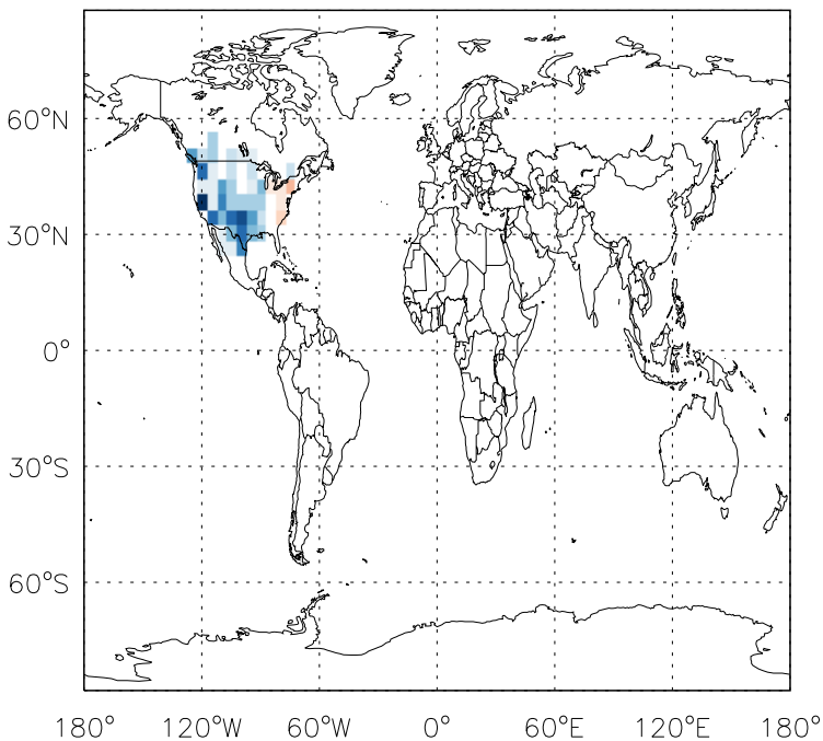
v11-01d-Run1 - v11-01b-Run0 C3H8 anthro+biofuel emissions for Oct
