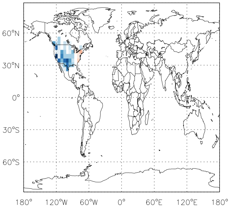
v11-01d-Run1 - v10-01-public-Run0 C3H8 anthro+biofuel emissions for Oct
