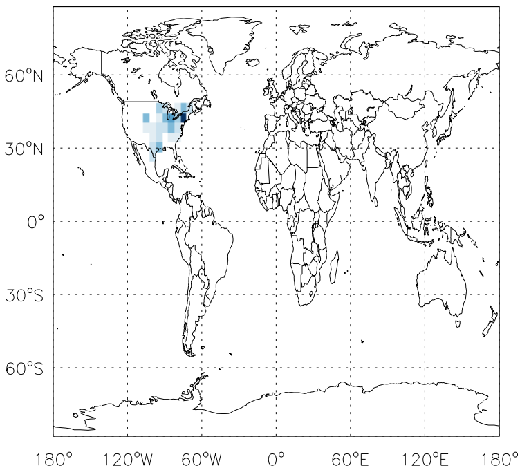
v11-01d-Run1 - v11-01b-Run0 CH 2 O anthro+biofuel emissions for Jan
