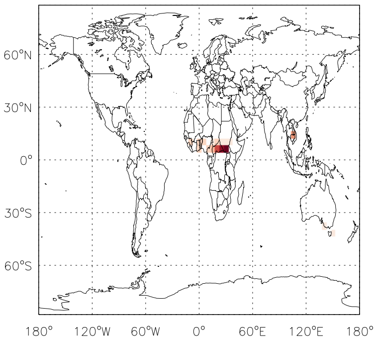
v11-01d-Run1 - v10-01-public-Run0 CH 2 O biomass emissions for Jan
