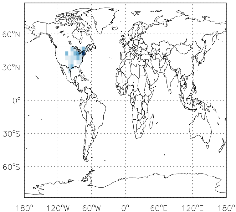
v11-01d-Run1 - v10-01-public-Run0 CH 2 O anthro+biofuel emissions for Jan
