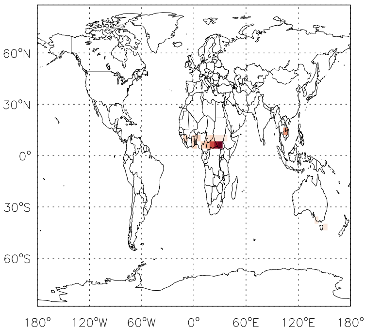
v11-01d-Run1 - v11-01b-Run0 CH 2 O biomass emissions for Jan
