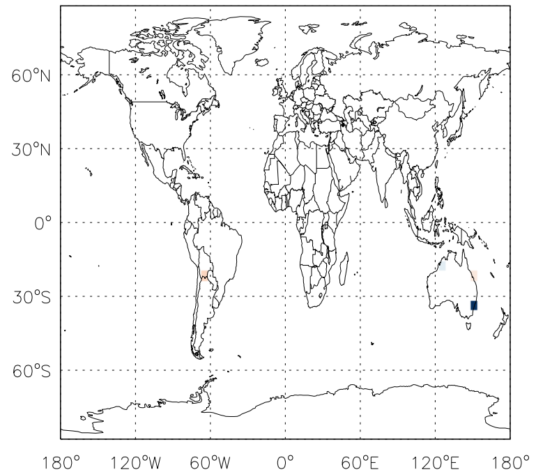
v11-01d-Run1 - v11-01b-Run0 CH 2 O biomass emissions for Oct
