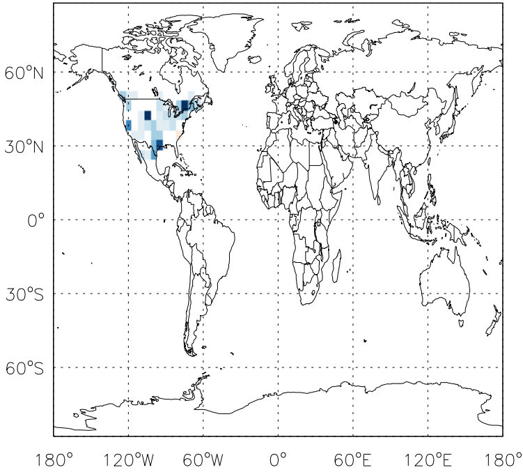
v11-01d-Run1 - v10-01-public-Run0 CH 2 O anthro+biofuel emissions for Oct
