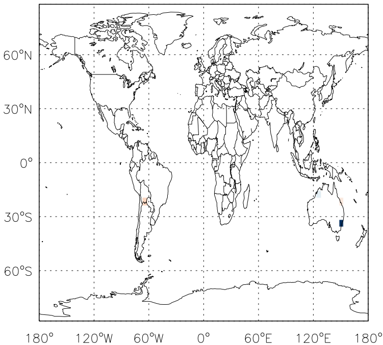
v11-01d-Run1 - v10-01-public-Run0 CH 2 O biomass emissions for Oct
