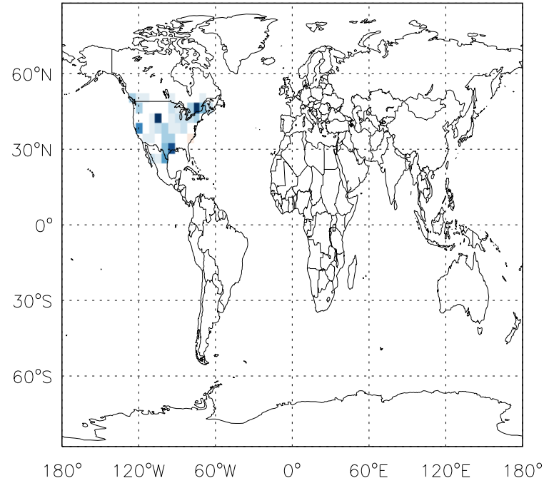
v11-01d-Run1 - v11-01b-Run0 CH 2 O anthro+biofuel emissions for Oct
