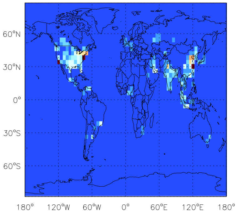
ALK4 anthro+biofuel emissions for Jul
