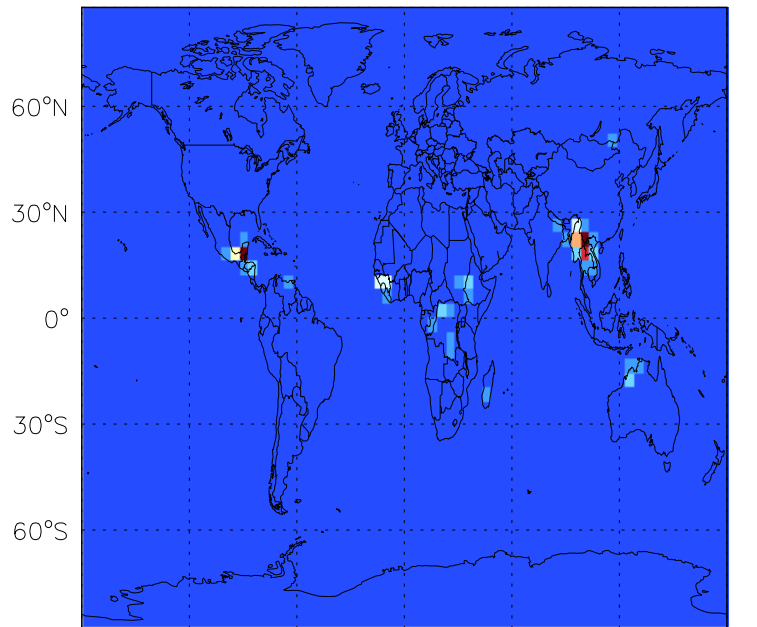
BC biomass emissions for Apr
