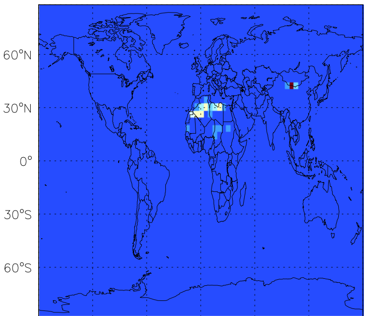
DST4 emissions for Apr
