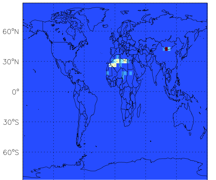
DST4 emissions for Apr
