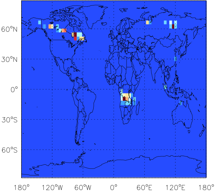
MEK biomass emissions for Jul
