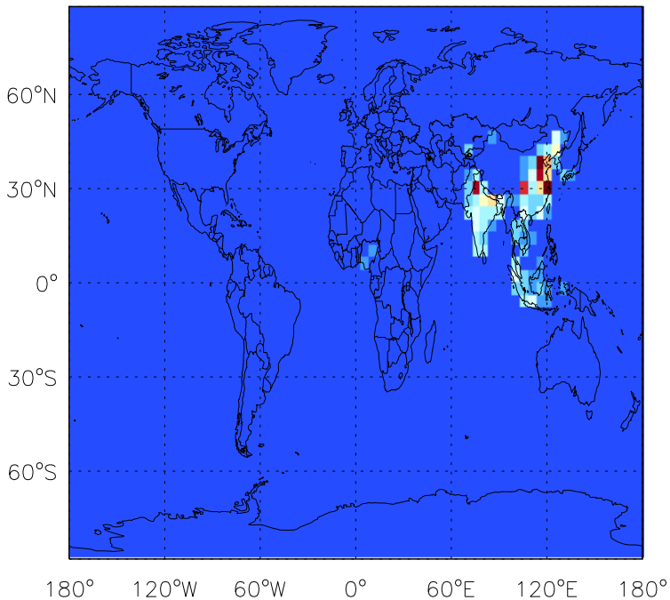
PRPE anthro+biofuel emissions for Jan
