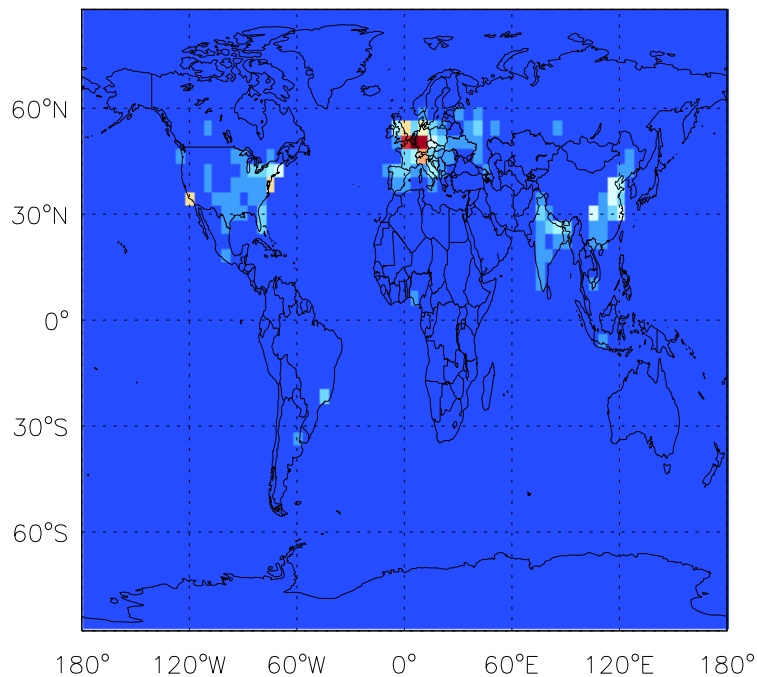
ACET anthro+biofuel emissions for Jan
