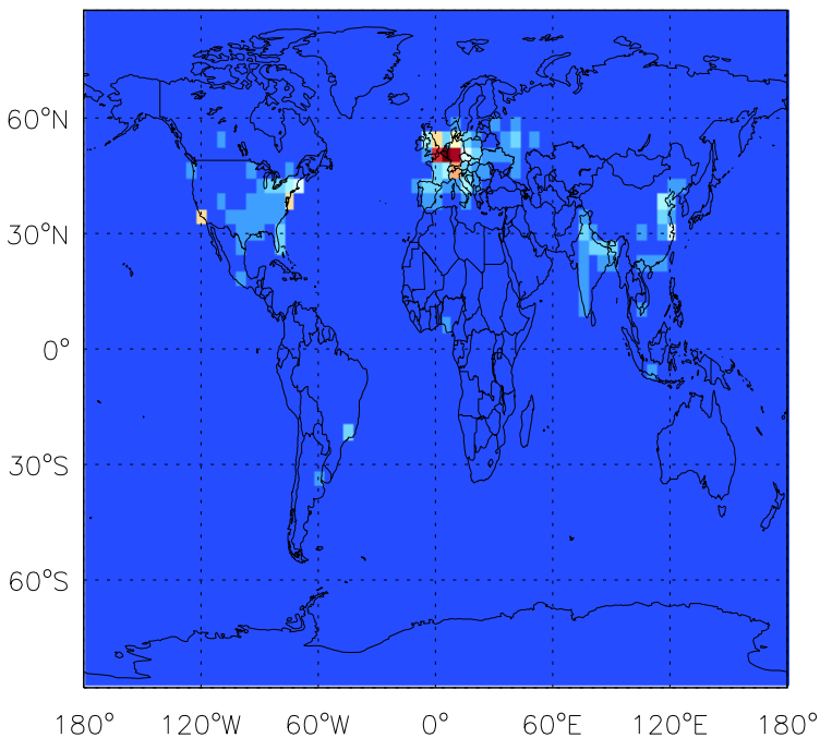
ACET anthro+biofuel emissions for Jul
