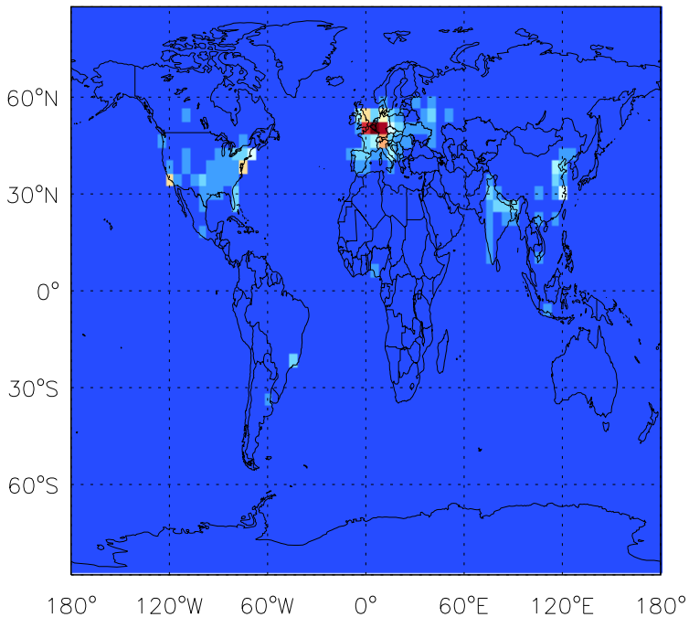
ACET anthro+biofuel emissions for Oct
