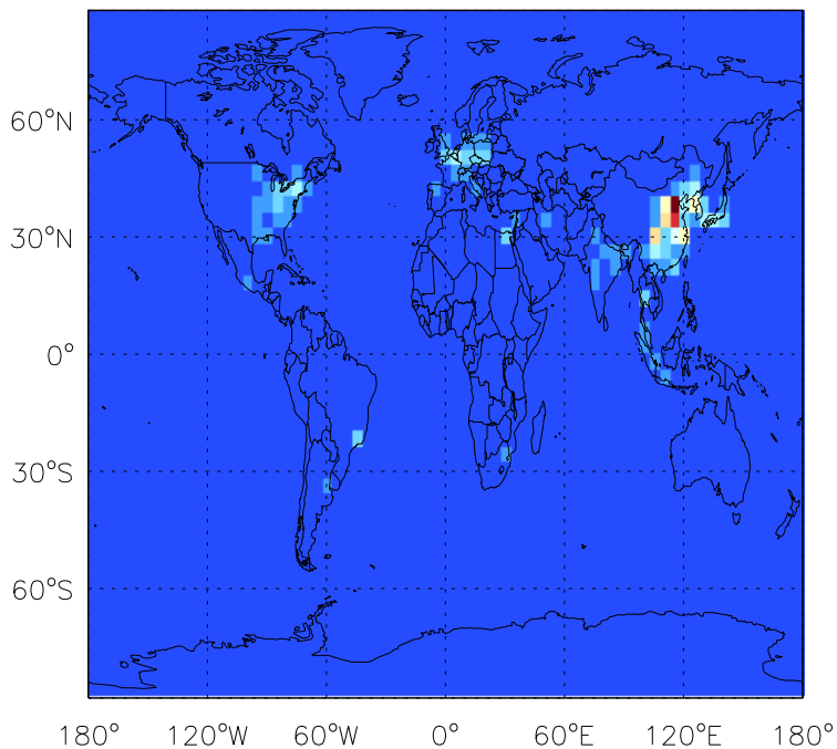
BC anthro emissions for Jan
