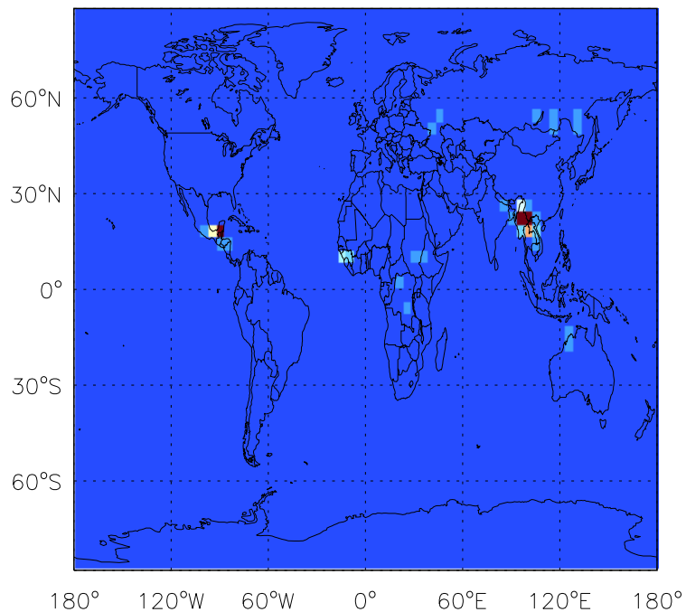
CH 2 O biomass emissions for Apr
