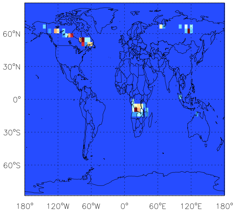
CO biomass emissions for Jul
