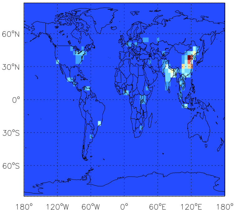
CO anthro+biofuel emissions for Oct
