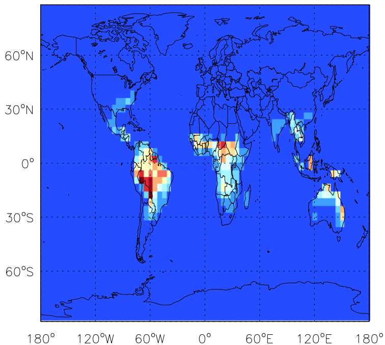
ISOP biogenic emissions for Oct
