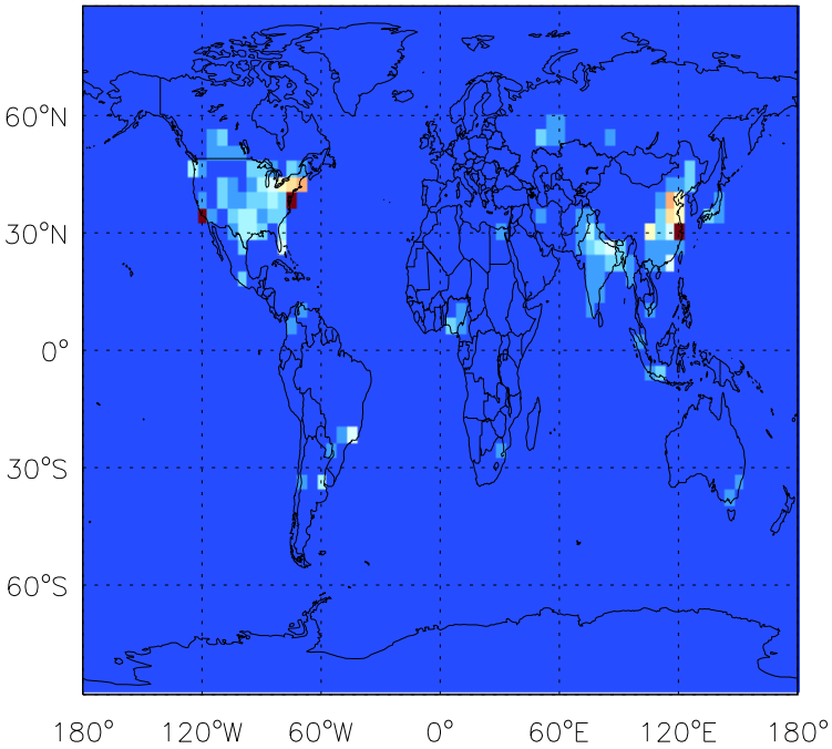
MEK anthro+biofuel emissions for Jan
