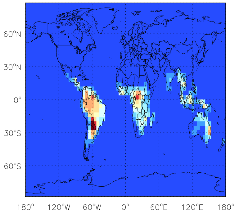
PRPE biogenic emissions for Jan
