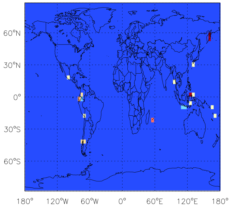
SO 2 column volcanic emissions for Jan
