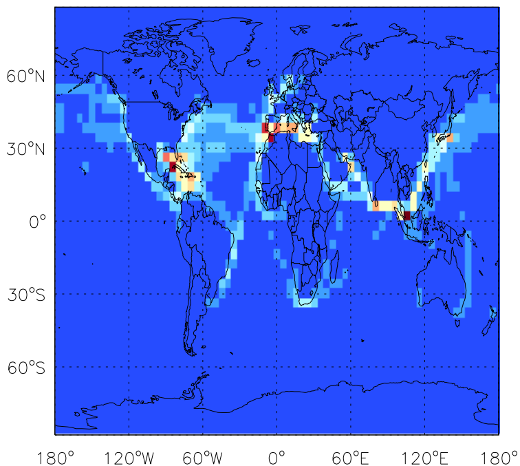
S02 ship emissions for Oct
