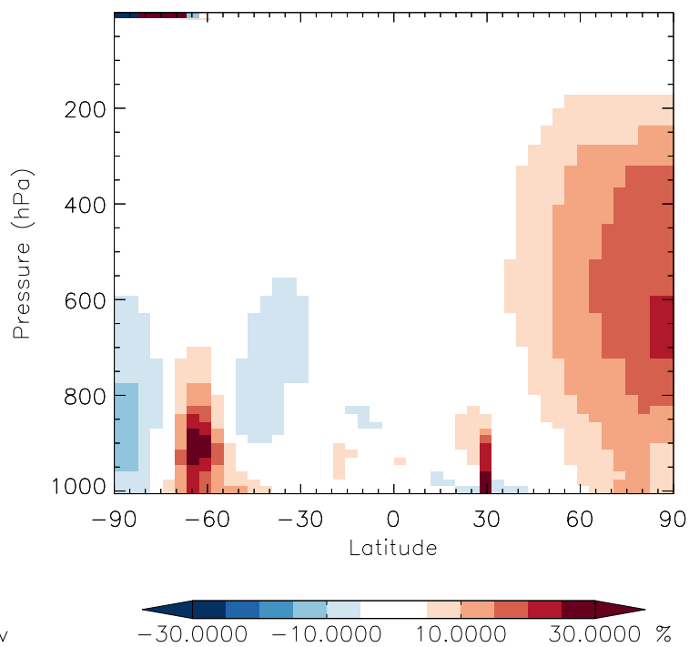
v11-01f-geosfp-Run0 / v11-01d-Run1 N2O5 - Zonal mean % diff for Jan
