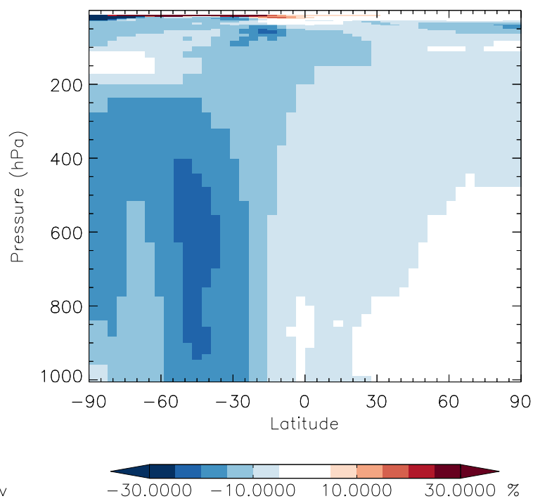
v11-01f-geosfp-Run0 / v11-01b-Run0 PROPNN - Zonal mean % diff for Jan
