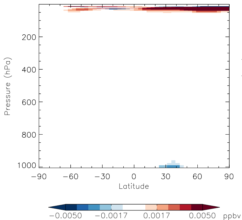
v11-01f-geosfp-Run0 - v11-01d-Run1 N2O5 - Zonal mean abs diff for Jan
