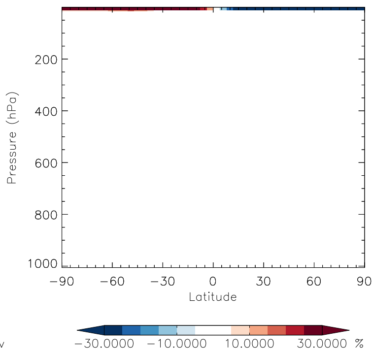
v11-01f-geosfp-Run0 / v11-01b-Run0 CH 3 CCl 3 - Zonal mean % diff for Jan
