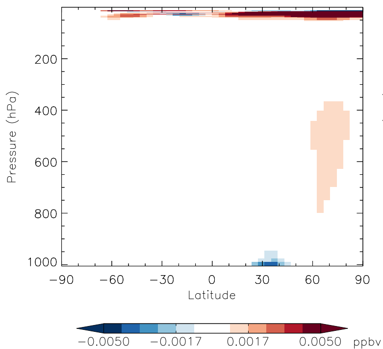
v11-01f-geosfp-Run0 - v11-01b-Run0 N2O5 - Zonal mean abs diff for Jan
