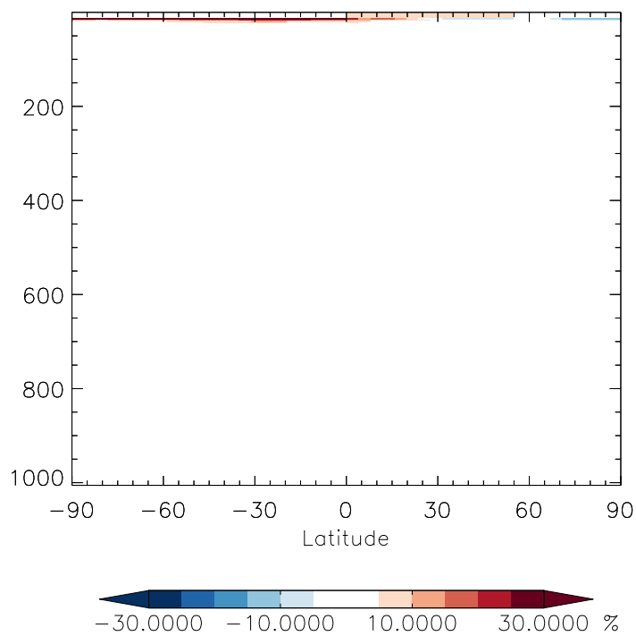
v11-01f-geosfp-Run0 / v11-01d-Run1 CH 2 Br 2 - Zonal mean % diff for Jan
