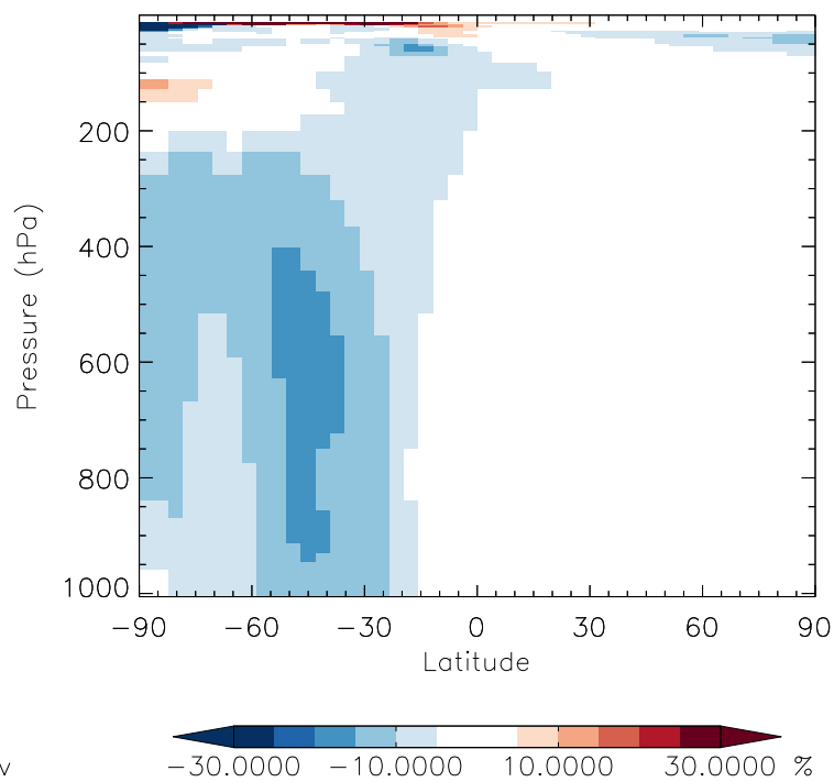
v11-01f-geosfp-Run0 / v11-01d-Run1 PROPNN - Zonal mean % diff for Jan
