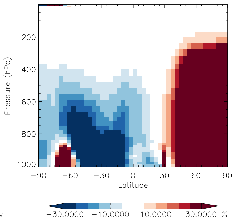
v11-01f-geosfp-Run0 / v11-01b-Run0 N2O5 - Zonal mean % diff for Jan
