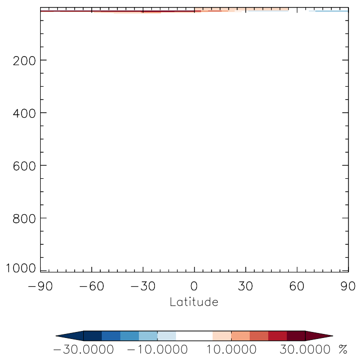
v11-01f-geosfp-Run0 / v11-01b-Run0 CH 2 Br 2 - Zonal mean % diff for Jan
