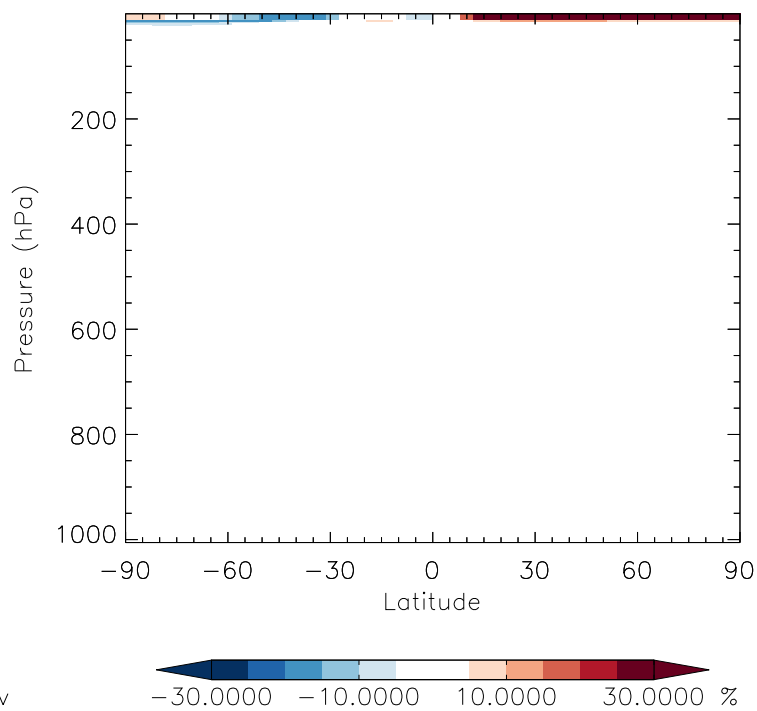
v11-01f-geosfp-Run0 / v11-01d-Run1 CH 3 CCl 3 - Zonal mean % diff for Jul
