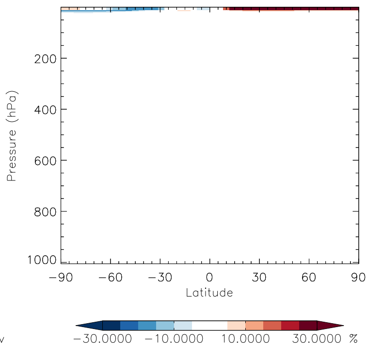
v11-01f-geosfp-Run0 / v11-01b-Run0 CH 3 CCl 3 - Zonal mean % diff for Jul
