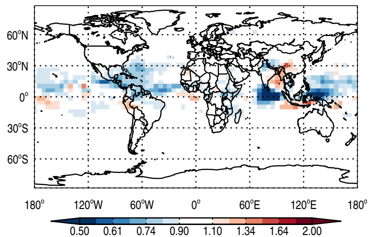
Ratio @ 500 hPa for Be7
