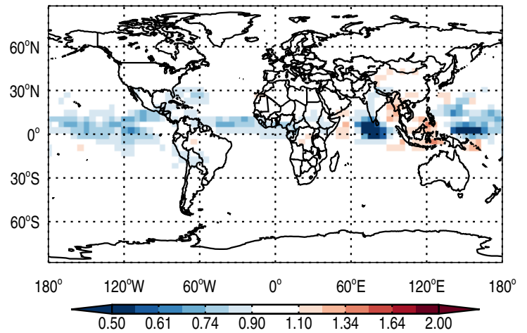
Ratio @ 500 hPa for Pb
