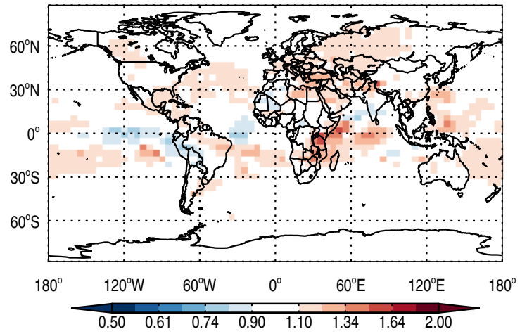
Ratio @ 500 hPa for Rn
