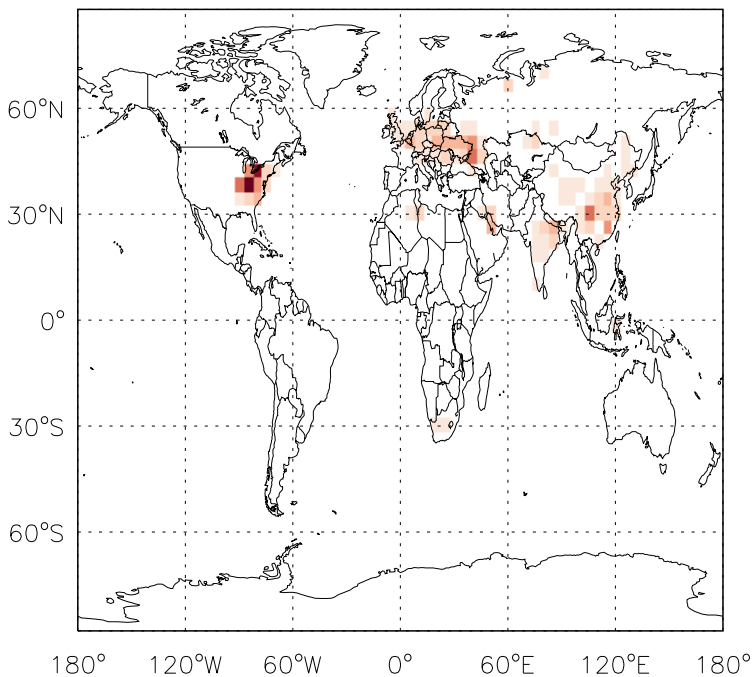
v11-01f-merra2-Run0 - v11-01d-Run1 C2H6 anthro+biofuel emissions for Jul
