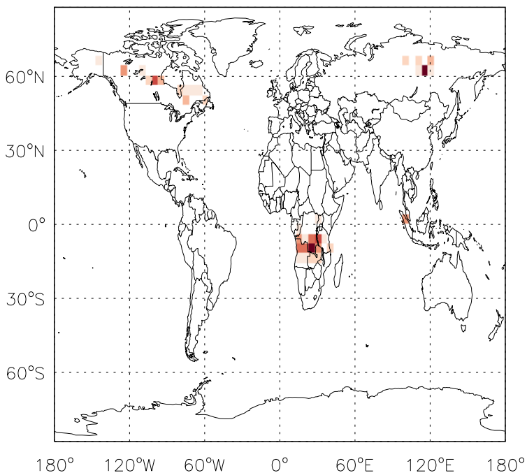
v11-01f-merra2-Run0 - v11-01d-Run1 CH2O biomass emissions for Jul
