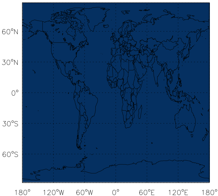
v11-01f-merra2-Run0 - v11-01f-geosp-Run0 C2H6 anthro+biofuel emissions for Oct
