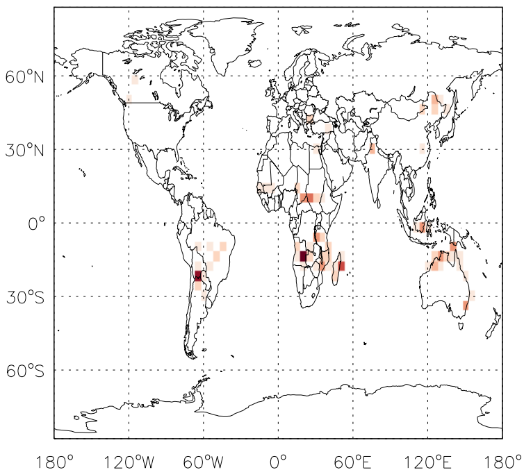
v11-01f-merra2-Run0 - v11-01d-Run1 CH2O biomass emissions for Oct
