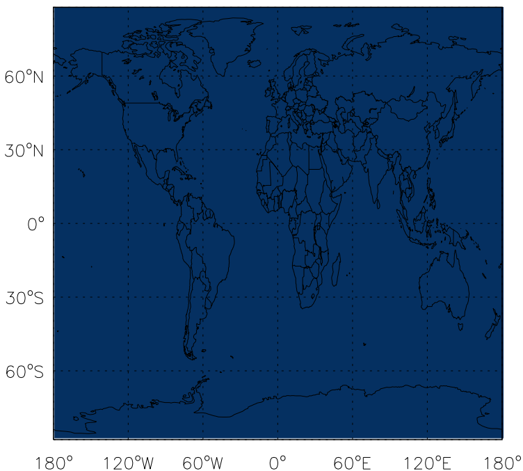
v11-01f-merra2-Run0 - v11-01f-geosp-Run0 CH2O biomass emissions for Oct
