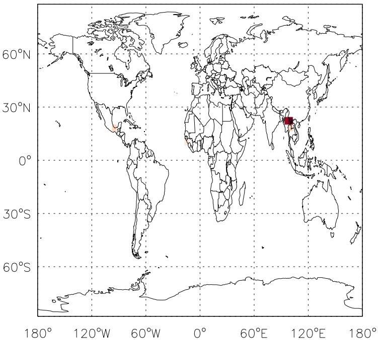
v11-01f-merra2-Run0 - v11-01d-Run1 C3H8 biomass emissions for Apr
