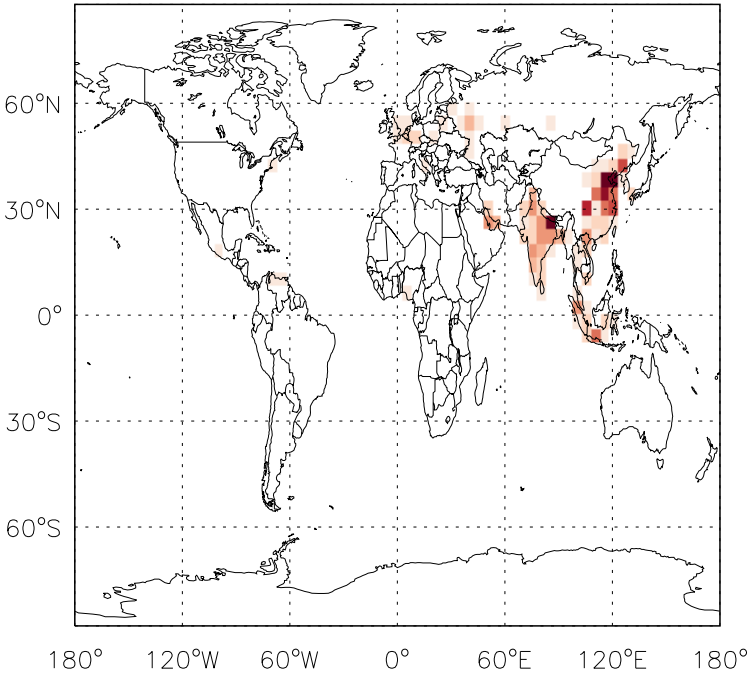
v11-01f-merra2-Run0 - v11-01d-Run1 C3H8 anthro+biofuel emissions for Apr
