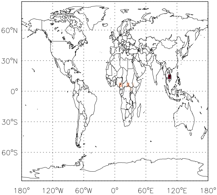
v11-01f-merra2-Run0 - v11-01d-Run1 C3H8 biomass emissions for Jan
