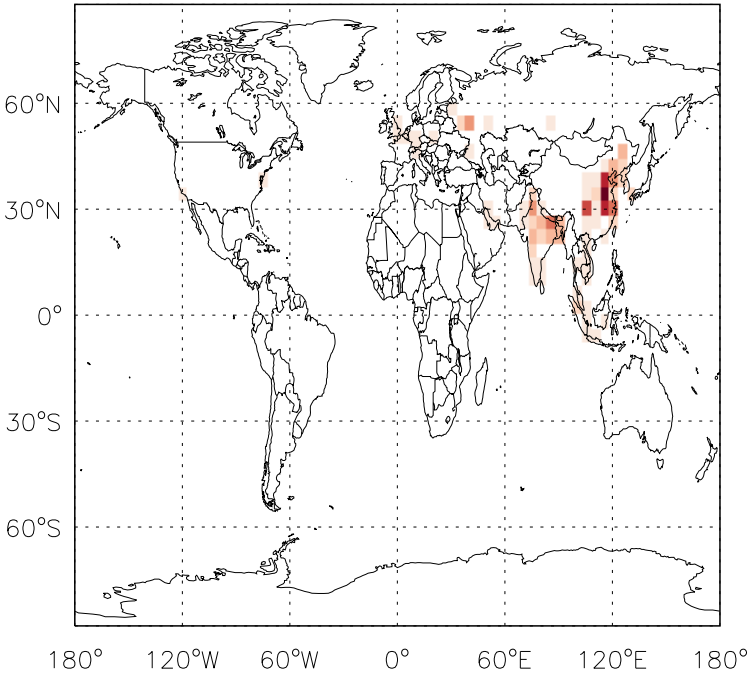
v11-01f-merra2-Run0 - v11-01d-Run1 C3H8 anthro+biofuel emissions for Jan
