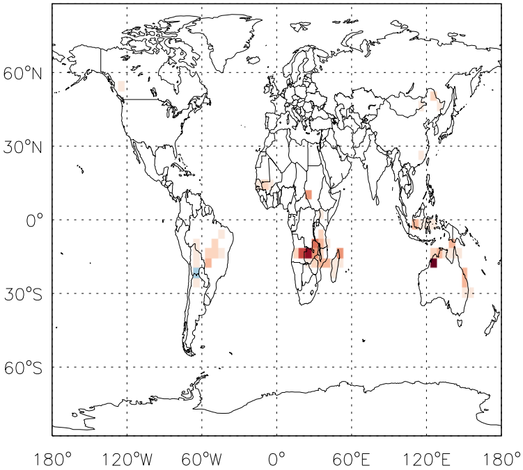
v11-01f-merra2-Run0 - v11-01d-Run1 C3H8 biomass emissions for Oct
