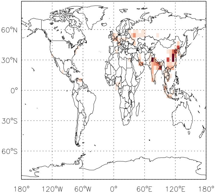
v11-01f-merra2-Run0 - v11-01d-Run1 C3H8 anthro+biofuel emissions for Oct
