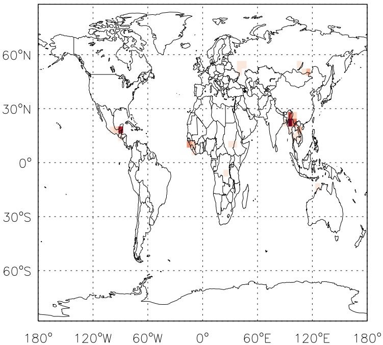
v11-01f-merra2-Run0 - v11-01d-Run1 CH 2 O biomass emissions for Apr
