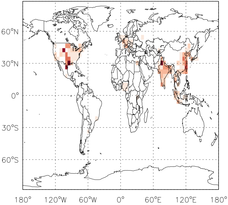
v11-01f-merra2-Run0 - v11-01d-Run1 CH 2 O anthro+biofuel emissions for Apr
